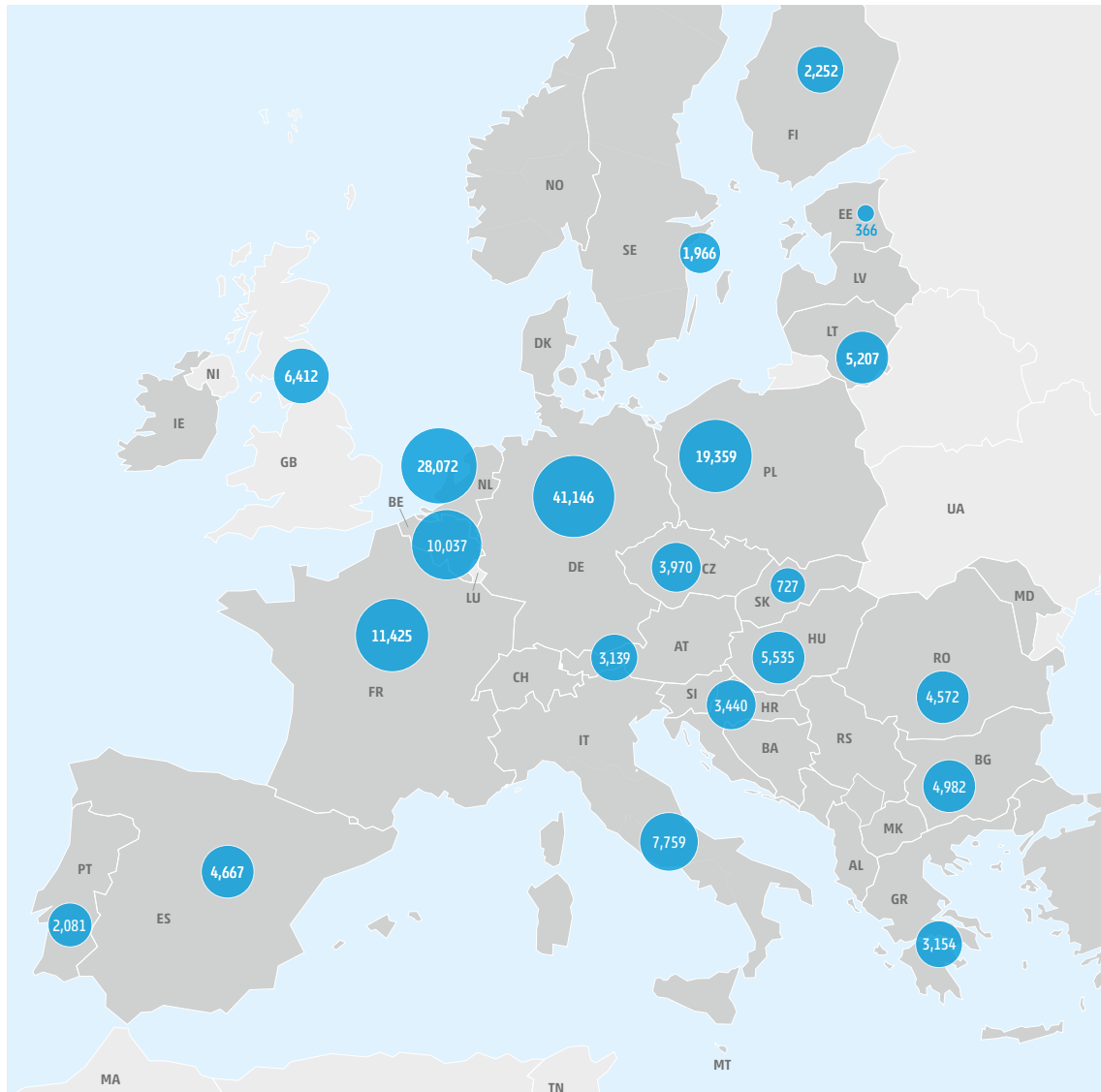
Figure 36: Distribution of hydrogen production from natural gas in the advanced infrastructure level in 2040 for stressful weather year (unit: GWh/y).
