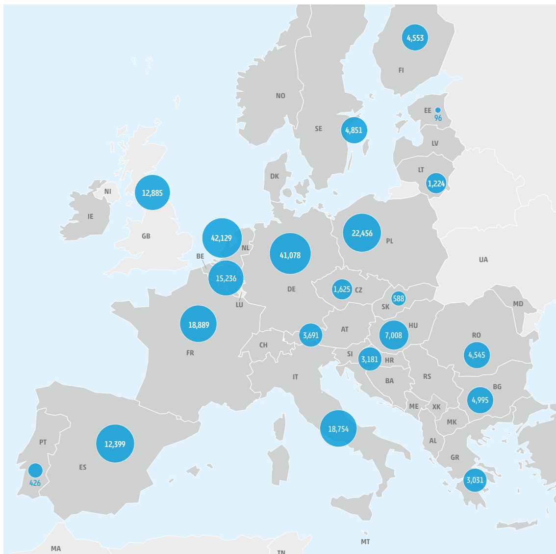
Figure 13: Distribution of hydrogen production from natural gas in the advanced infrastructure level in 2030 for reference weather year (unit: GWh/y).
