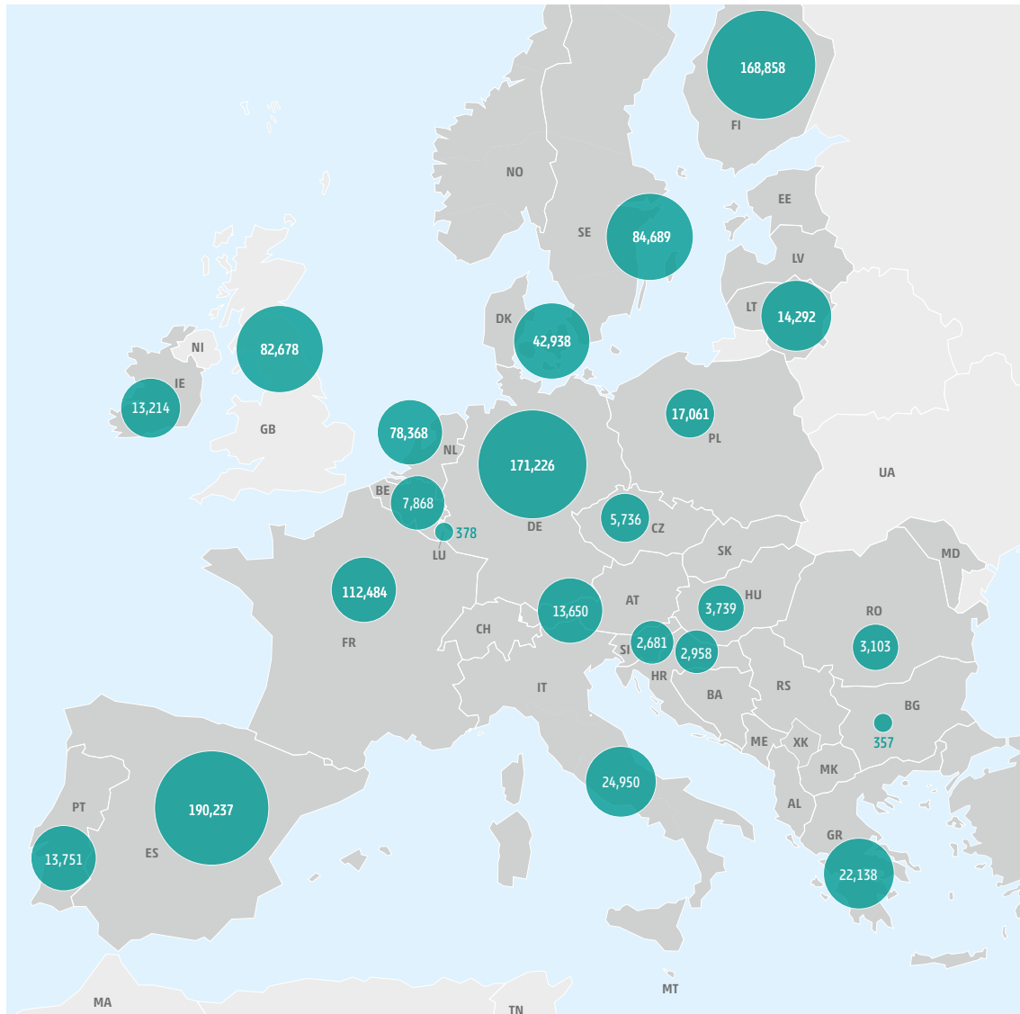
Figure 23: Distribution of electrolytic hydrogen production per country in the PCI/PMI hydrogen infrastructure level in 2040 for reference weather year (unit: GWh/y).
