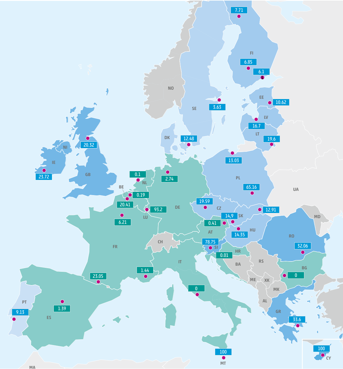
Figure 20: Yearly average hydrogen demand curtailment rate at country or node level in the advanced infrastructure level in 2030 for stressful weather year (unit: %).
