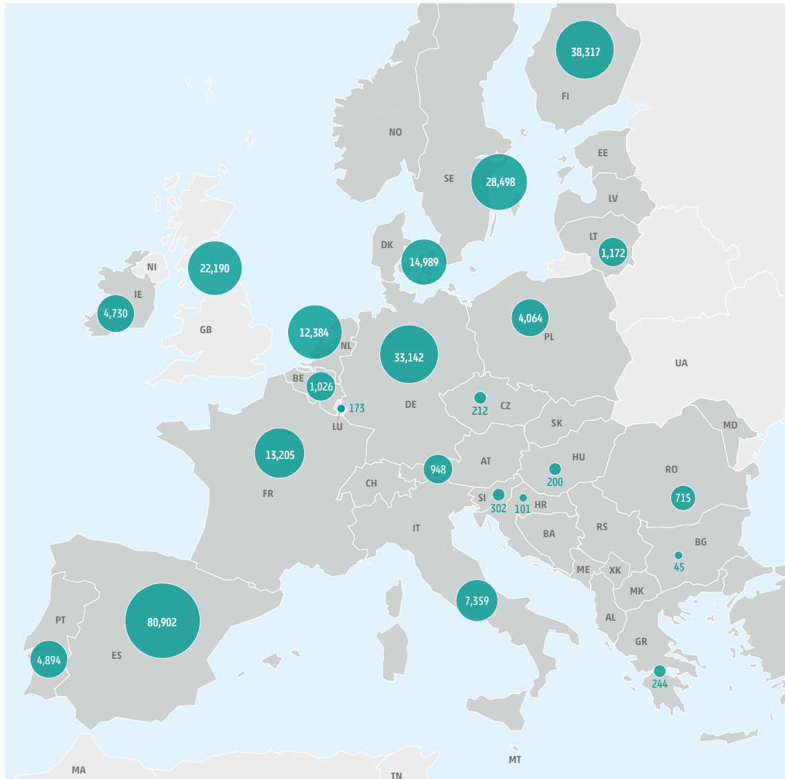
Figure 6: Distribution of hydrogen production via electrolysis in the PCI/PMI hydrogen infrastructure level in 2030 for stressful weather year (unit: GWh/y).
