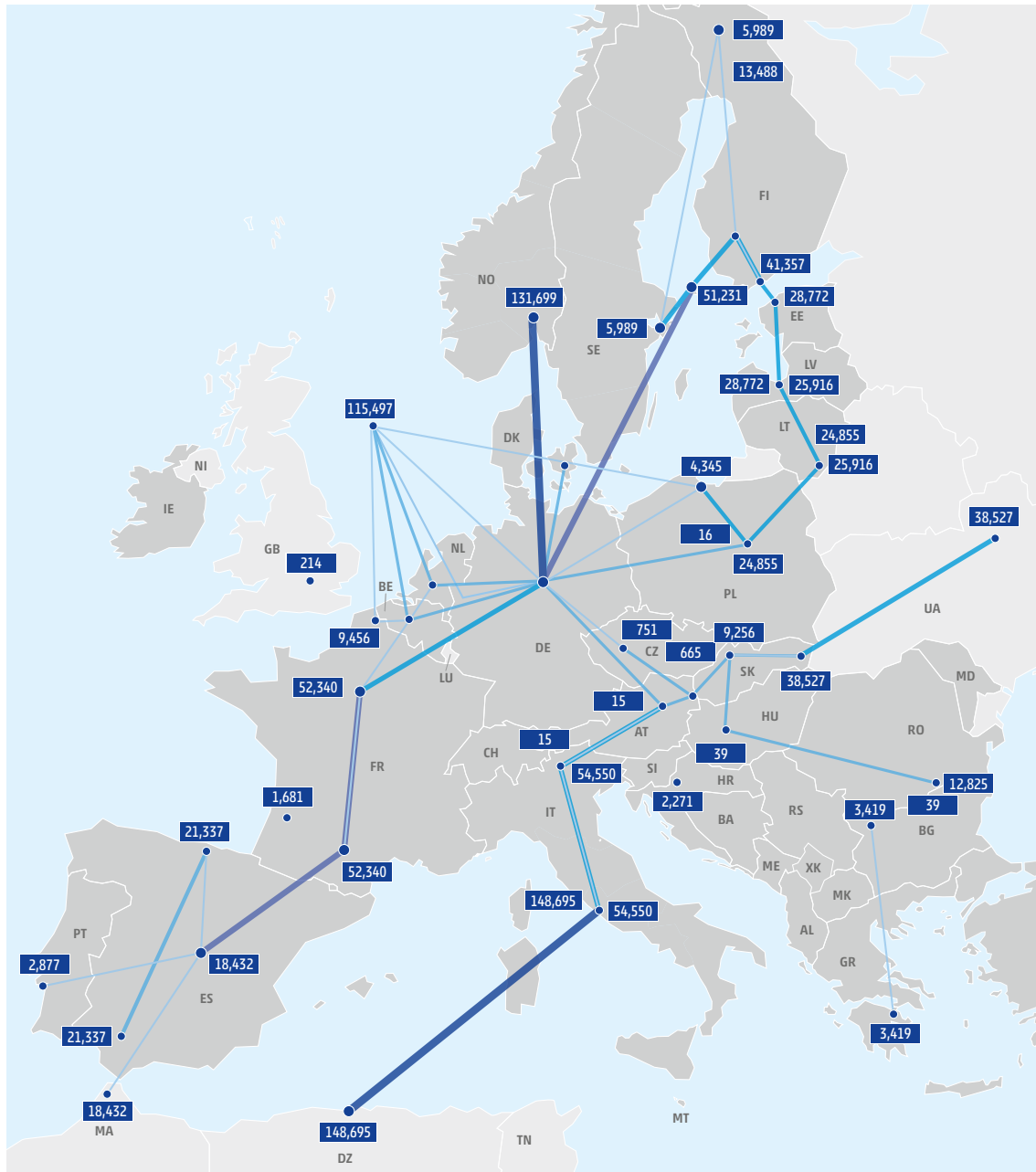
Figure 37: Grid flows* in the Advanced hydrogen infrastructure level in 2040 for stressful weather year (unit: GWh/y).
