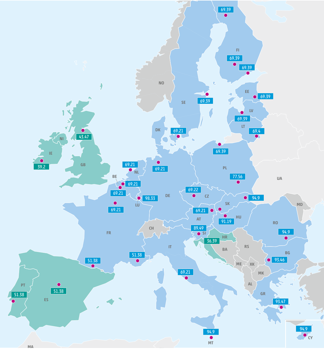
Figure 9: Average of the hourly hydrogen market clearing prices per country in the PCI/PMI hydrogen infrastructure level in 2030 (unit: €/MWh).
