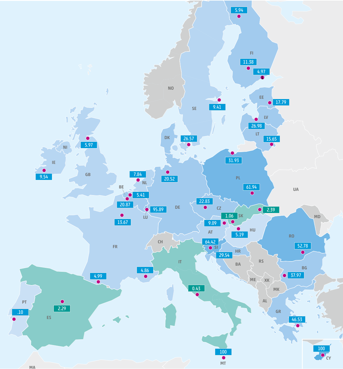
Figure 40: Yearly average hydrogen demand curtailment rate at country or node level in the Advanced hydrogen infrastructure level in 2040 for stressful weather year (unit: %).
