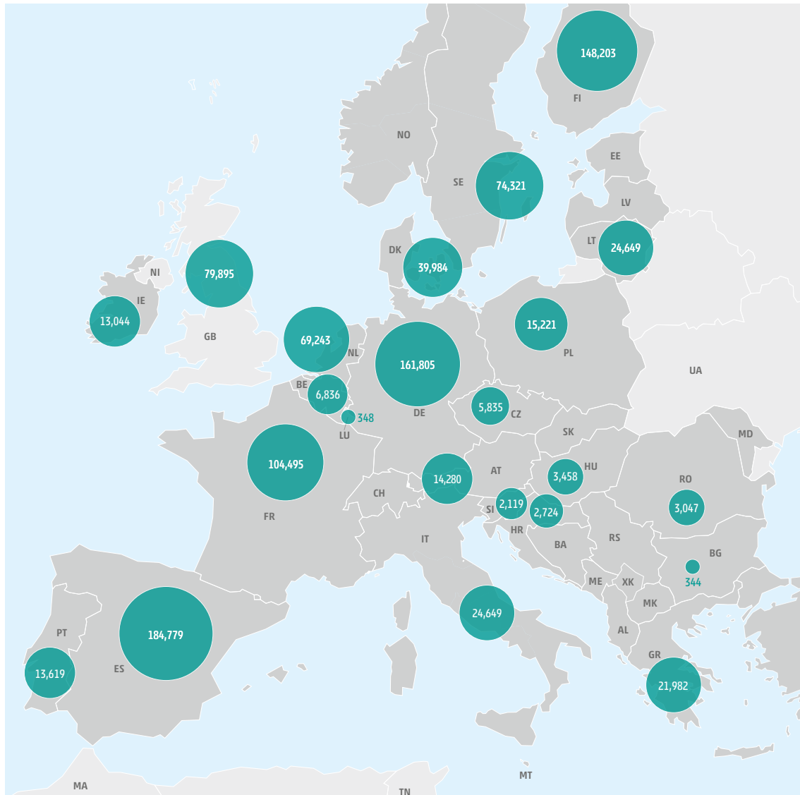
Figure 35: Distribution of electrolytic hydrogen production from natural gas in the Advanced hydrogen infrastructure level in 2040 for stressful weather year (unit: GWh/y).
