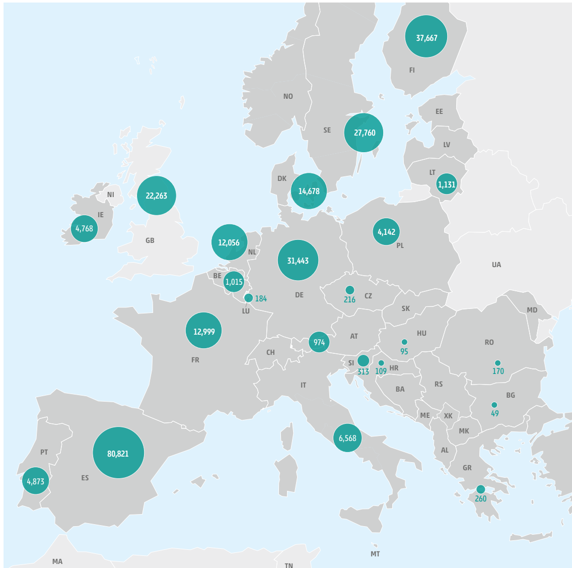
Figure 15: Distribution of hydrogen production via electrolysis in the advanced infrastructure level in 2030 for stressful weather year (unit: GWh/y).
