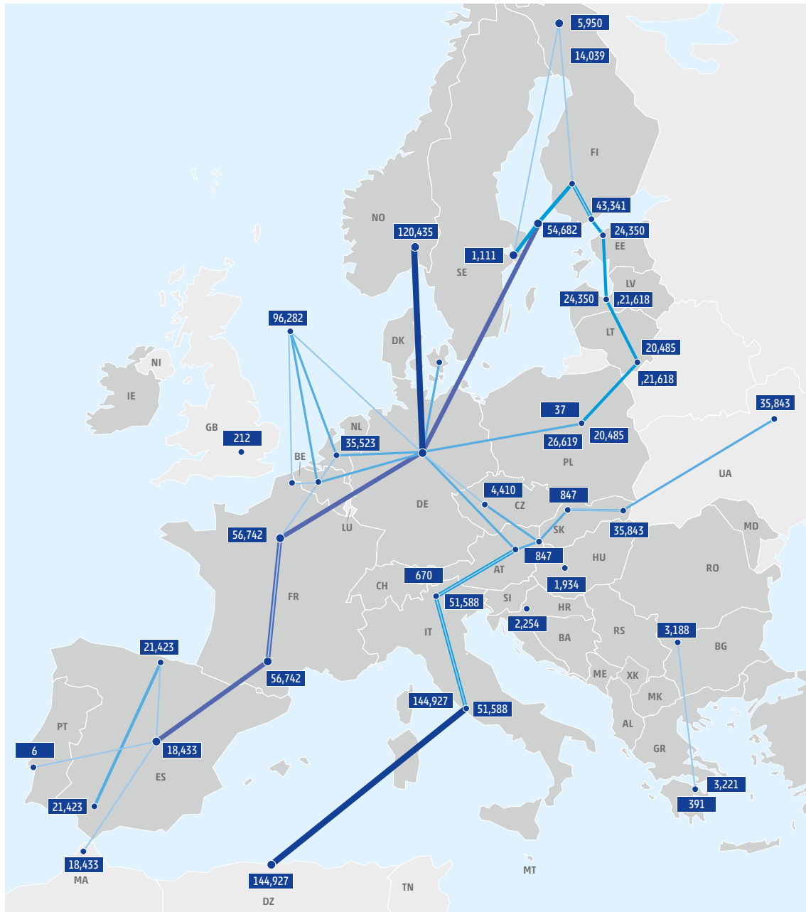
Figure 28: Grid flows* in the PCI/PMI hydrogen infrastructure level in 2040 for stressful weather year (unit: GWh/y).
