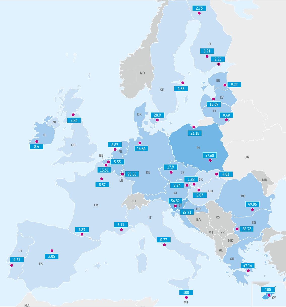
Figure 39: Yearly average hydrogen demand curtailment rate at country or node level in the advanced hydrogen infrastructure level in 2040 for reference year (unit: %).
