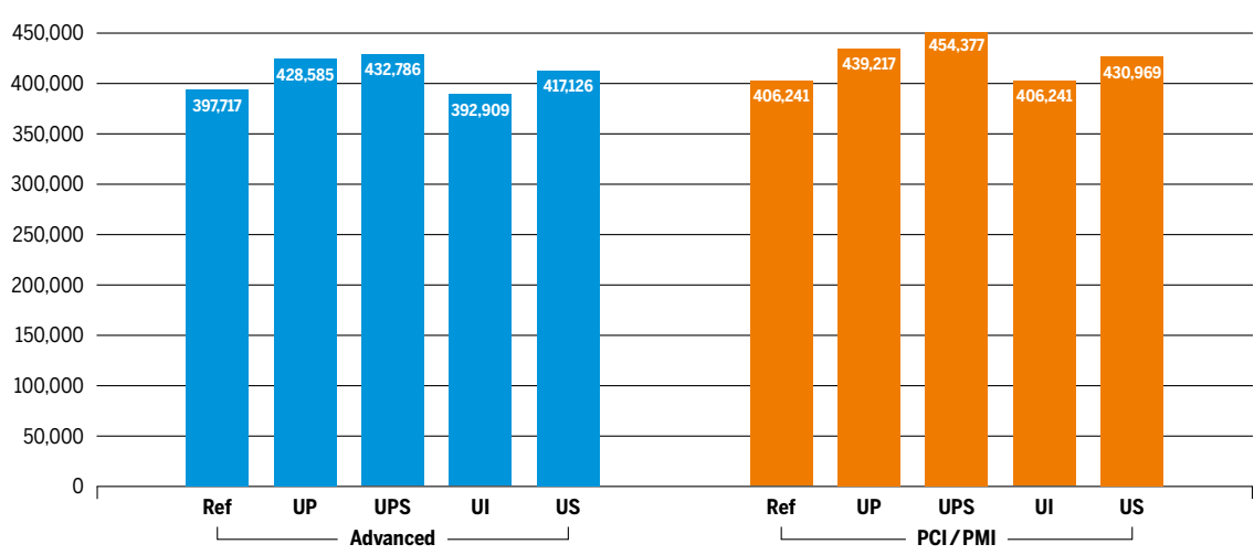
Figure 22: Electrolyser production Advanced level 2030 and PCI level 2030 (unit: GWh/y).
