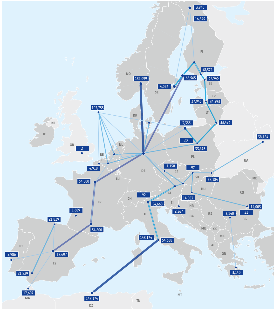
Figure 34: Grid flows* in the Advanced hydrogen infrastructure level in 2040 for reference weather year (unit: GWh/y).
