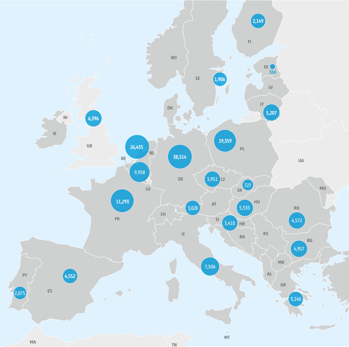
Figure 27: Distribution of hydrogen production from natural gas in the PCI/PMI hydrogen infrastructure level in 2040 for stressful weather year (unit: GWh/y).
