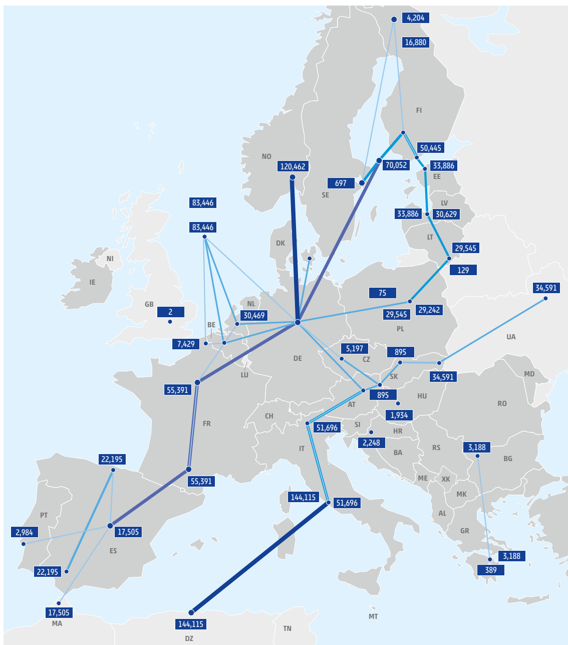
Figure 25: Grid flows* in the PCI/PMI hydrogen infrastructure level in 2040 for reference weather year (unit: GWh/y).
