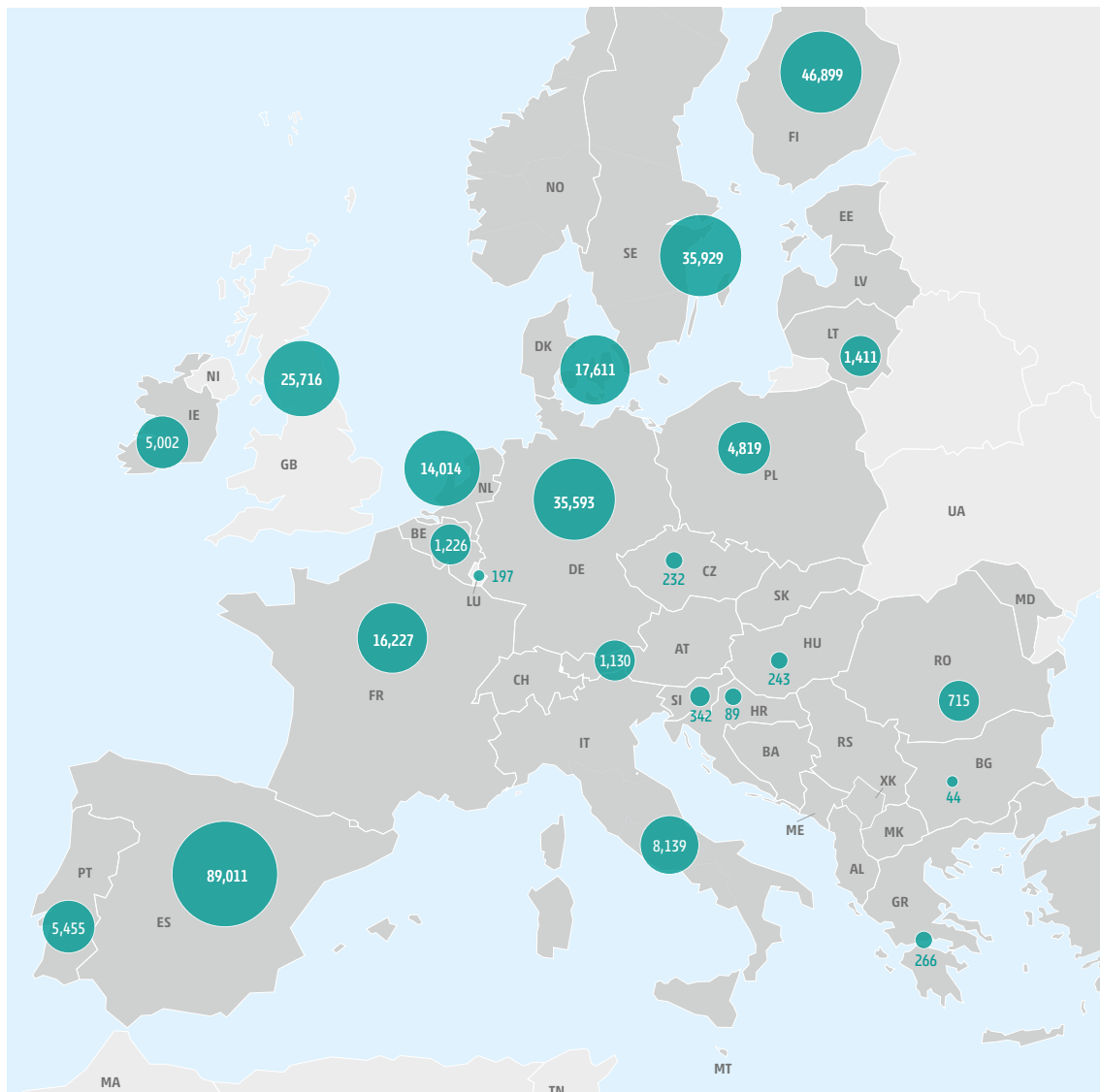
Figure 3: Distribution of hydrogen production via electrolysis in the PCI/PMI hydrogen infrastructure level in 2030 for reference weather year (unit: GWh/y).
