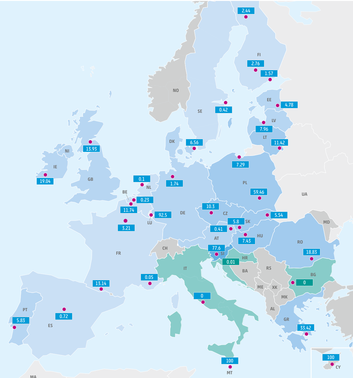
Figure 19: Yearly average hydrogen demand curtailment rate at country or node level in the advanced infrastructure level in 2030 for reference year (unit: %).
