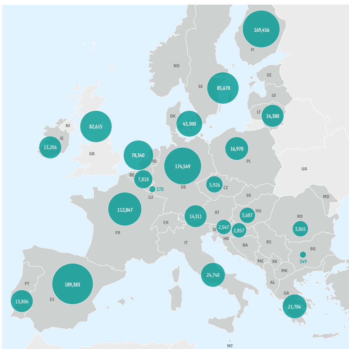
Figure 32: Distribution of electrolytic hydrogen production in the Advanced hydrogen infrastructure level in 2040 for reference weather year (unit: GWh/y).
