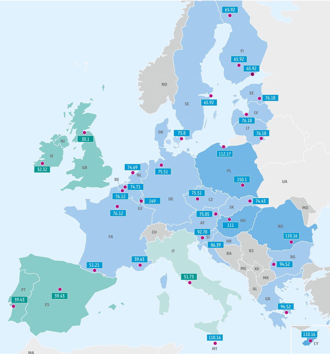
Figure 29: Average of the hourly hydrogen market clearing prices per country in the PCI/PMI hydrogen infrastructure level in 2040 (unit: €/MWh).
