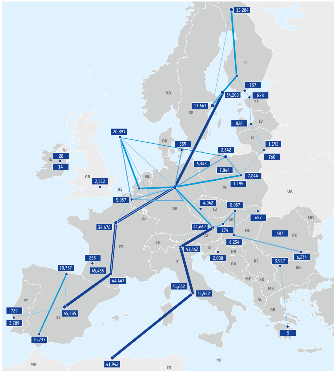
Figure 14: Grid flows* in the advanced infrastructure level in 2030 for reference weather year (unit: GWh/y).
