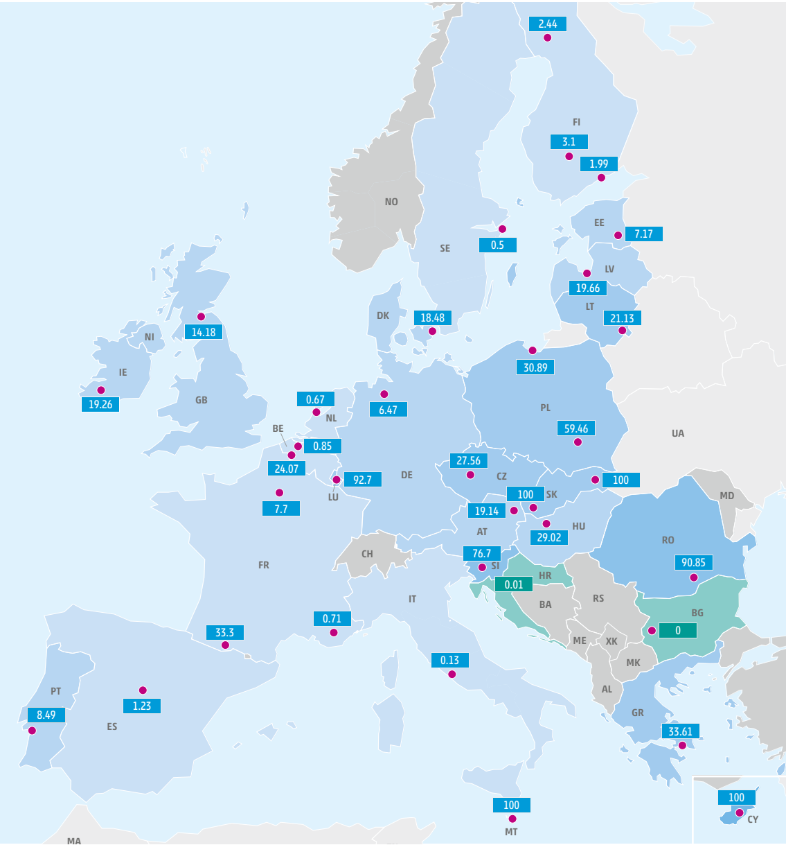
Figure 10: Yearly average hydrogen demand curtailment rate at country/sub-zone level in the PCI/PMI hydrogen infrastructure level in 2030 for reference weather year (unit: %).
