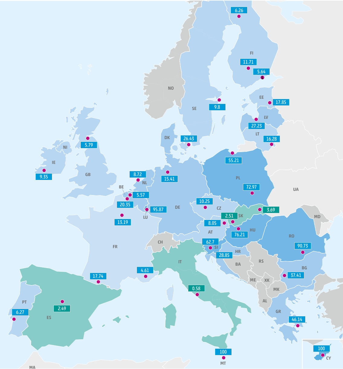
Figure 31: Yearly average hydrogen demand curtailment rate at country or node level in the PCI/PMI hydrogen infrastructure level in 2040 for stressful weather year (unit: %).
