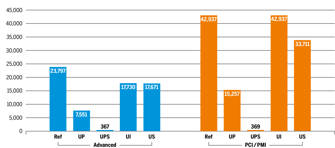
Figure 21: Shortage Advanced level and Shortage PCI/PMI level 2030 (unit: GWh/y).
