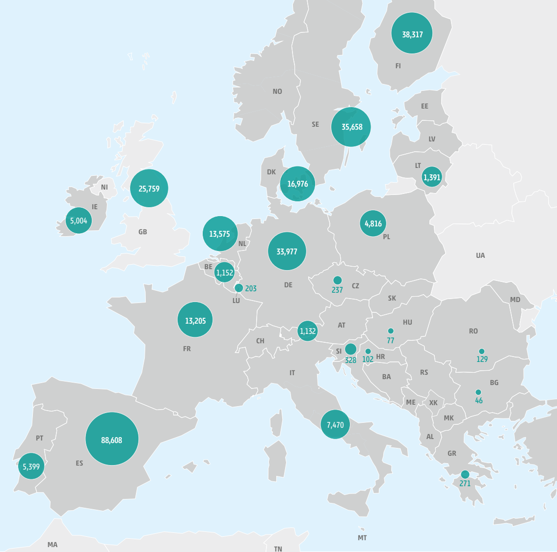
Figure 12: Distribution of hydrogen production via electrolysis in the Advanced hydrogen infrastructure level in 2030 for reference weather year (unit: GWh/y).
