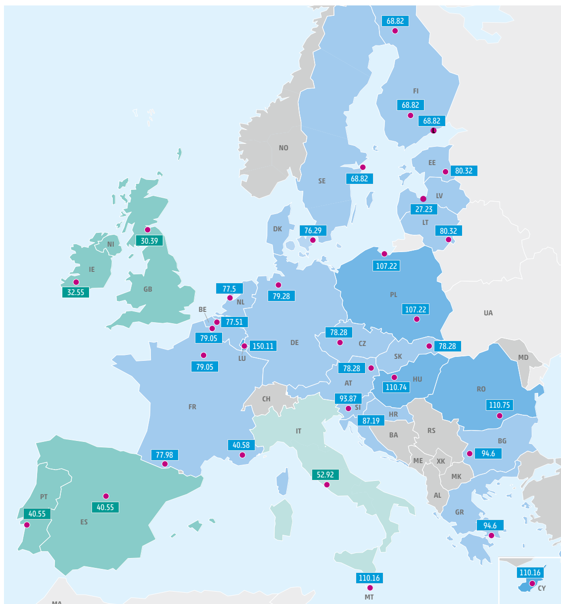
Figure 38: Average of the hourly hydrogen market clearing prices per country in the Advanced hydrogen infrastructure level in 2040 (unit: €/MWh).
