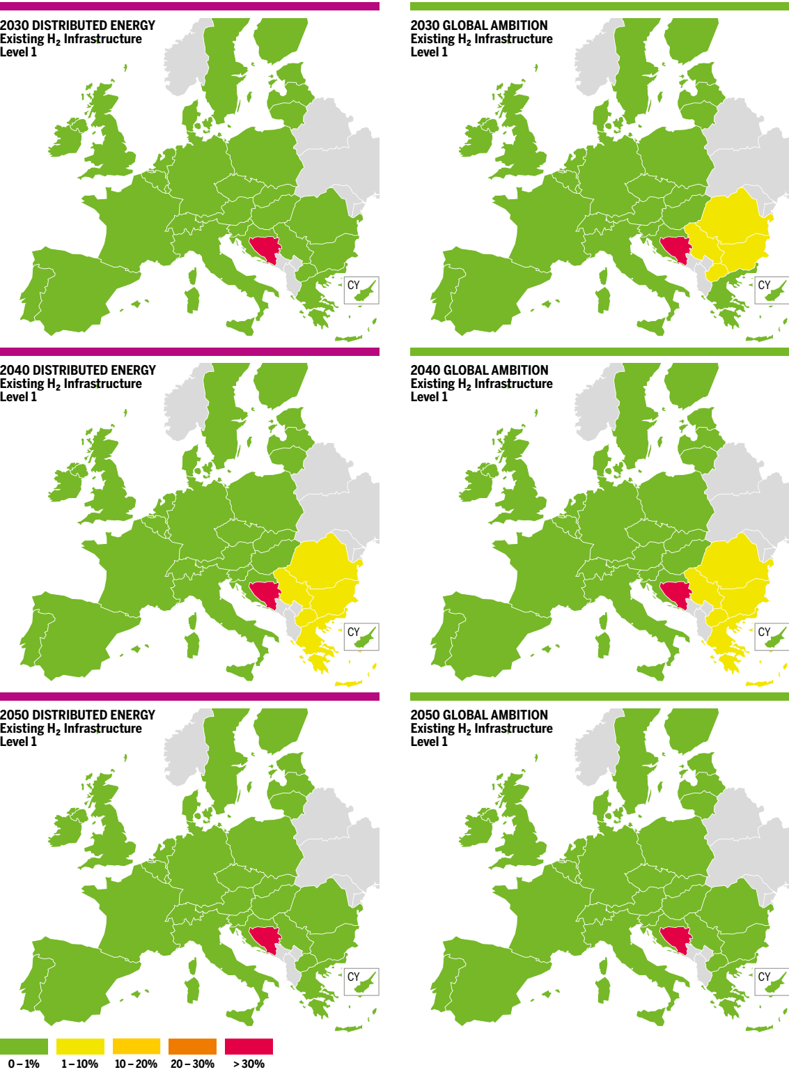
Figure 74a: UA H 2 Supply Disruption – Methane Results for 2W Demand in Existing CH 4 Infrastructure and H 2 Level 1
