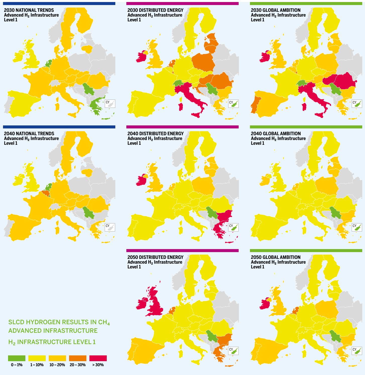
Figure 100: Hydrogen SLID Results for Peak Demand in Advanced CH 4 Infrastructure with H 2 Level 1
