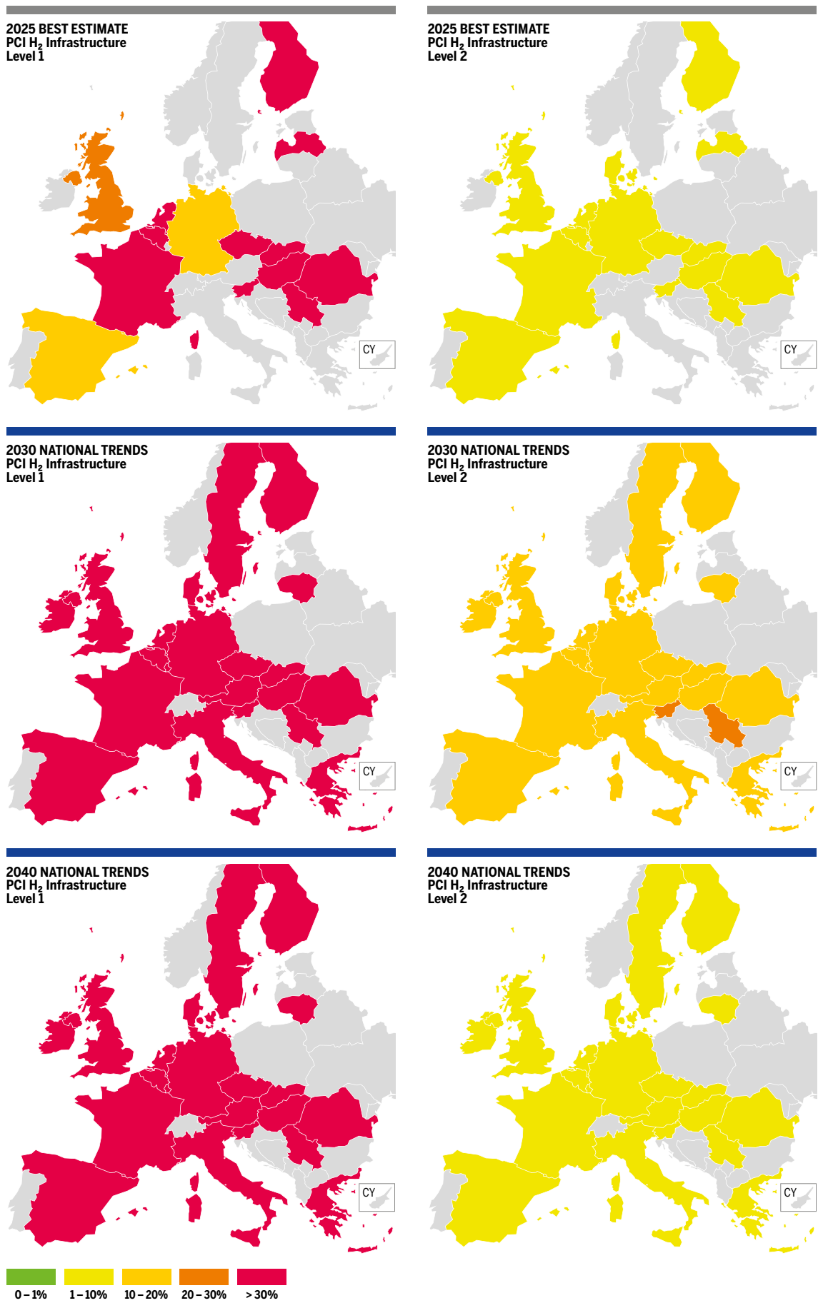
Figure 54a: RU CH 4 Supply Disruption – Hydrogen Results for Yearly Demand in PCI & Advanced CH 4 Infrastructure and H 2 Level 1 + 2
