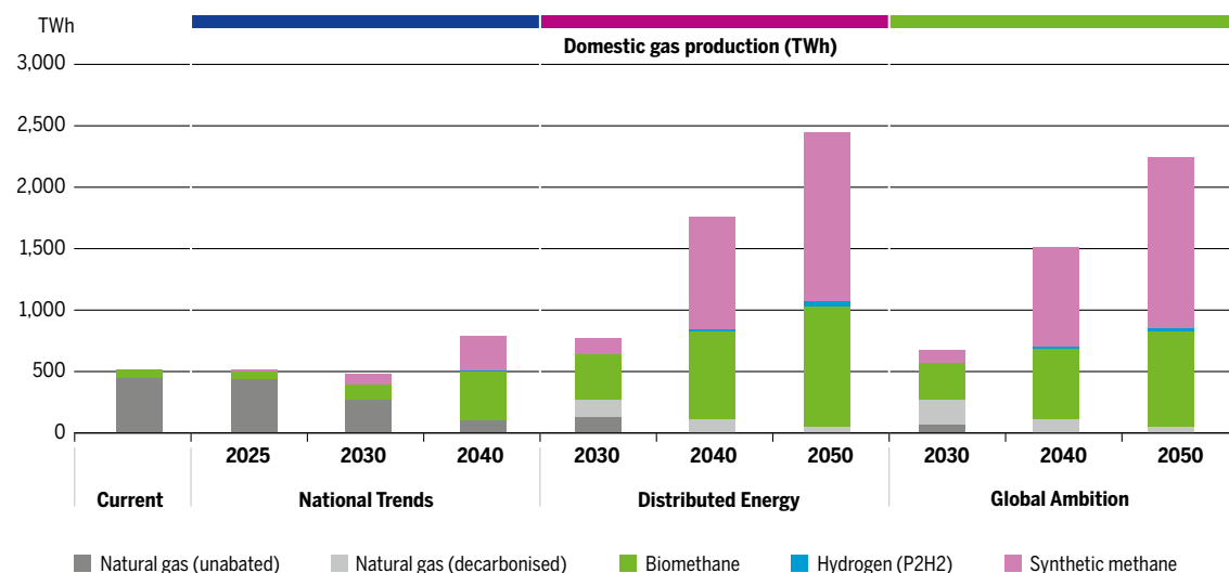
Figure 8: EU27 annual gas production per scenario (before REPowerEU adjustments)
