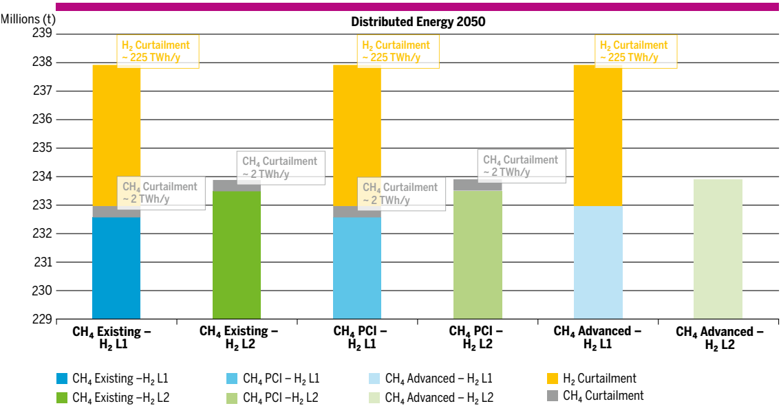
Figure 22: CO 2 emissions H 2 Levels 1 and 2 in 2050 Distributed Energy (million tons/year) combined CH 4 & H 2
