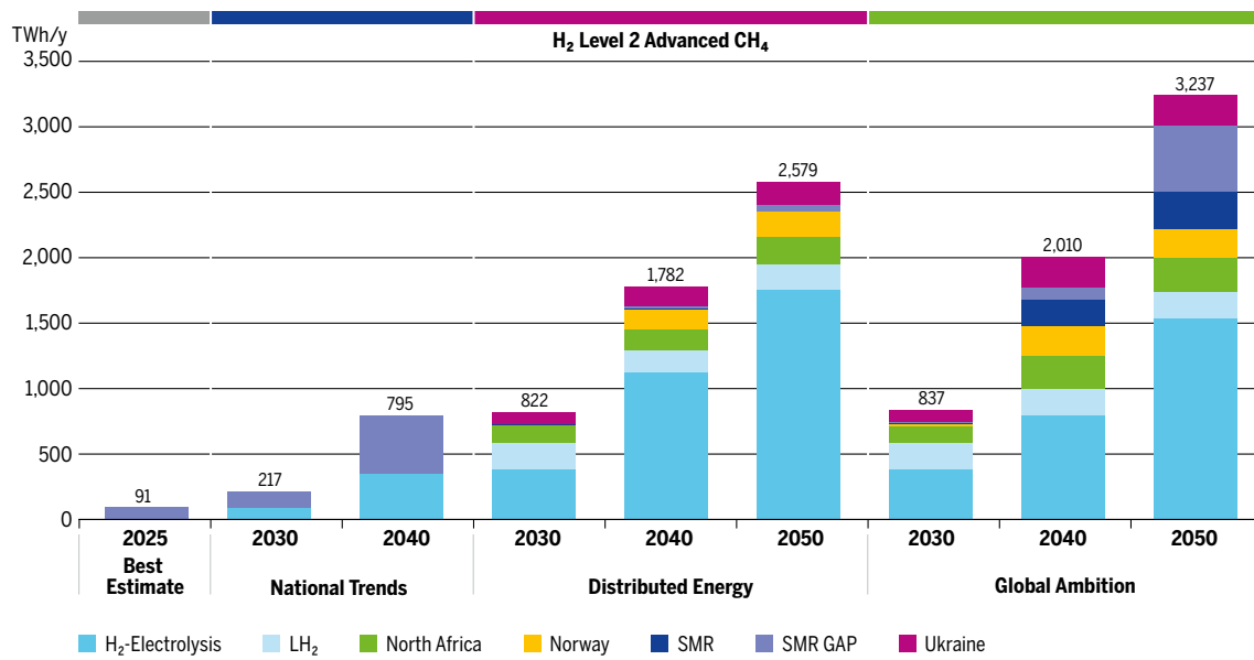
Figure 40: H 2 Yearly Supply Results in Advanced CH 4 Infrastructure with H 2 Level 2
