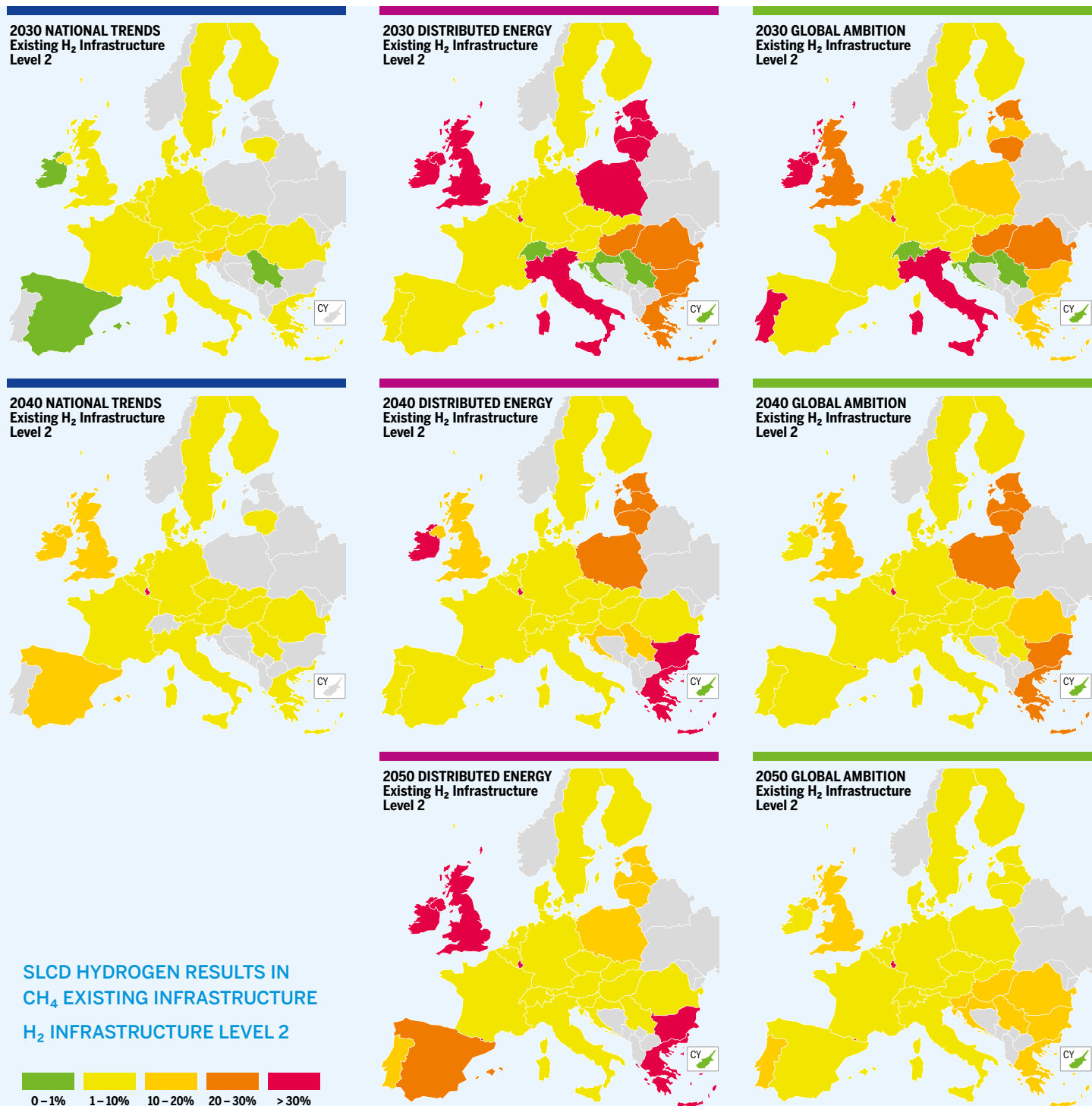
Figure 99: Hydrogen SLCD Results for Peak Demand in Existing CH 4 Infrastructure with H 2 Level 2
