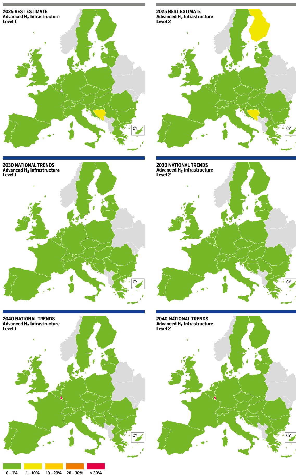
Figure 56b: RU CH 4 Supply Disruption – Methane Results for 2W Demand in PCI & Advanced CH 4 Infrastructure and H 2 Level 1 and 2
