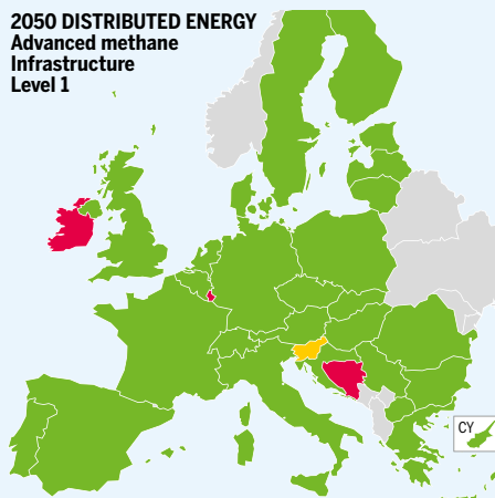
Figure 86: Methane SLID Results for Peak Demand in Advanced CH 4 Infrastructure with H 2 Level 1
