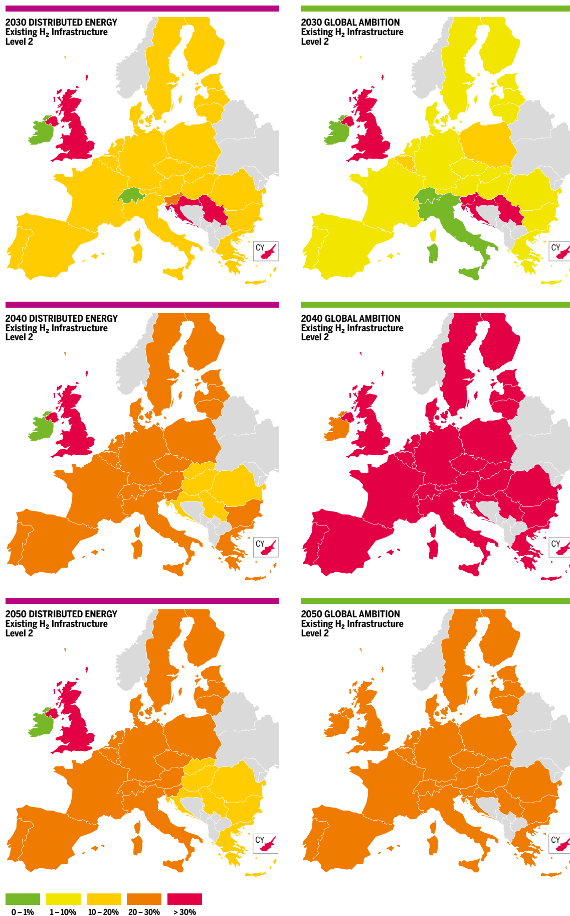
Figure 81b: LH 2 H 2 Supply Disruption – Hydrogen Results for 2W Demand in Existing CH 4 Infrastructure and H 2 Level 2
