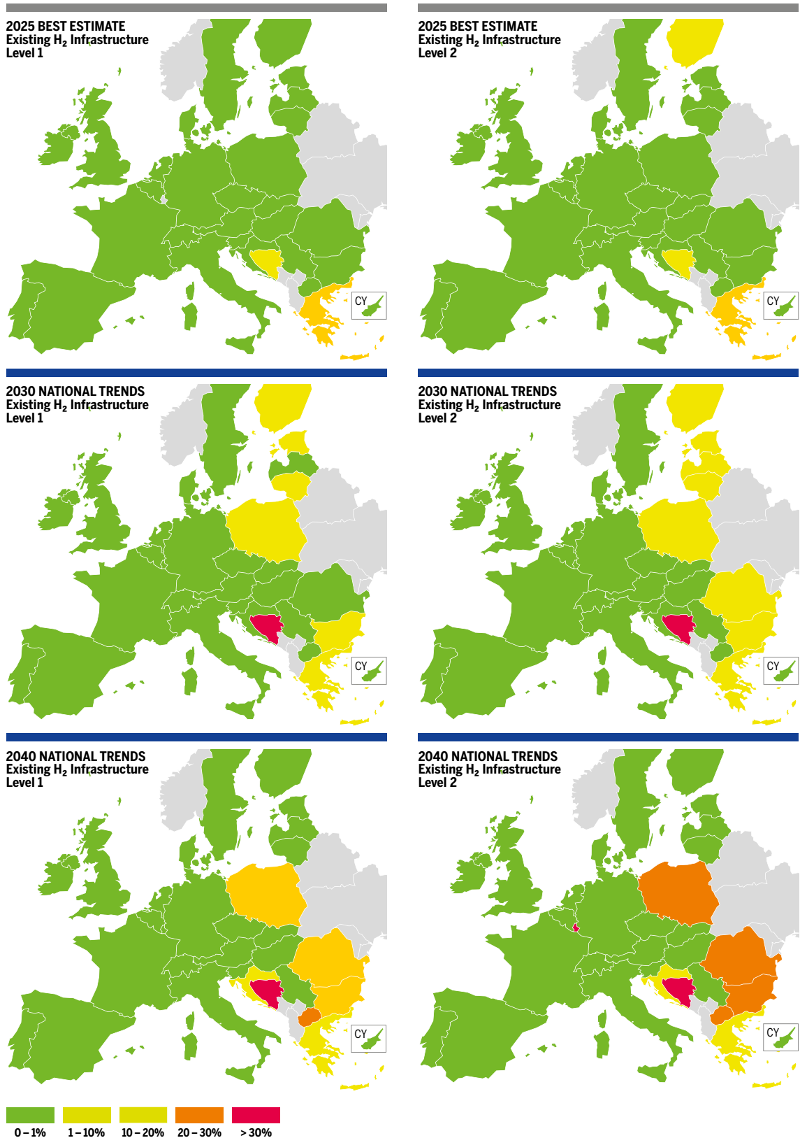
Figure 55: RU CH 4 Supply Disruption – Methane Results for 2W Demand in Existing CH 4 Infrastructure and H 2 Level 1 and 2
