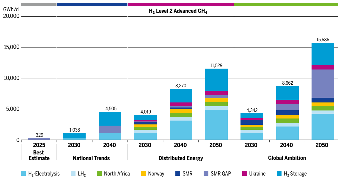
Figure 31: H 2 Supply Results for Peak Demand in Advanced CH 4 Infrastructure with H 2 Level 2
