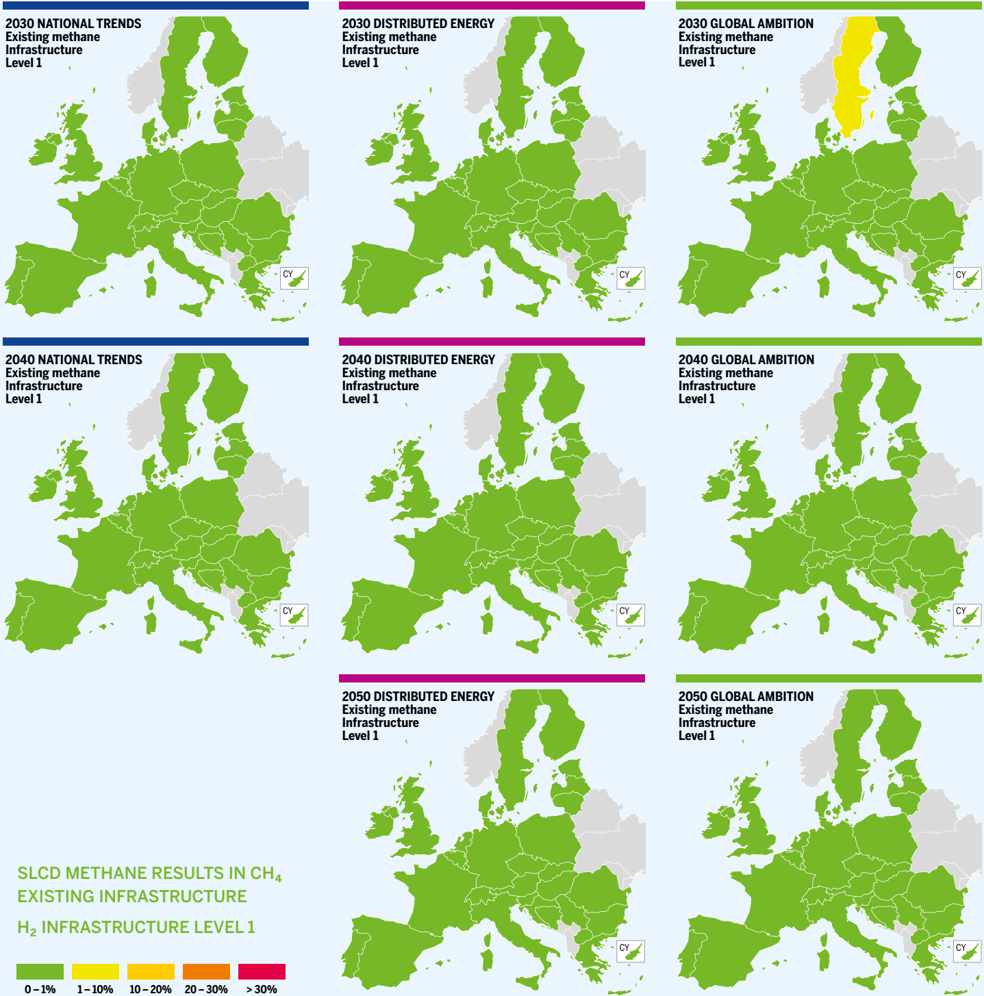
Figure 96: Methane SLCD Results for Peak Demand in Existing CH 4 Infrastructure with H 2 Level 1
