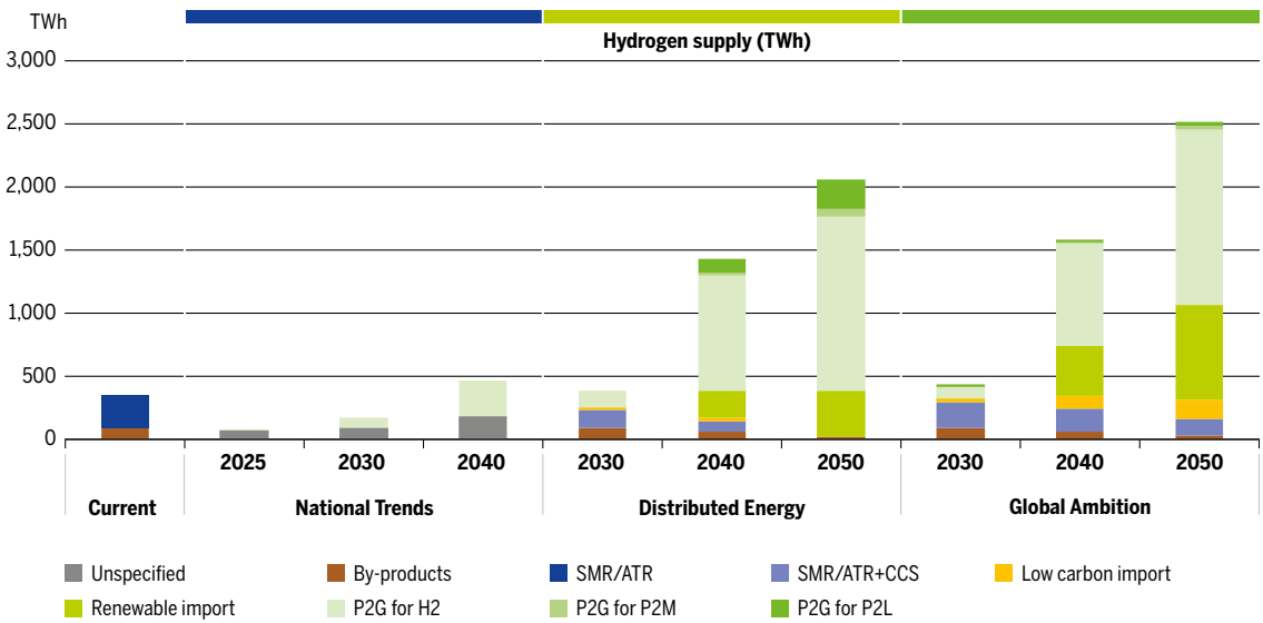
Figure 7: Hydrogen supply for EU27
