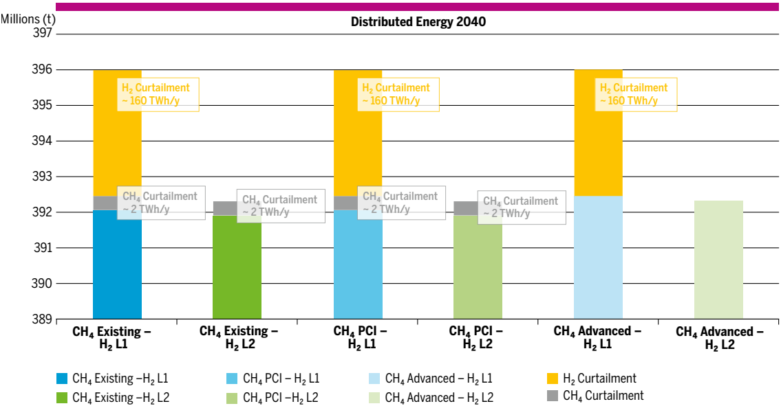
Figure 20: CO 2 emissions H 2 Levels 1 and 2 in 2040 Distributed Energy (million tons/year) combined CH 4 & H 2
