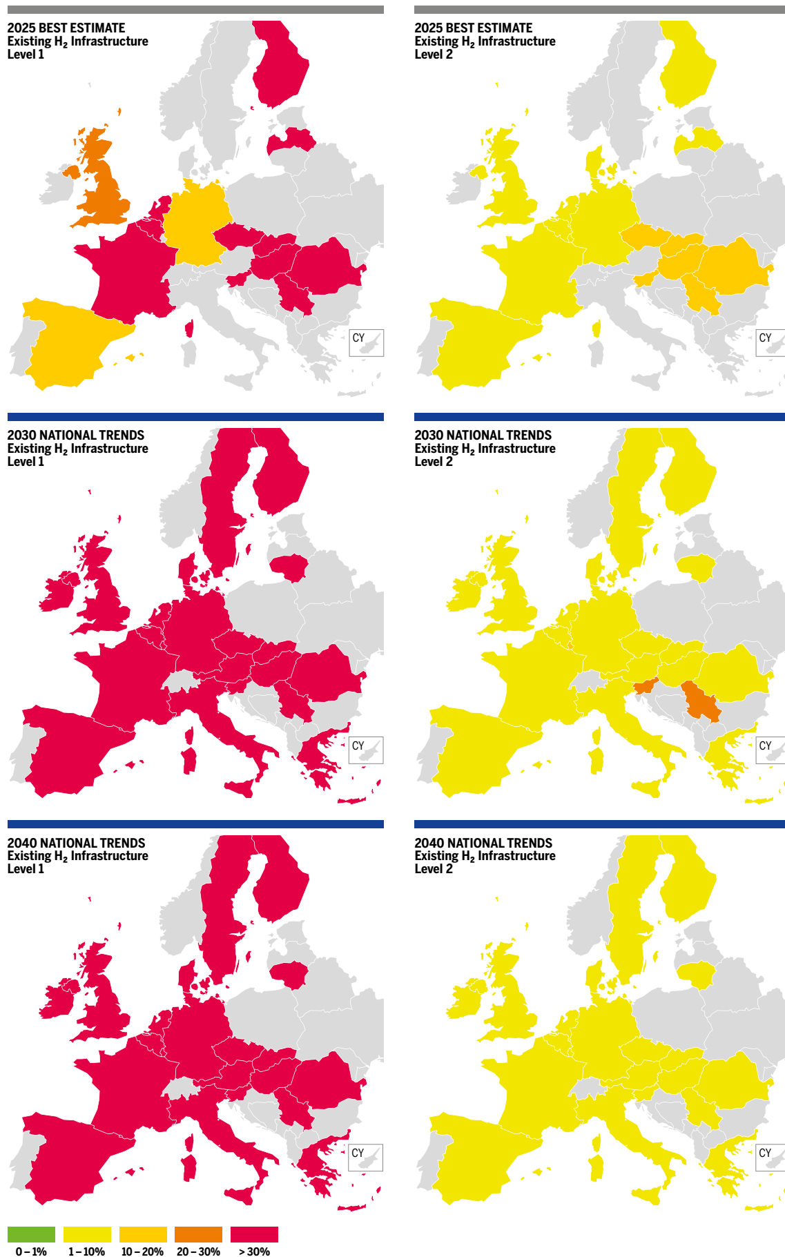
Figure 53: RU CH 4 Supply Disruption – Hydrogen Results for Yearly Demand in Existing CH 4 Infrastructure and H 2 Level 1 and 2
