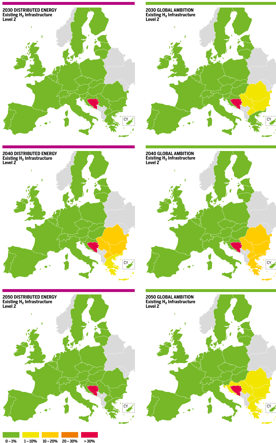
Figure 74b: UA H 2 Supply Disruption – Methane Results for 2W Demand in Existing CH 4 Infrastructure and H 2 Level 2
