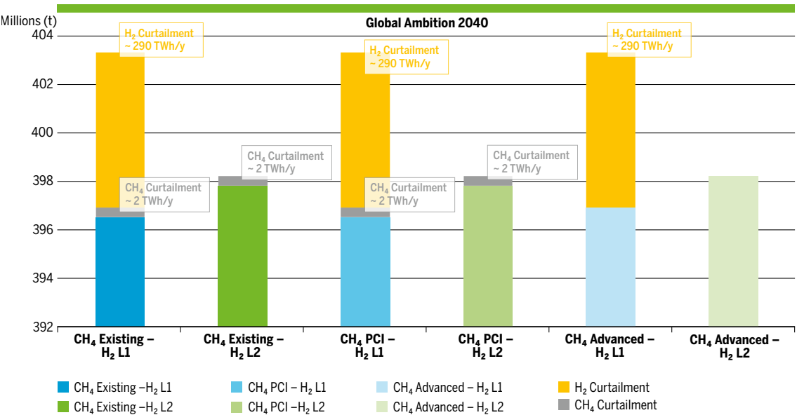
Figure 21: CO 2 emissions H 2 Levels 1 and 2 in 2040 Global Ambition (million tons/year) combined CH 4 & H 2
