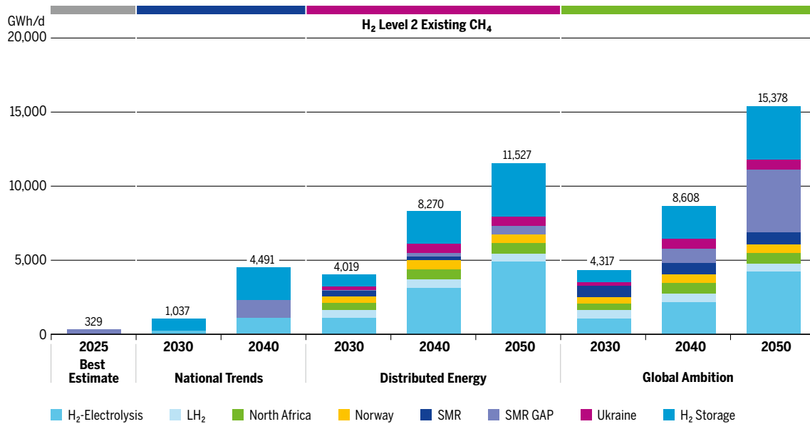
Figure 30: H 2 Supply Results for Peak Demand in Existing CH 4 Infrastructure with H 2 Level 2
