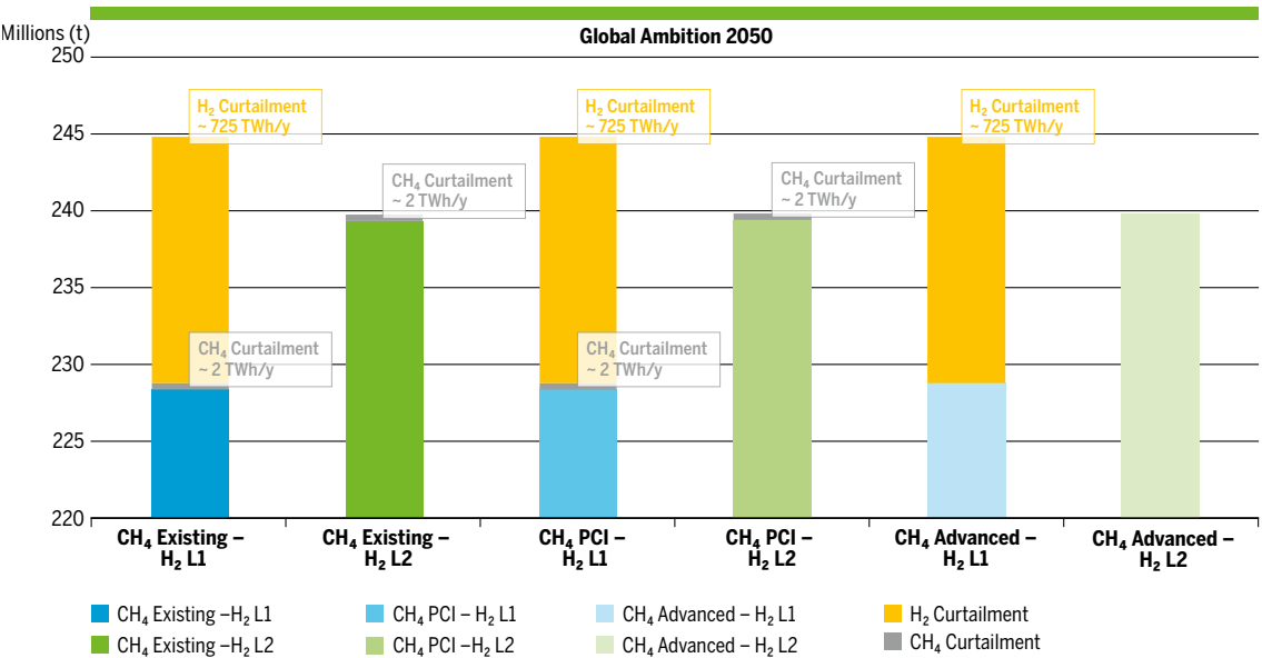
Figure 23: CO 2 emissions H 2 Levels 1 and 2 in 2050 Global Ambition (million tons/year) combined CH 4 & H 2
