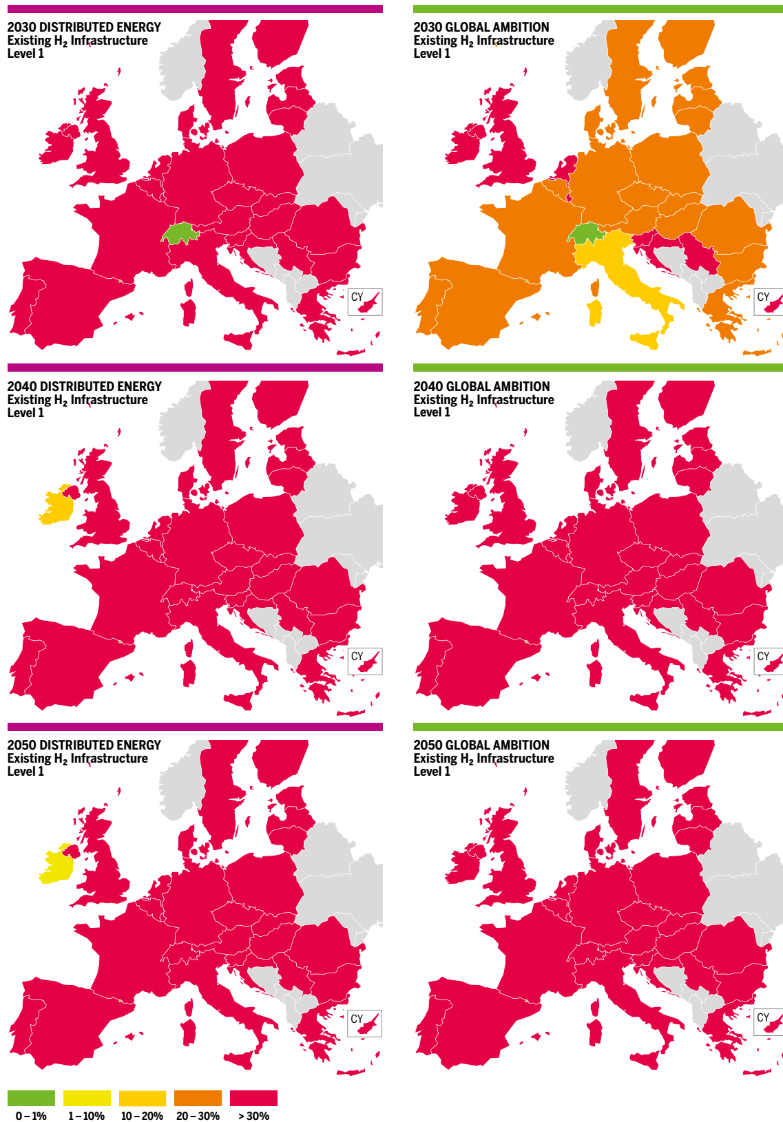
Figure 83a: LH 2 H 2 Supply Disruption – Hydrogen Results for Peak Demand in Existing CH 4 Infrastructure and H 2 Level 1
