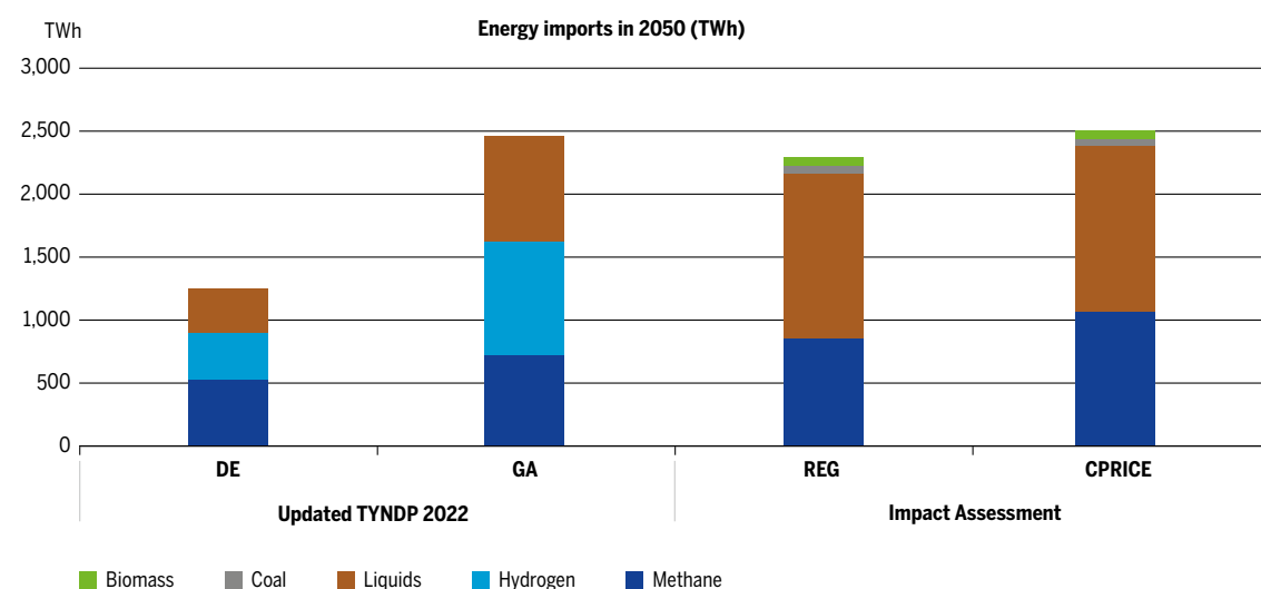
Figure 9: Energy imports to the EU in 2050 in TYNDP 2022 scenarios and EU Impact Assessment
