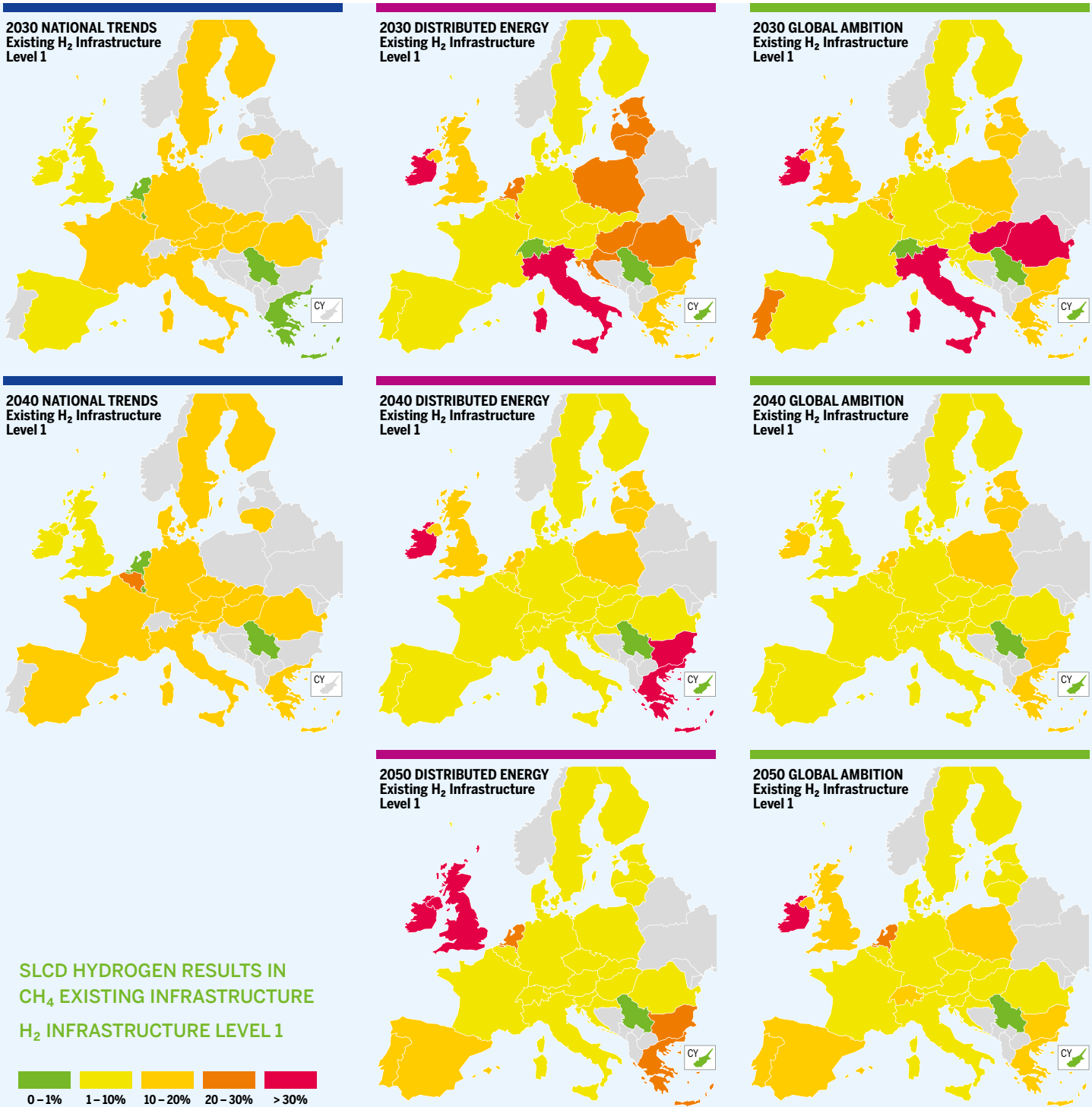
Figure 98: Hydrogen SLCD Results for Peak Demand in Existing CH 4 Infrastructure with H 2 Level 1
