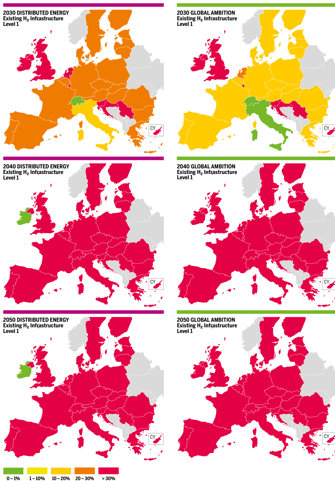
Figure 70a: NO 2 Supply Disruption – Hydrogen Results for 2W Demand in Existing CH 4 Infrastructure and H 2 Level 1
