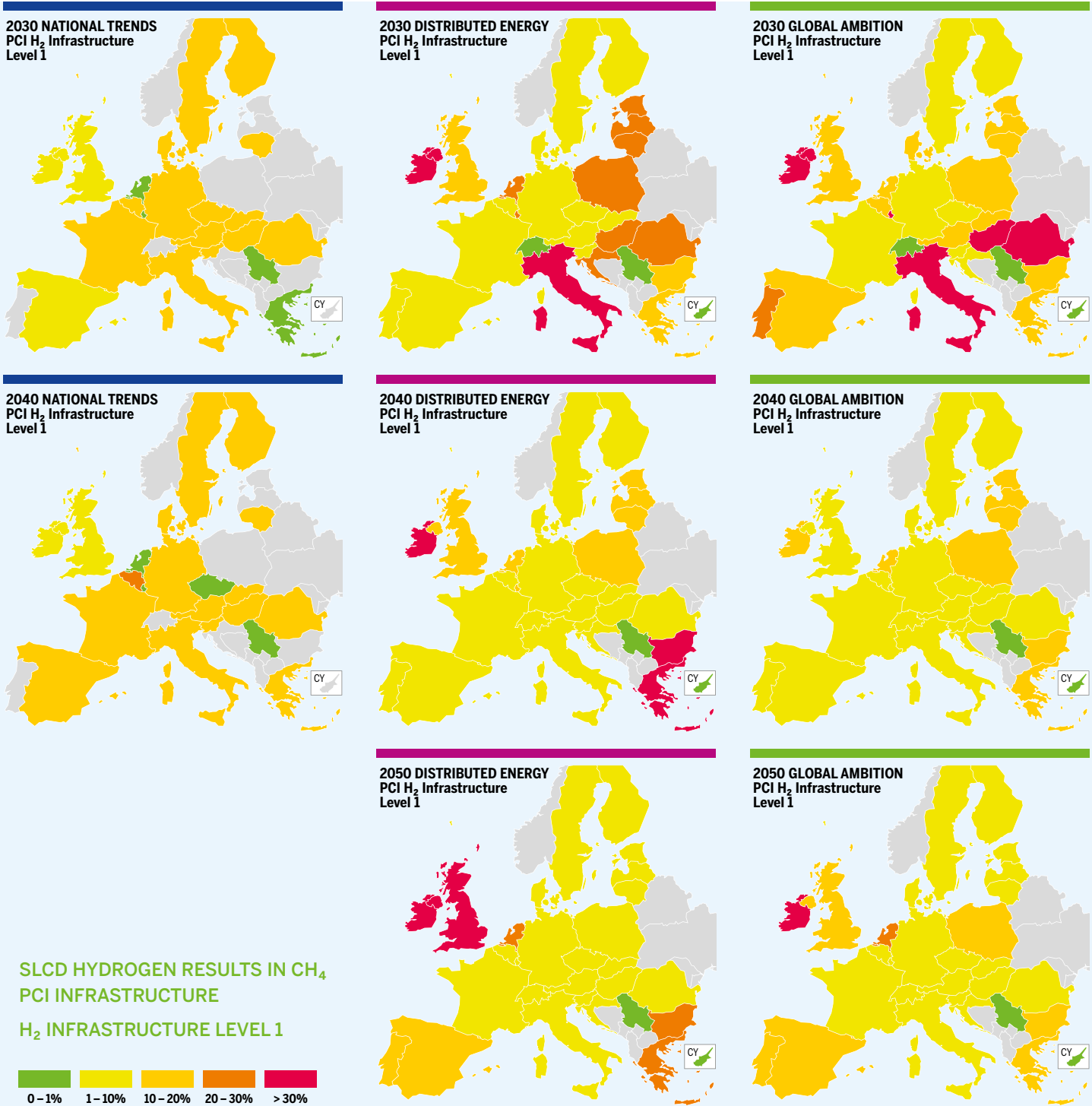
Figure 102: Hydrogen SLCD Results for Peak Demand in PCI CH 4 Infrastructure with H 2 Level 1
