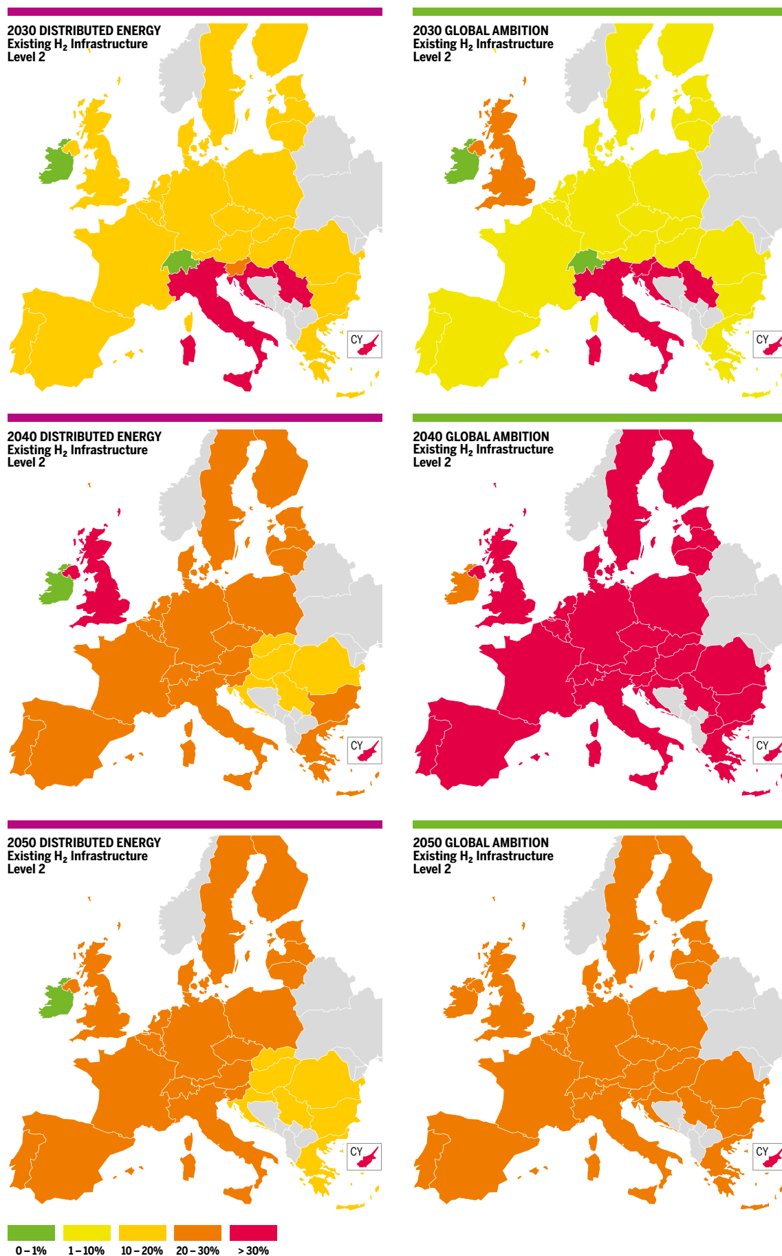
Figure 66b: NA H 2 Supply Disruption – Hydrogen Results for 2W Demand in Existing CH 4 Infrastructure and H 2 Level 2
