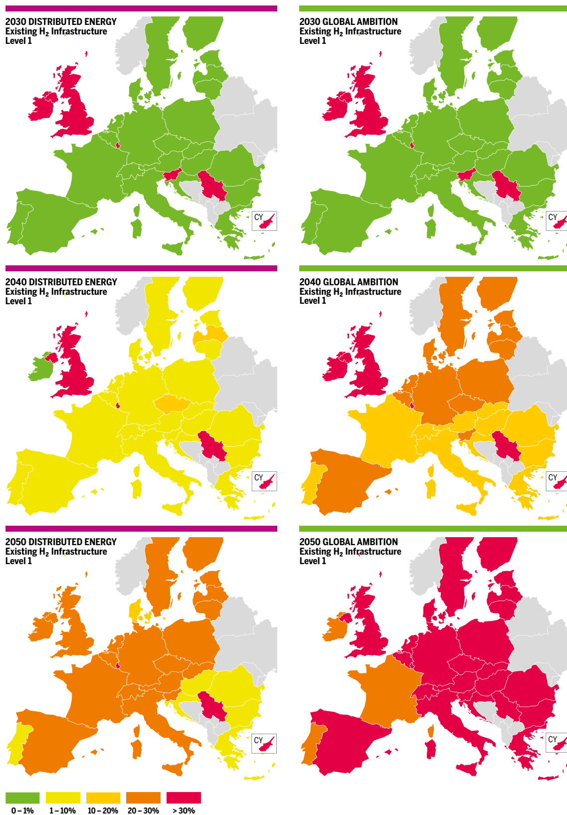
Figure 69a: NO 2 Supply Disruption – Hydrogen Results for Yearly Demand in Existing CH 4 Infrastructure and H 2 Level 1
