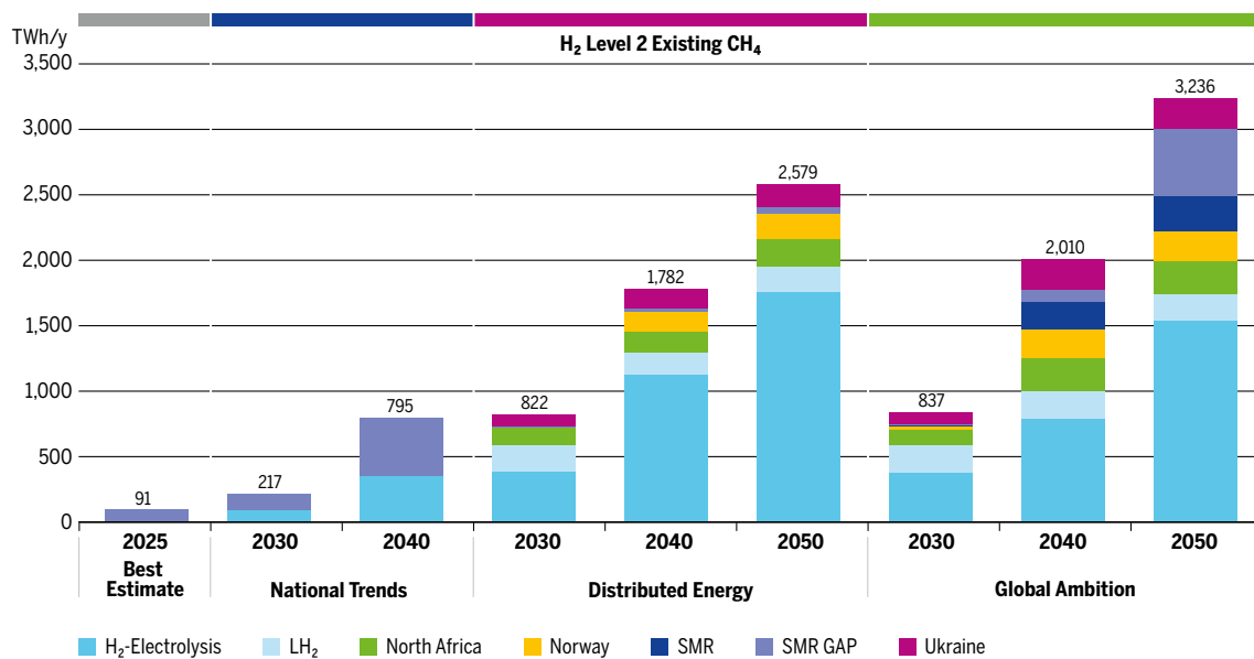
Figure 39: H 2 Yearly Supply Results in Existing CH 4 Infrastructure with H 2 Level 2
