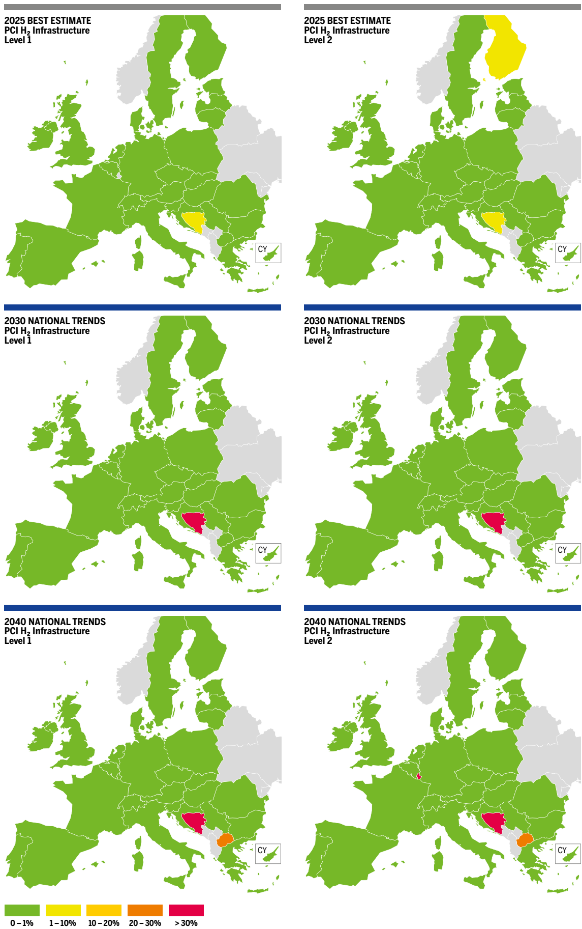
Figure 56a: RU CH 4 Supply Disruption – Methane Results for 2W Demand in PCI & Advanced CH 4 Infrastructure and H 2 Level 1 and 2
