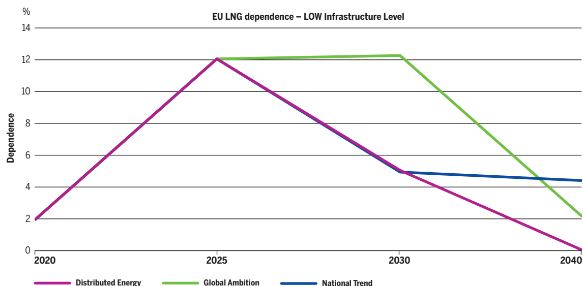
Figure 4.7 Overall EU dependence on LNG supply in the Low infrastructure level.
