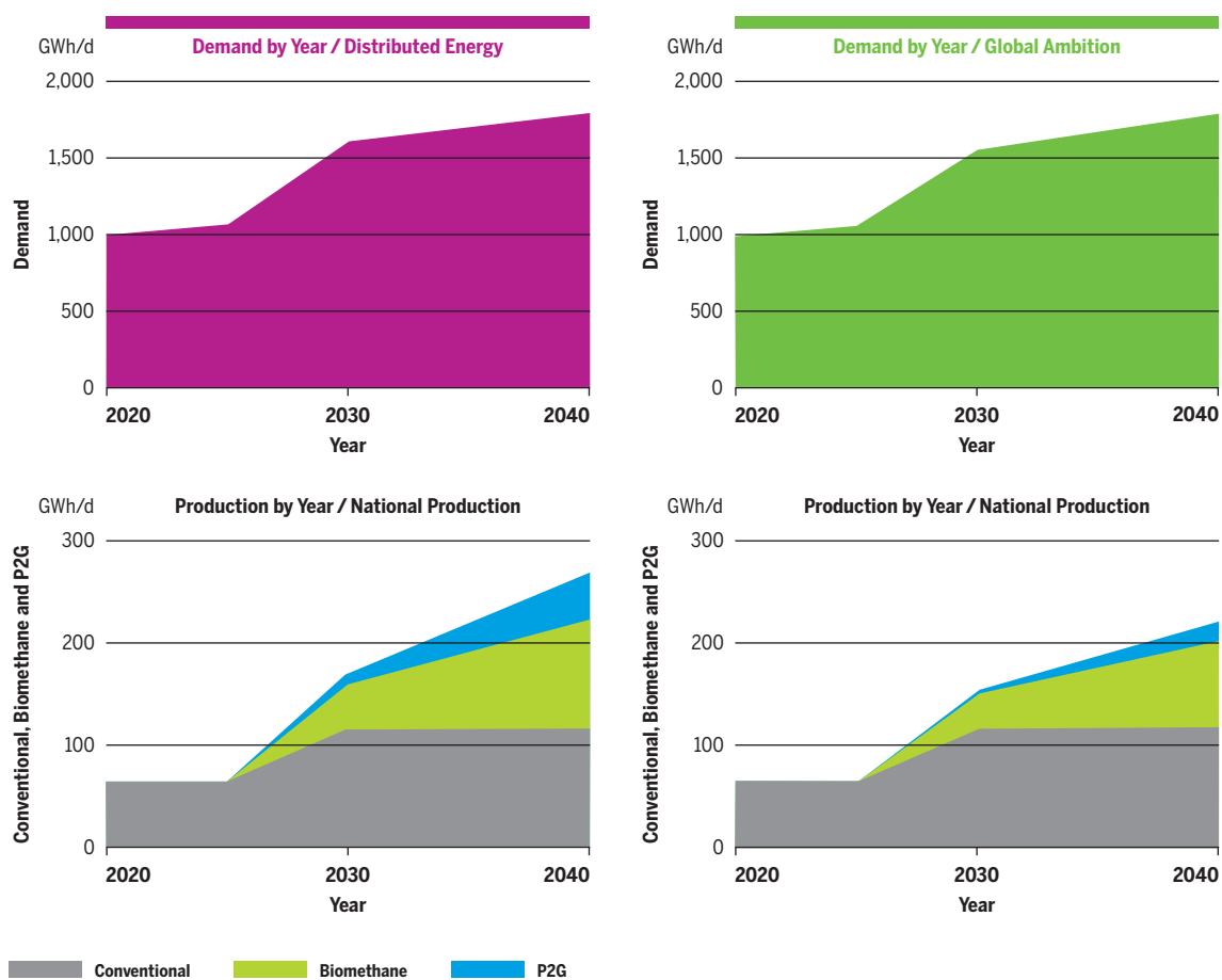
Figure 3.18 2-week cold spell demand and production in Poland in COP 21 scenarios in GWh/d.
