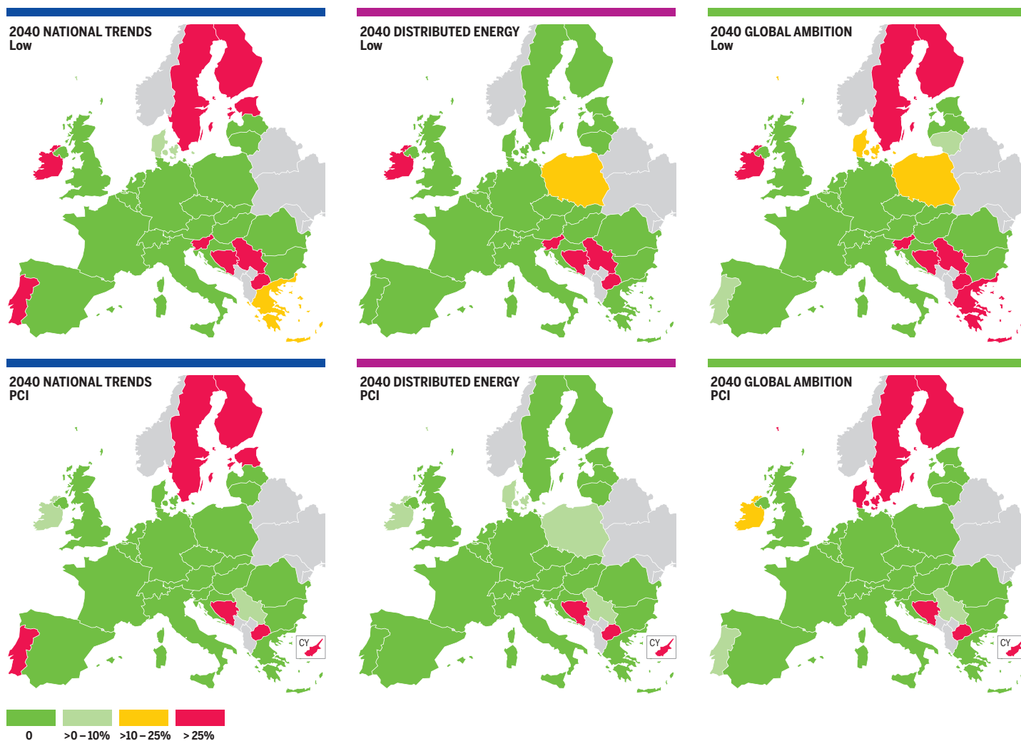
Figure 3.127 Maximum exposure to demand curtailment in case of SLID in Low and PCI infrastructure levels in 2040 for all scenarios.
