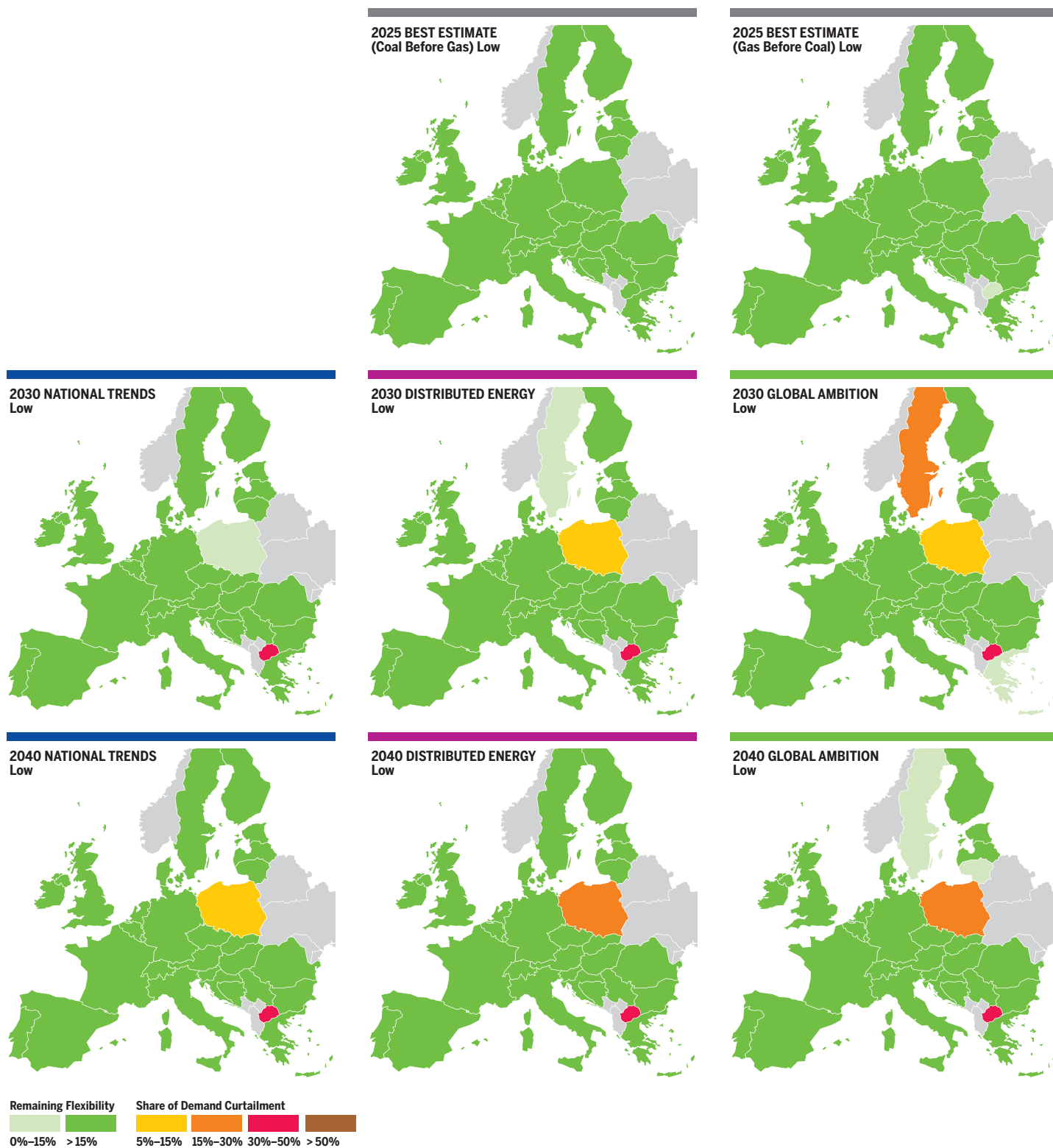
Figure 3.74 Low infrastructure level: Belarus transit disruption under 2-week Dunkelflaute situation.
