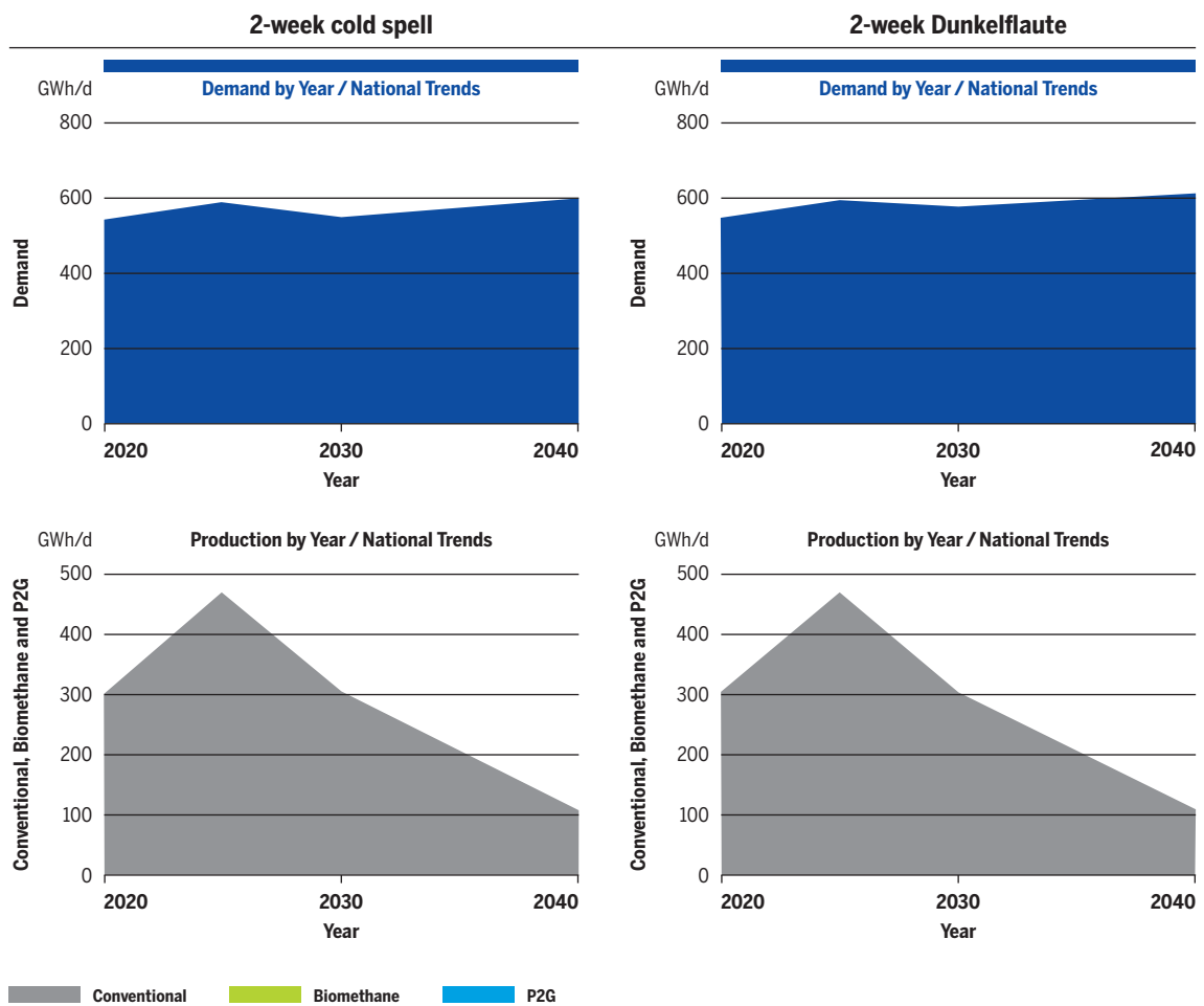
Figure 3.53 2-week cold spell/Dunkelflaute demand and production in Romania in National Trends scenario in GWh/d.
