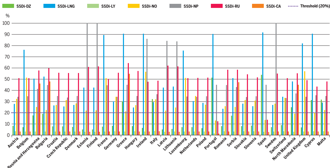
Figure 4.76 SSDi – PCI infrastructure level – Distributed Energy 2040
