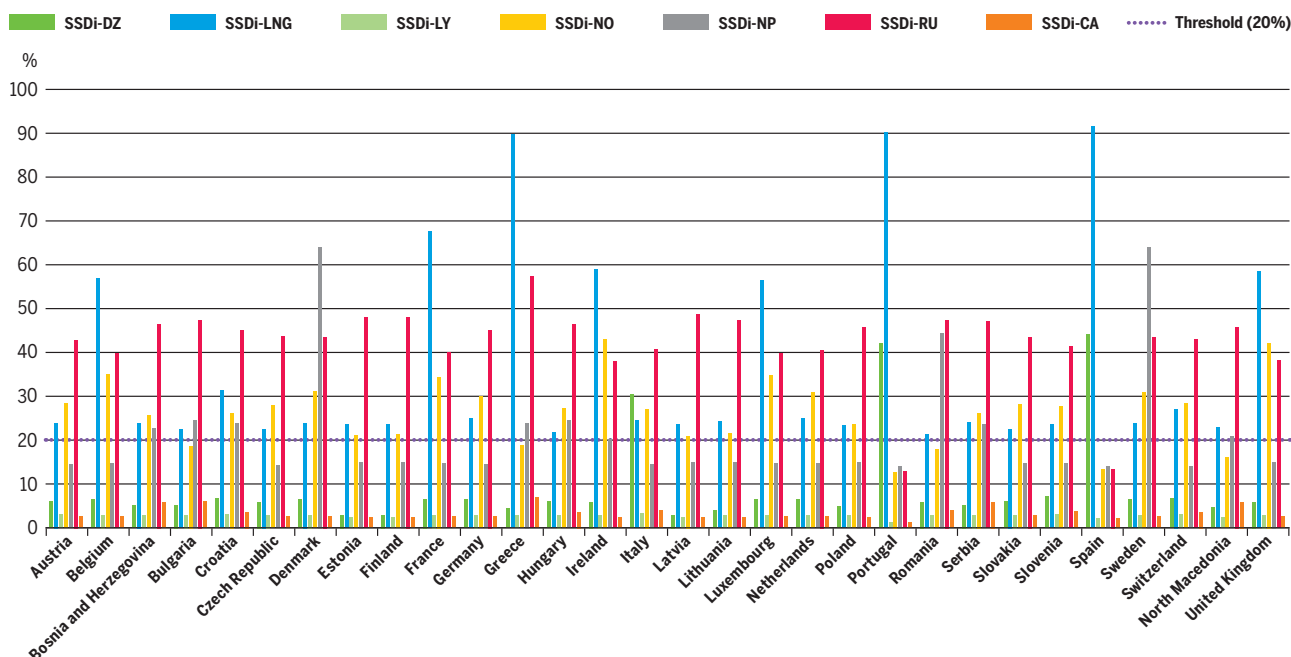
Figure 4.59 SSDi – Low infrastructure level – Global Ambition 2030
