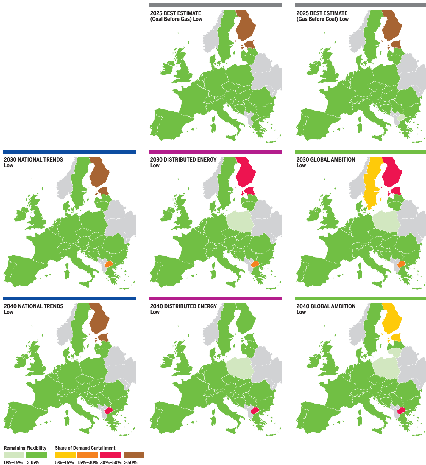
Figure 3.86 Low infrastructure level: Baltics States and Finland transit disruption under 2-week cold sell situation.
