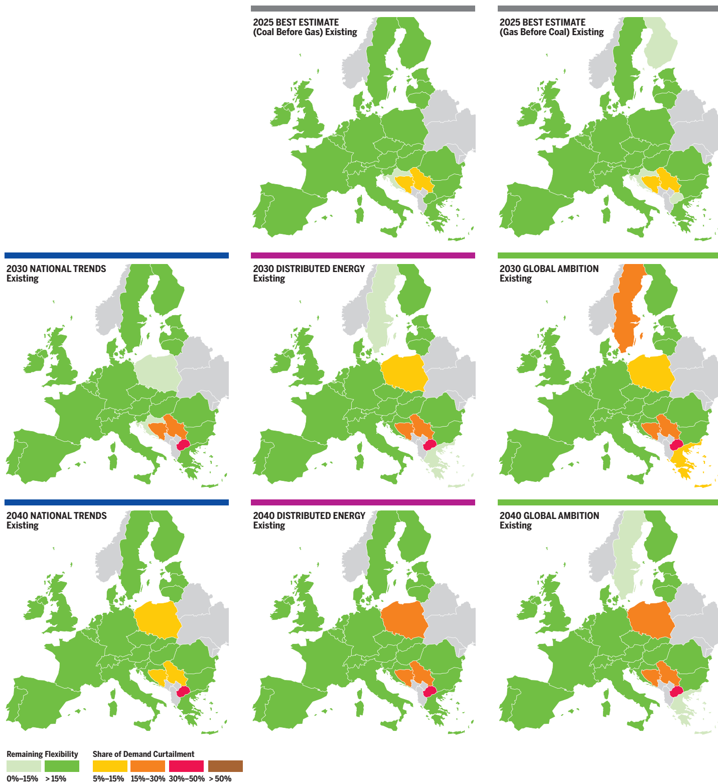
Figure 3.33 Existing infrastructure level: Climatic Stress under 2-wek Dunkelflaute situation.
