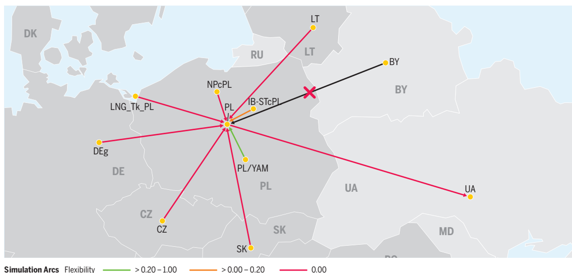
Figure 3.62 Infrastructure limitations towards Poland under Belarus transit disruption, Low infrastructure, Global Ambition, 2040
