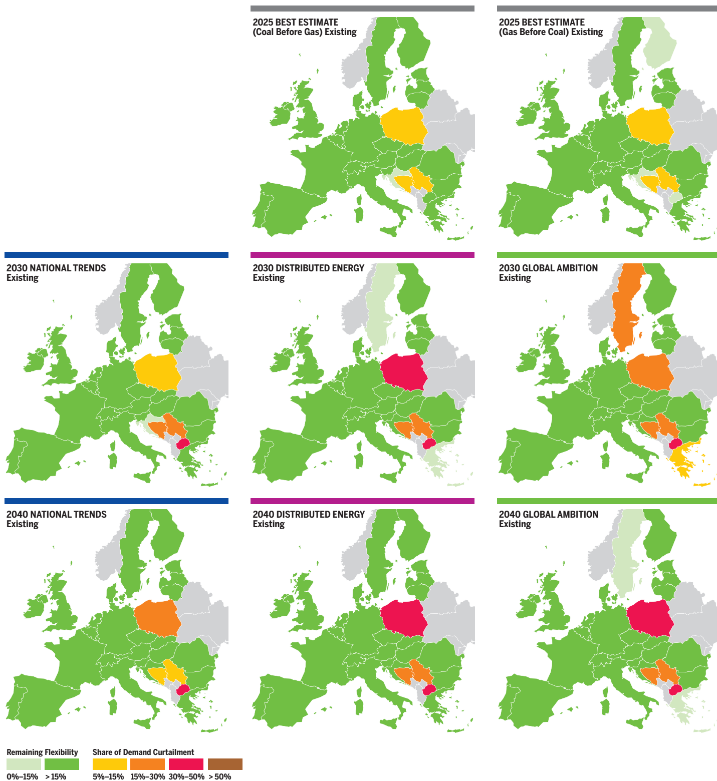
Figure 3.73 Existing infrastructure level: Belarus transit disruption under 2-week Dunkelflaute situation.
