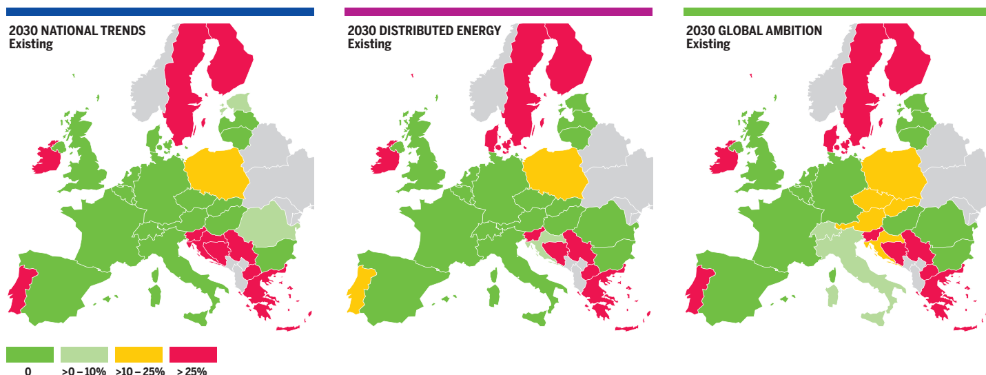
Figure 3.117 Maximum exposure to demand curtailment in case of SLID in Existing Infrastructure level in 2030 for all scenarios.
