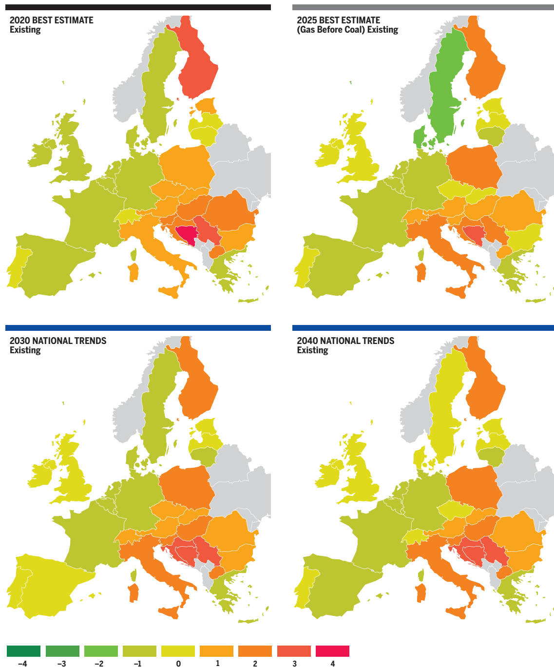
Figure 4.84 MP delta (EUR/MWh) – Existing infrastructure level, South Max supply configuration
