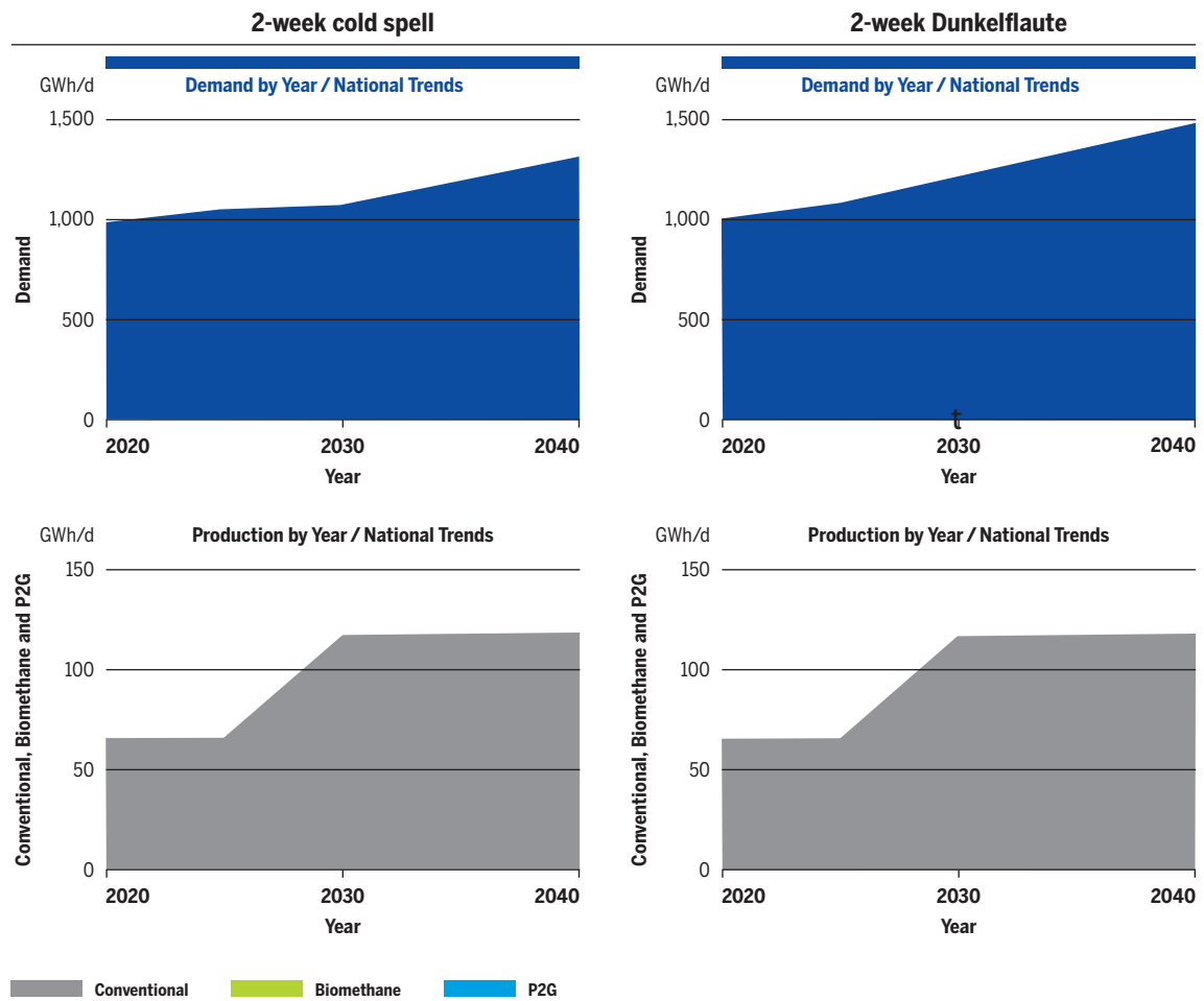
Figure 3.26 2-week cold spell/Dunkelflaute demand and production in Poland in National Trends scenario in GWh/d.
