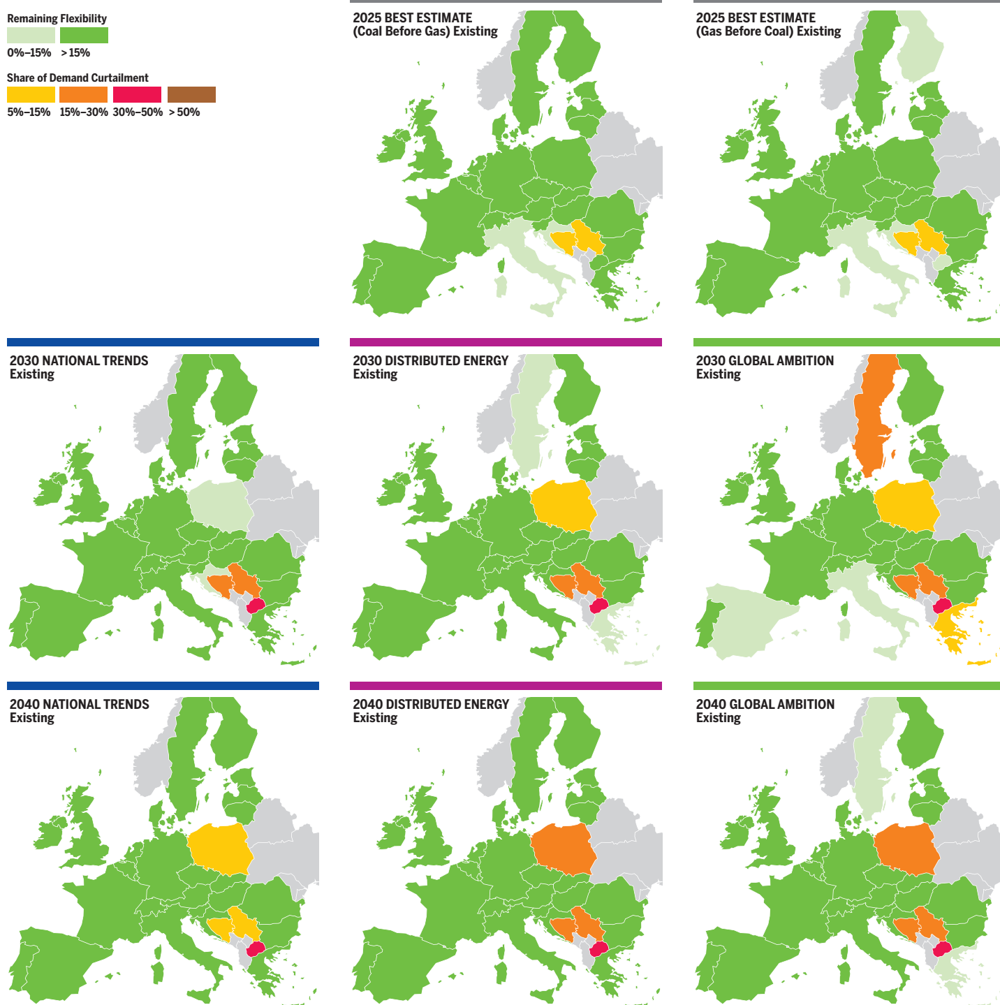
Figure 3.103 Existing infrastructure level: Algerian pipeline import route disruption under 2-week Dunkelflaute situation.
