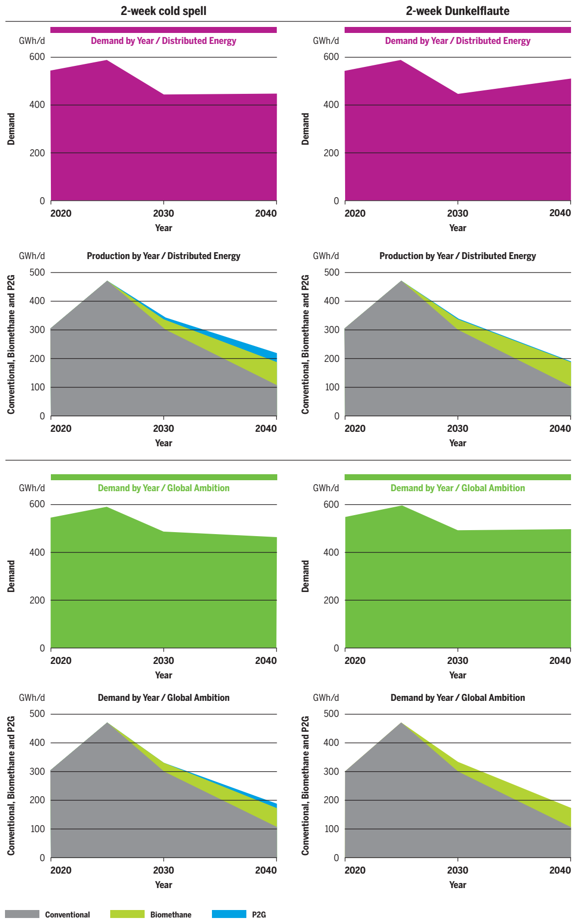
Figure 3.54 2-week cold spell/Dunkelflaute demand and production in Romania in Distributed Energy & Global Ambition scenarios in GWh/d.
