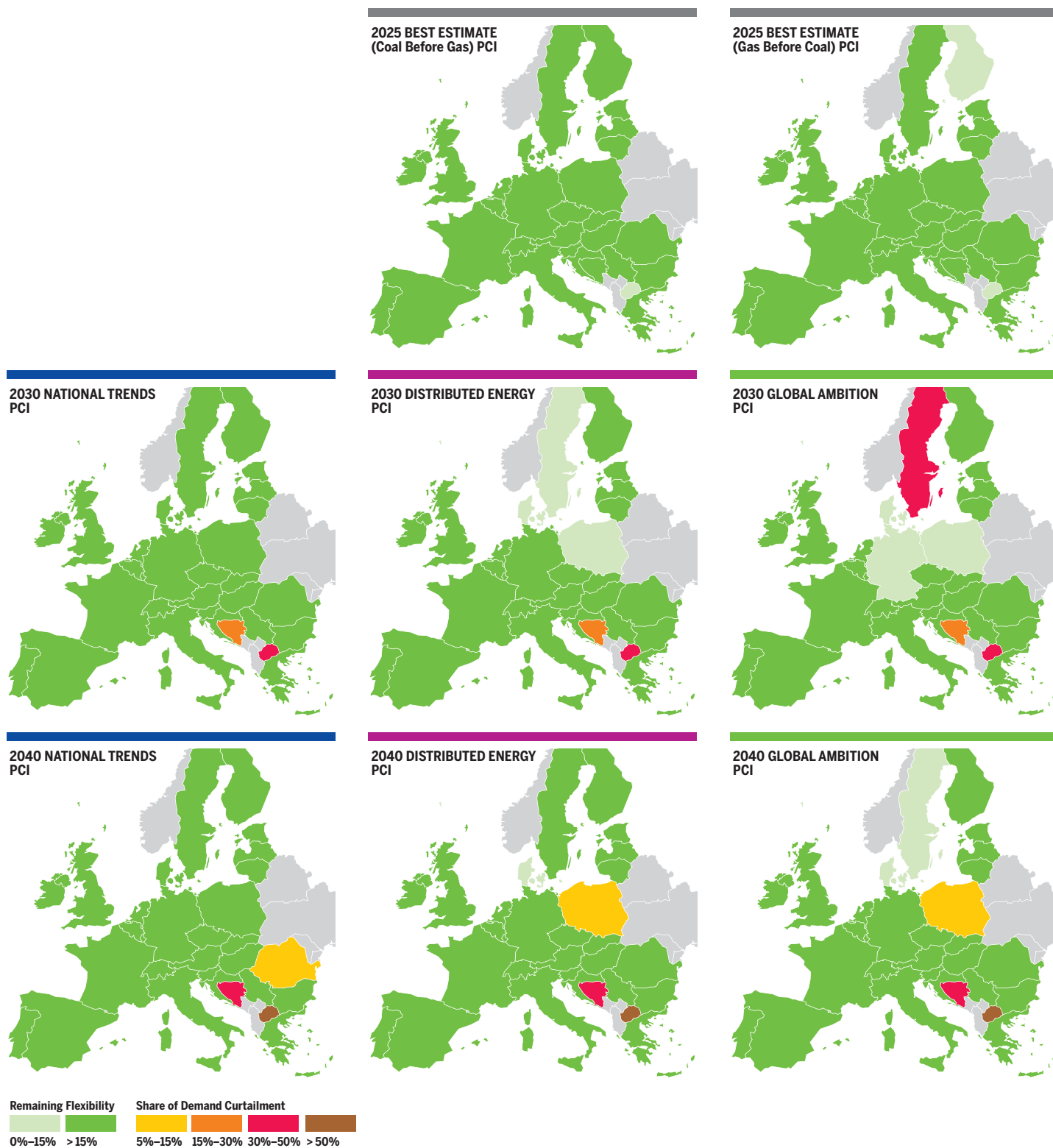
Figure 3.44 PCI infrastructure level: Ukraine transit disruption under peak day situation.
