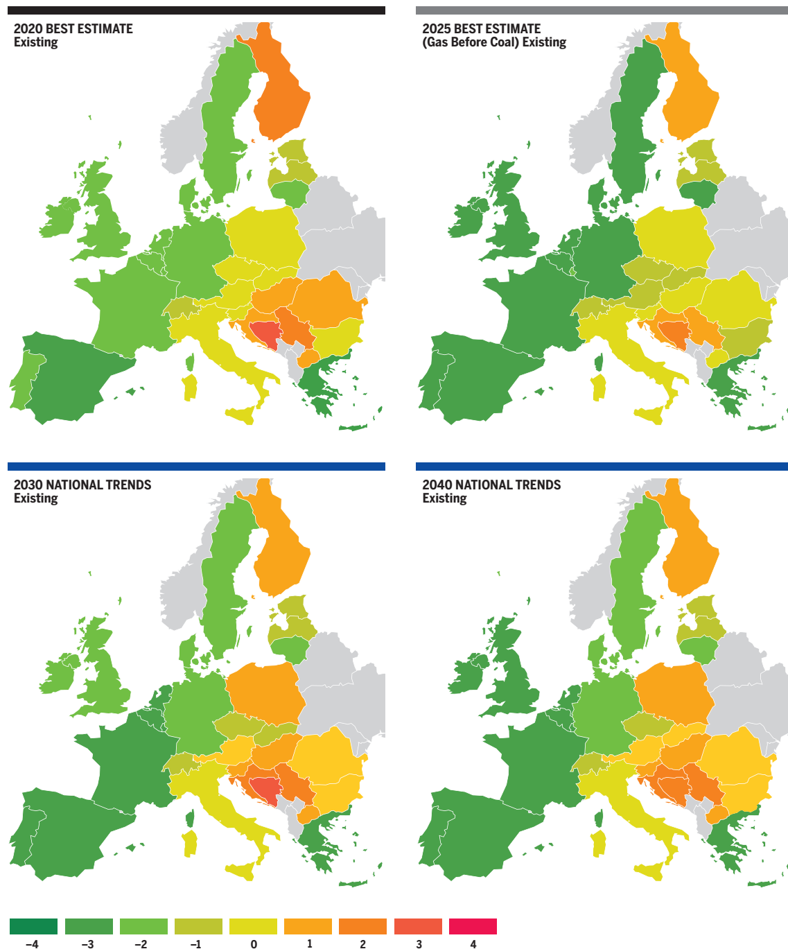
Figure 4.80 MP delta (EUR/MWh) – Existing infrastructure level, LNG Max supply configuration
