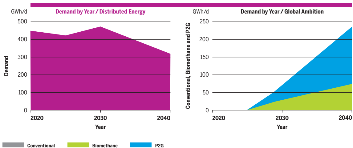
Figure 4.21 Demand and production evolution in the Baltic states and Finland in Distributed Energy scenario.
