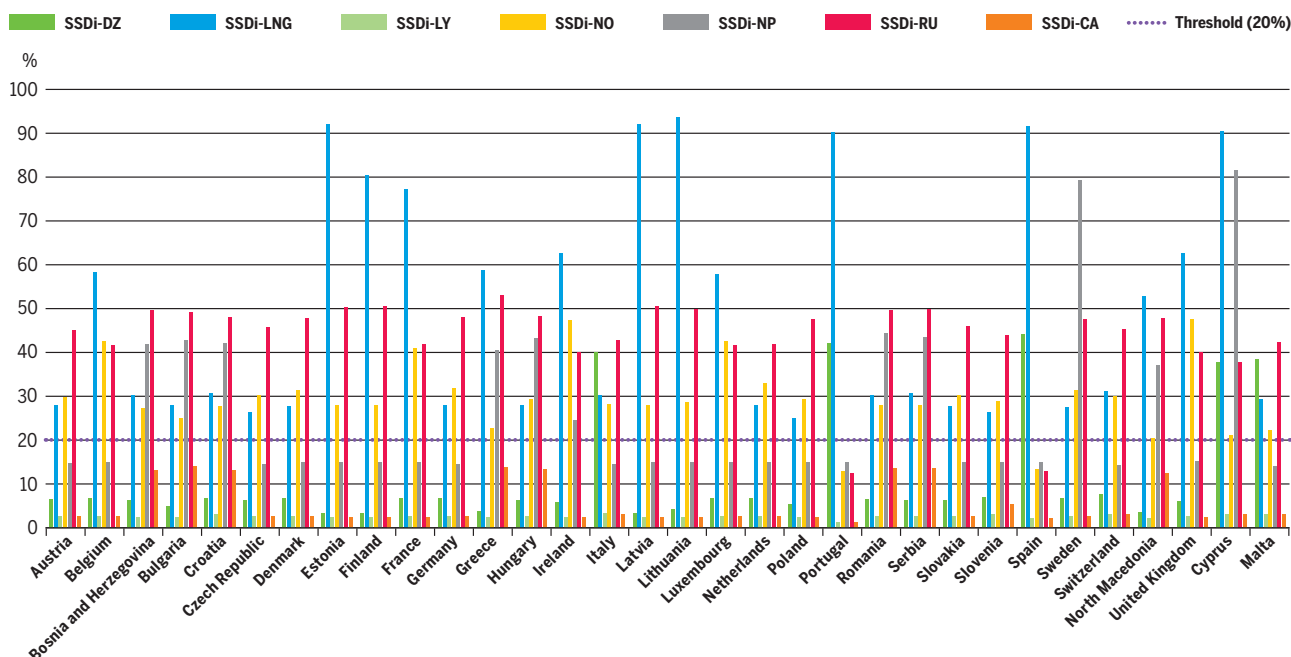
Figure 4.66 SSDi – Advanced infrastructure level – Distributed Energy 2030
