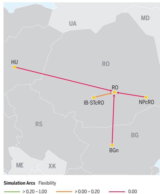
Figure 3.38 Infrastructure limitations towards Romania under Ukraine disruption, Existing infrastructure, 2025.
