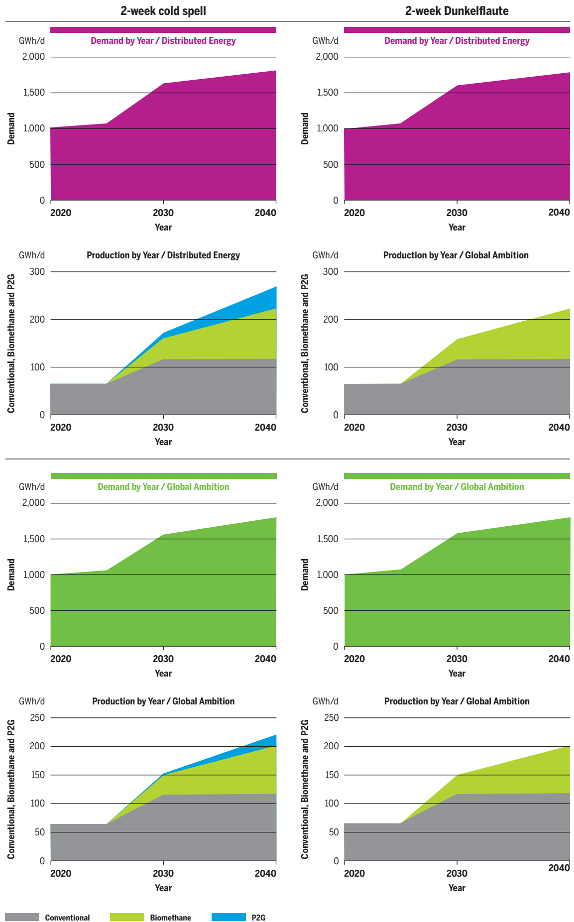
Figure 3.28 2-week cold spell/Dunkelflaute demand and production in Poland in Distributed Energy & Global Ambition scenarios in GWh/d.
