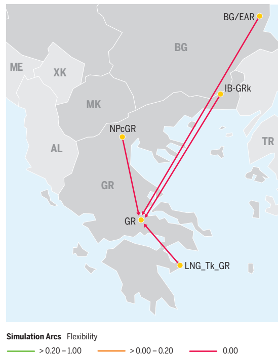
Figure 3.29 Infrastructure limitations towards Greece, Existing infrastructure, Global Ambition 2030.
