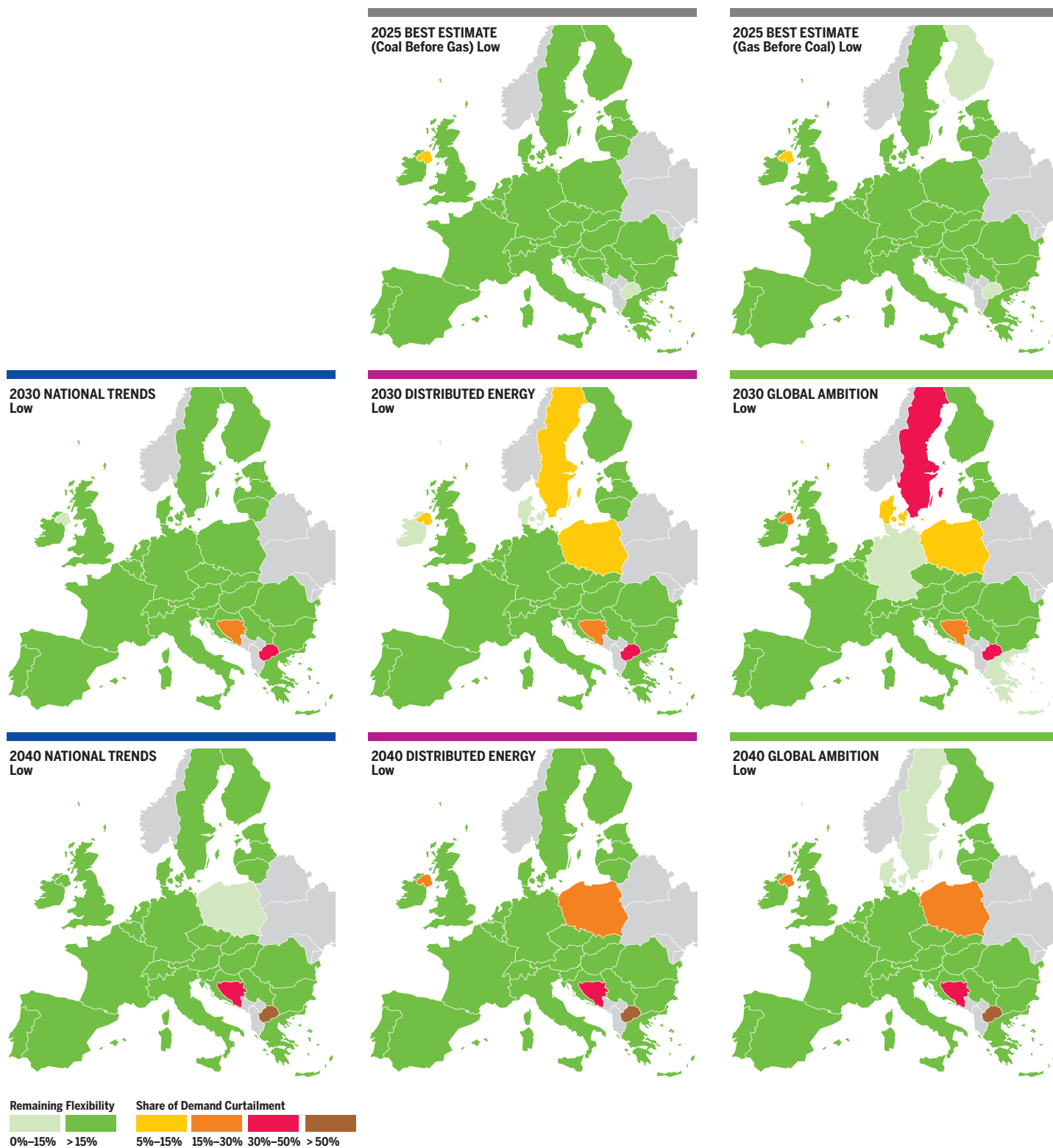
Figure 3.12 Low infrastructure level: Climatic Stress under a peak day situation.
