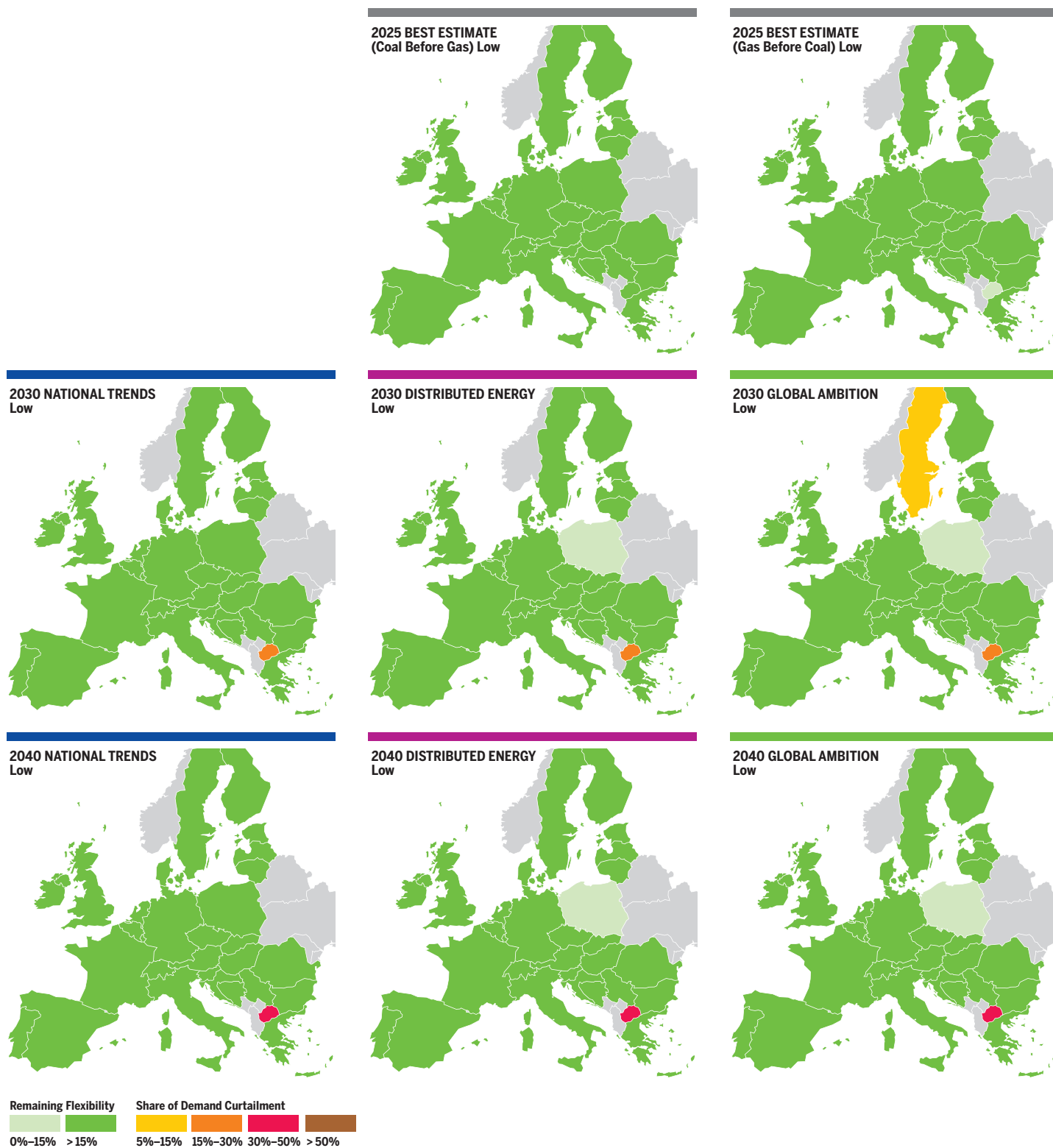
Figure 3.21 Low infrastructure level: Climatic Stress under 2-week cold spell situation.
