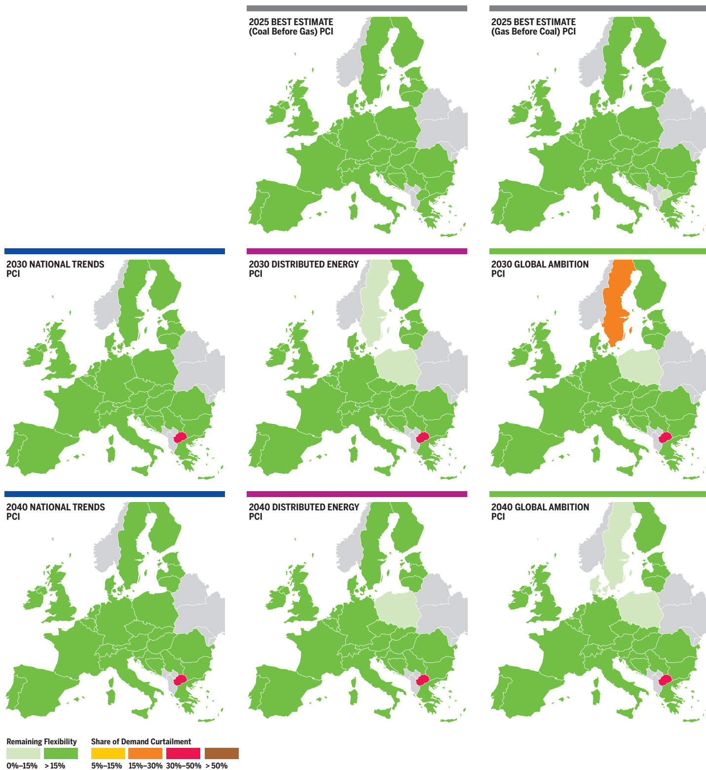
Figure 3.76 PCI infrastructure level: Belarus transit disruption under 2-week Dunkelflaute situation.
