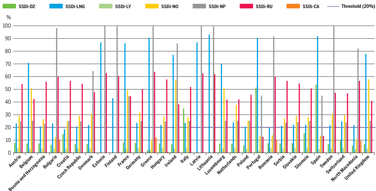
Figure 4.49 SSDi – Existing infrastructure level – Distributed Energy 2040
