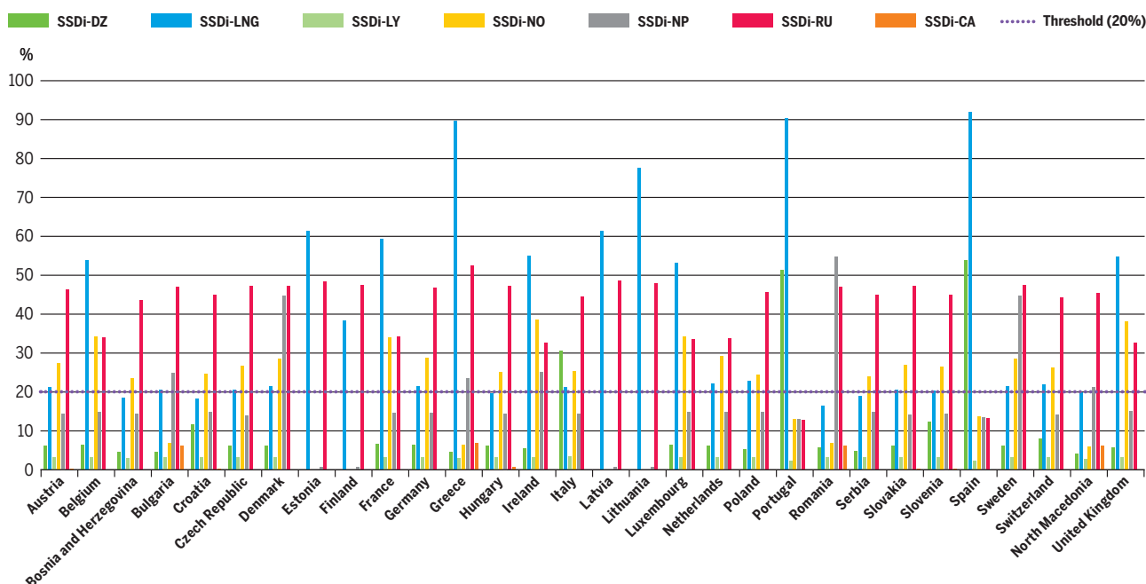
Figure 4.45 SSDi – Existing infrastructure level – Gas Before Coal 2025
