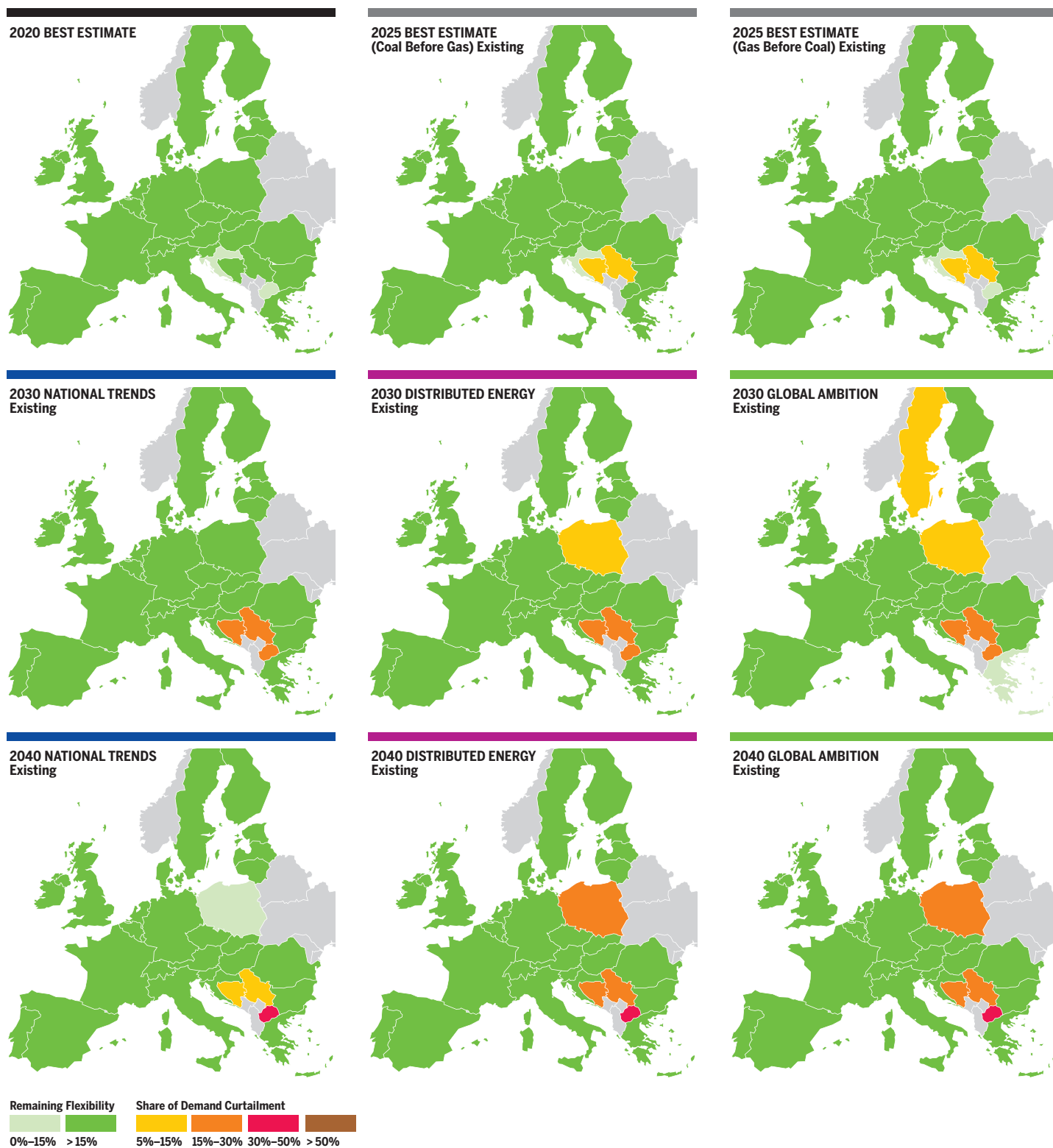
Figure 3.20 Existing infrastructure level: Climatic Stress under 2-week cold spell situation.
