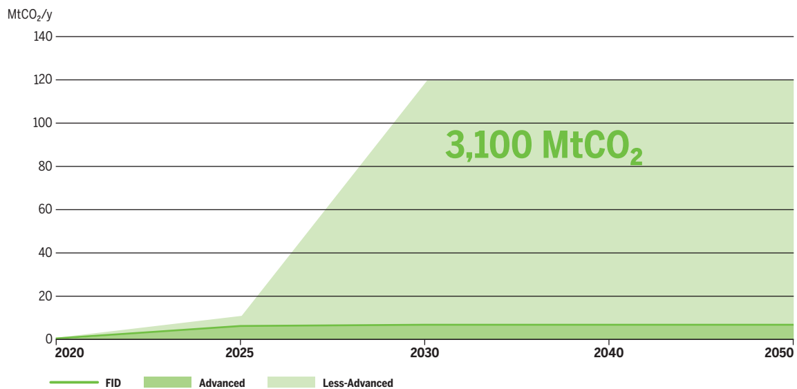
Figure 2.9 CO 2 savings generated by ETR projects in TYNDP 2020
