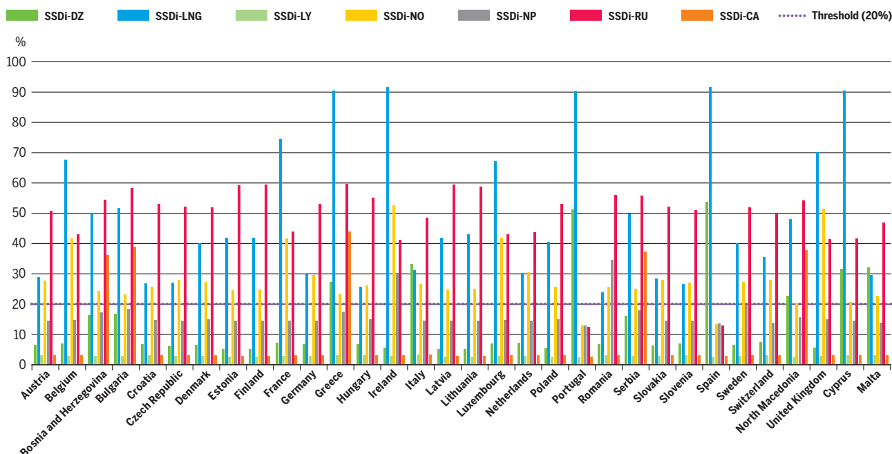
Figure 4.73 SSDi – PCI infrastructure level – National Trends 2030
