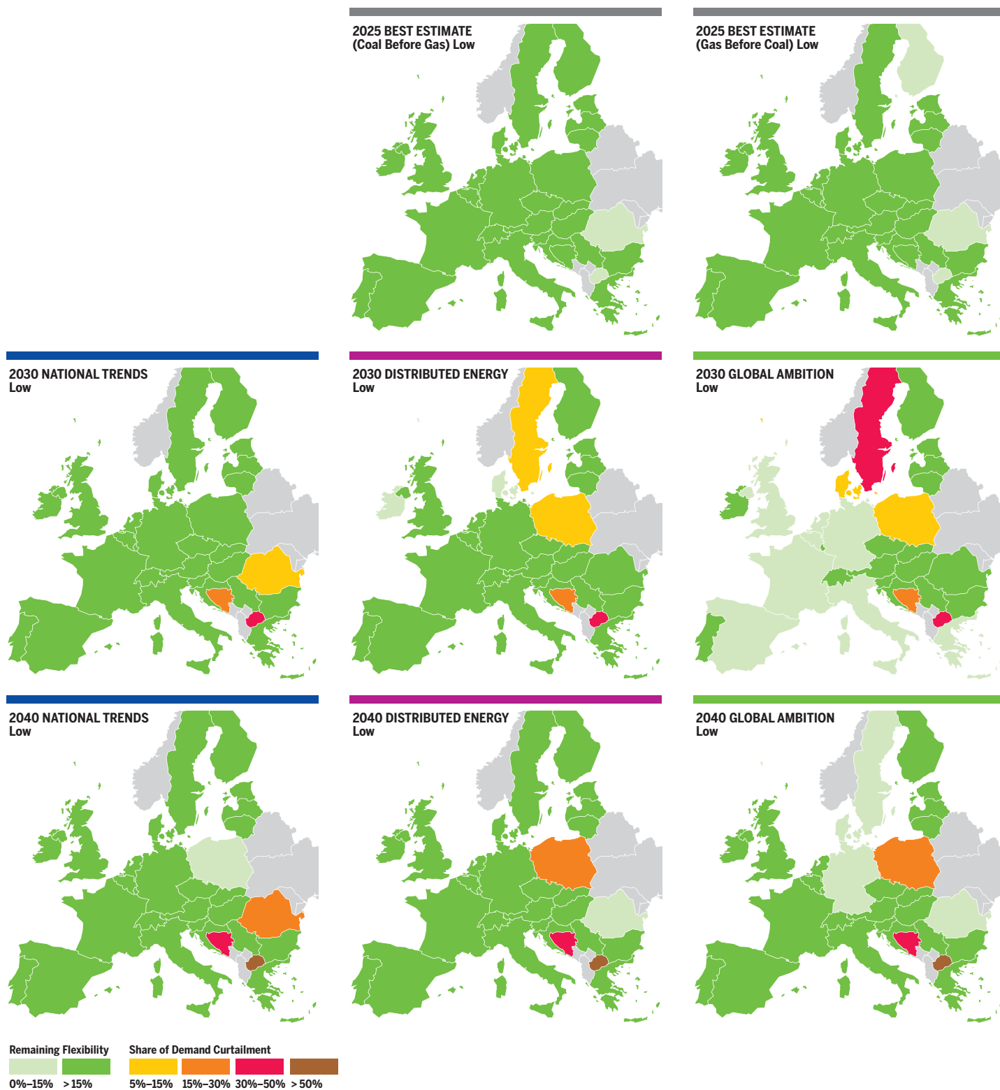
Figure 3.42 Low infrastructure level: Ukraine transit disruption under peak day situation.
