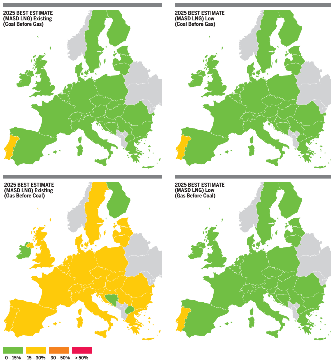
Figure 4.8 MASD LNG – Gas Before Coal and Coal Before Gas – 2025 – Existing and Low Infrastructure levels
