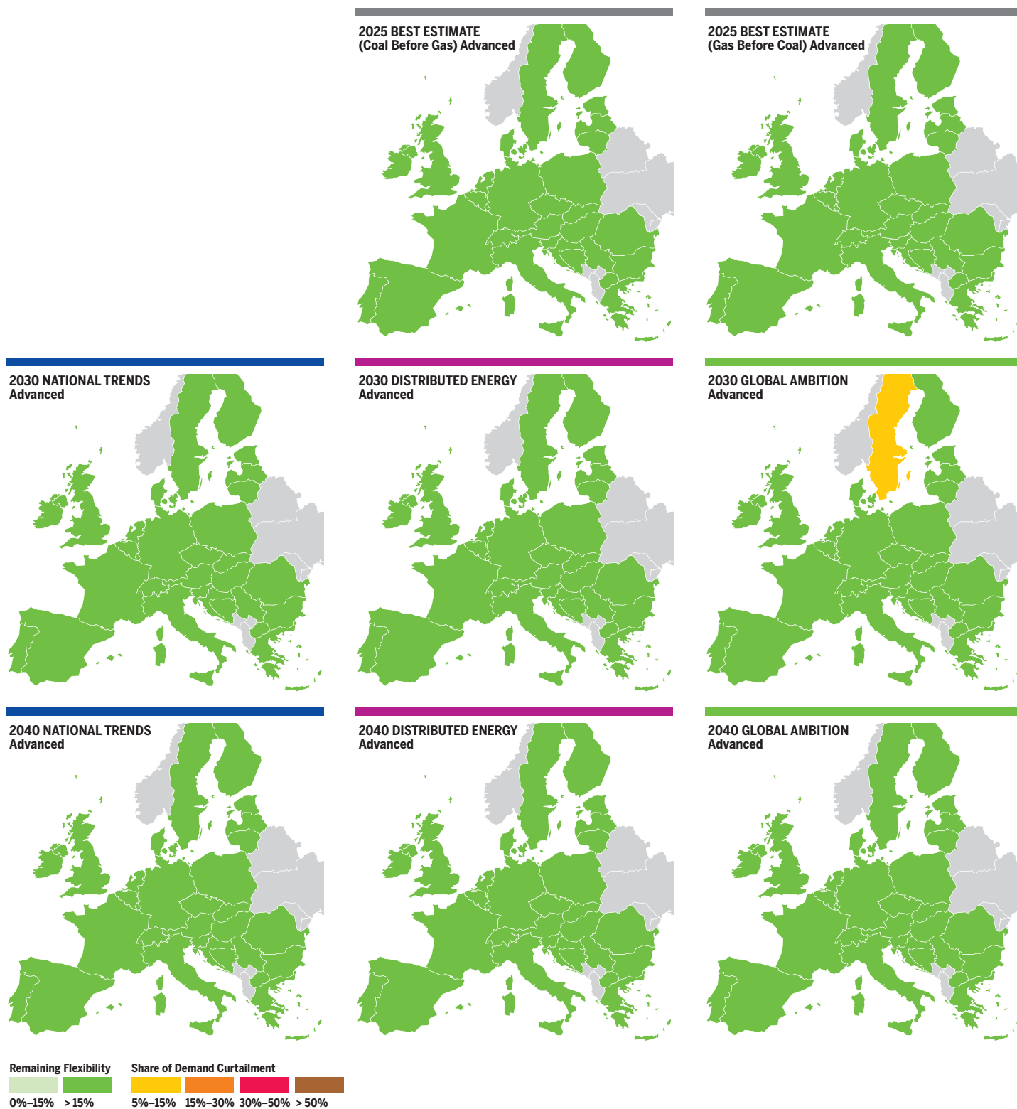
Figure 3.50 Advanced infrastructure level: Ukraine transit disruption under 2-week cold spell situation.
