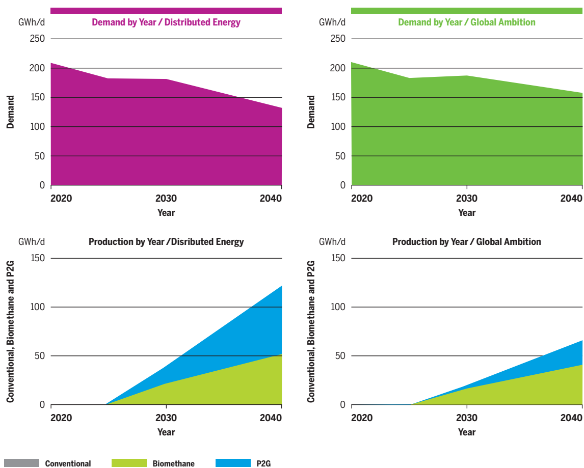
Figure 3.84 2-week cold spell demand and production in Finland in COP 21 scenarios in GWh/d.
