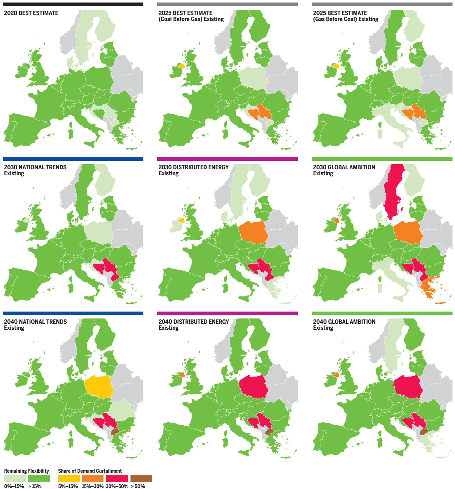
Figure 3.8 Existing infrastructure level: Climatic Stress under a peak day situation.
