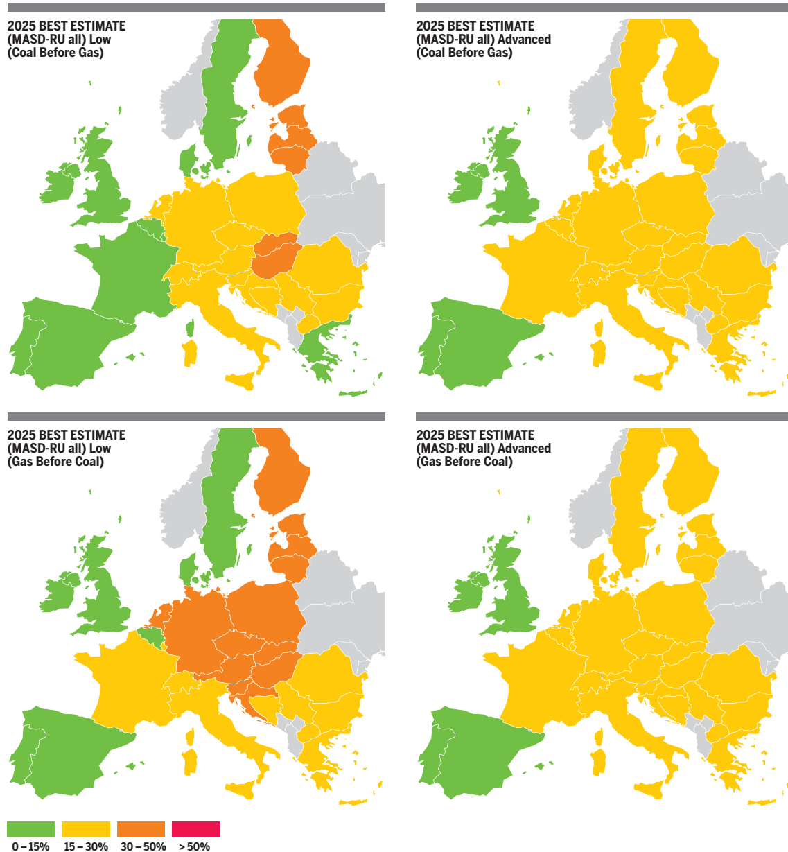
Figure 4.27 MASD RUSSIA – Gas Before Coal and Coal Before Gas – 2025 – Low and Advanced infrastructure levels.
