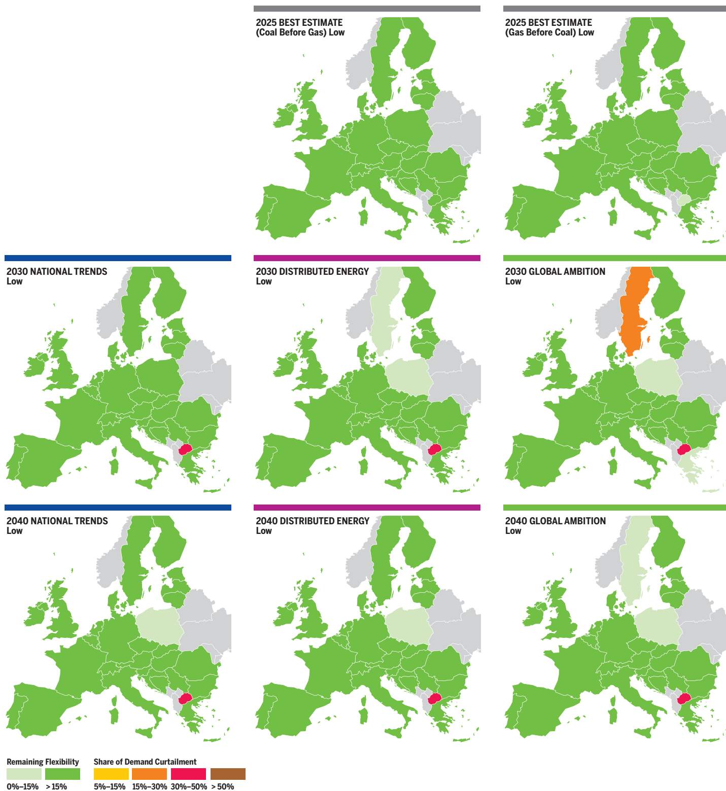
Figure 3.34 Low infrastructure level: Climatic Stress under 2-week Dunkelflaute situation.
