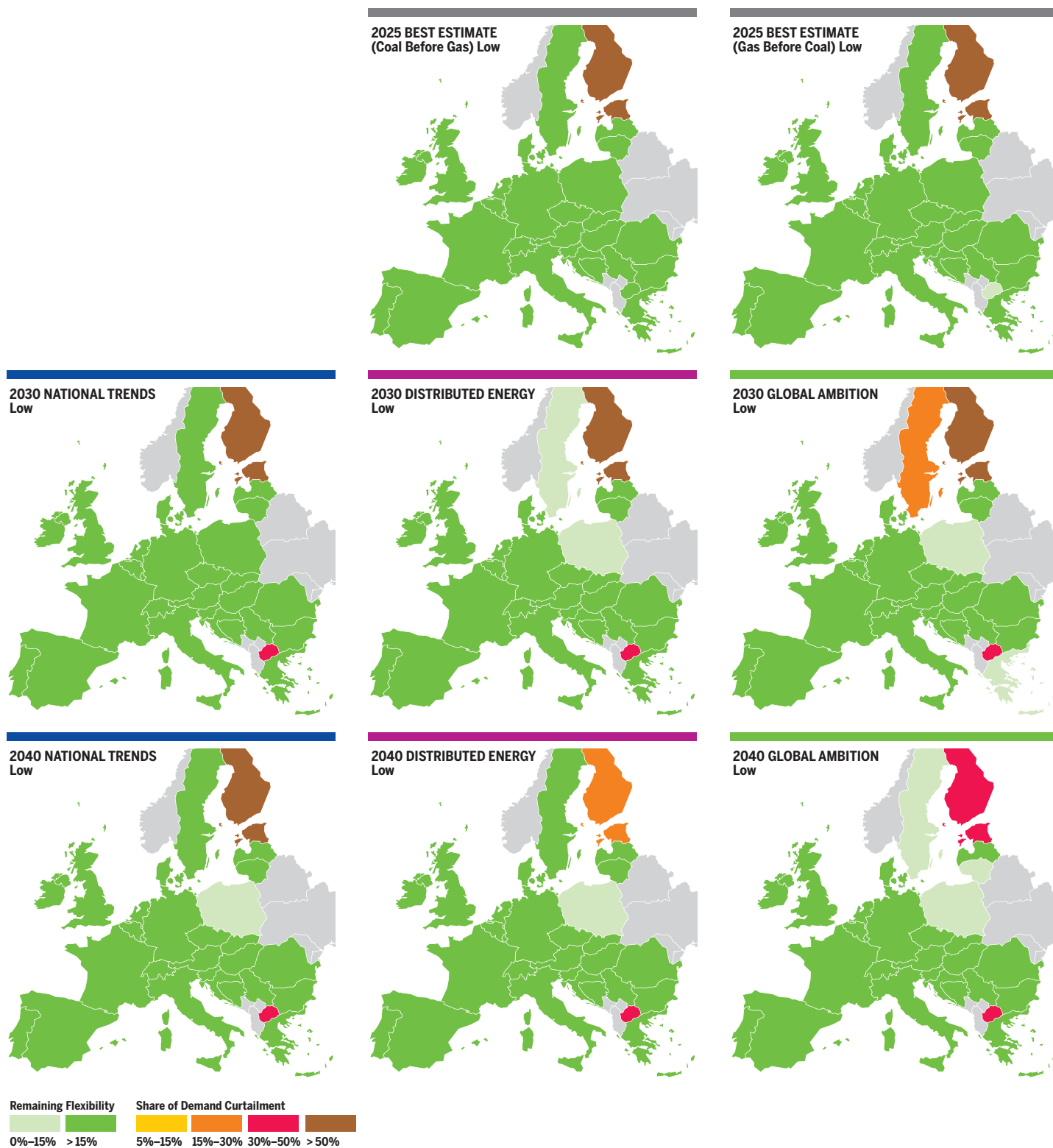
Figure 3.91 Low infrastructure level: Baltics States and Finland transit disruption under 2-week Dunkelflaute situation.
