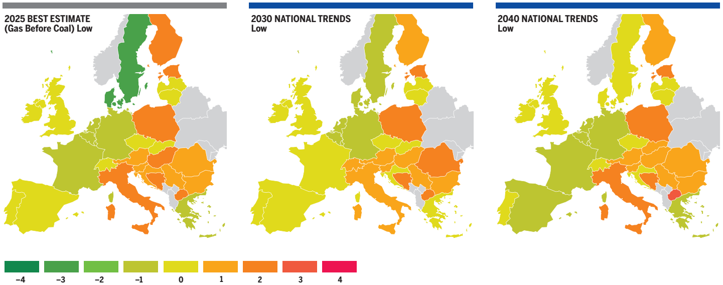
Figure 4.91 MP delta (EUR/MWh) – Low infrastructure level, South Max supply configuration
