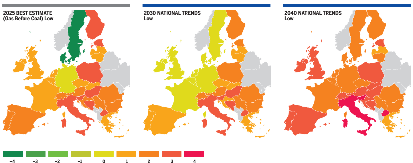
Figure 4.88 MP delta (EUR/MWh) – Low infrastructure level, LNG Min supply configuration
