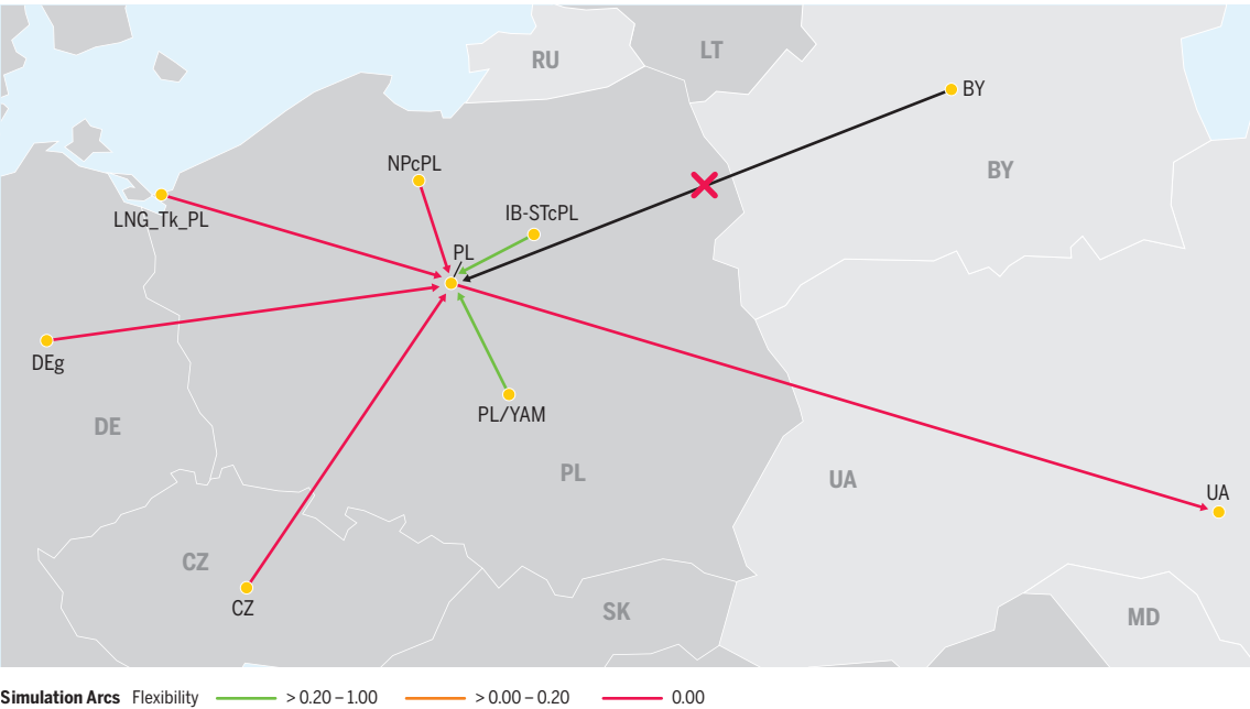
Figure 3.67 Infrastructure limitations towards Poland under Belarus disruption, Existing infrastructure, Gas Before Coal, 2025.
