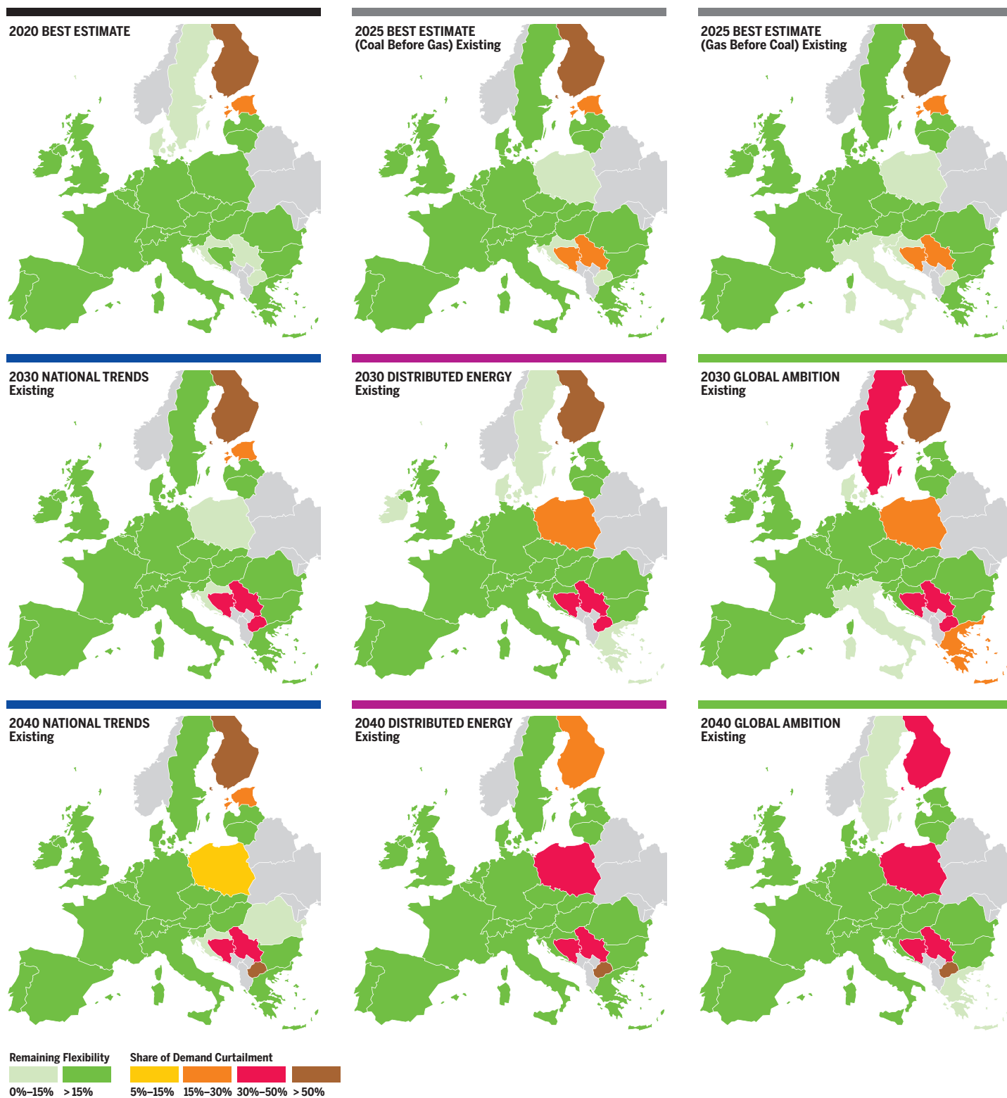
Figure 3.80 Existing infrastructure level: Baltics States and Finland transit disruption under peak day situation.
