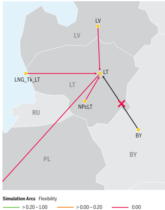
Figure 3.63 Infrastructure limitations towards Lithuania under Belarus transit disruption, Low infrastructure, Global Ambition, 2040.
