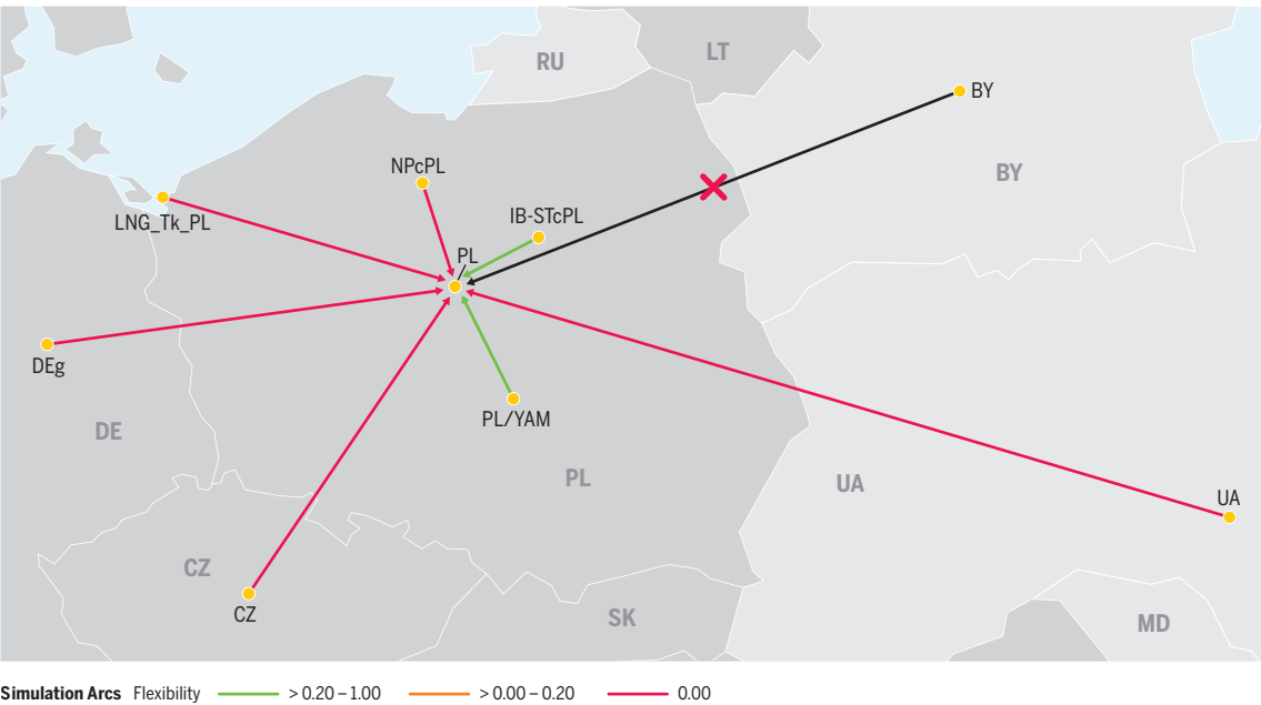
Figure 3.72 Infrastructure limitations towards Poland under Belarus transit disruption, Existing infrastructure, 2025.
