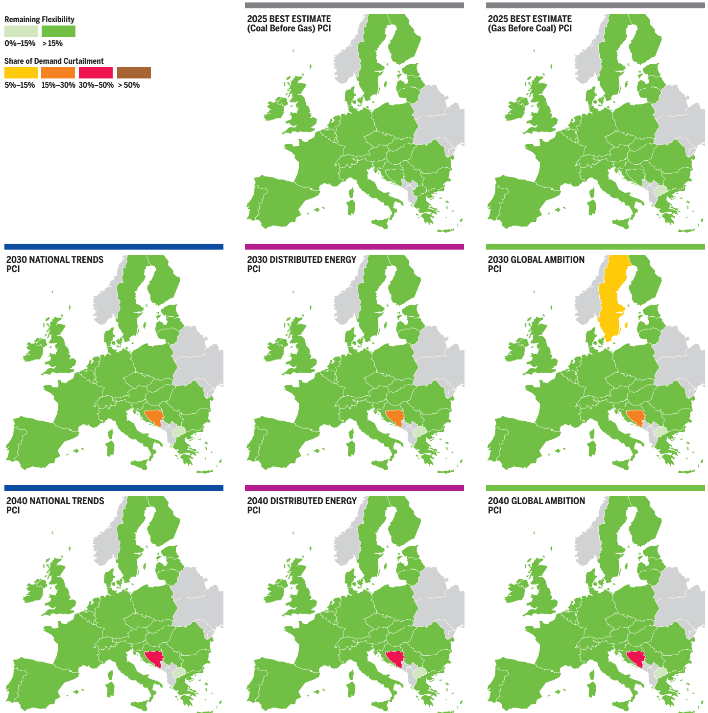
Figure 3.102 PCI infrastructure level: Algerian pipeline import route disruption under 2-week cold spell situation.
