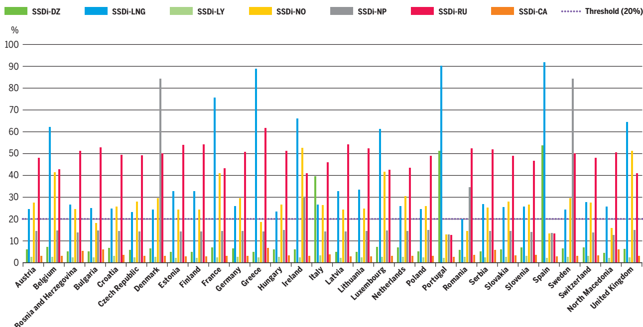
Figure 4.55 SSDi – Low infrastructure level – National Trends 2030
