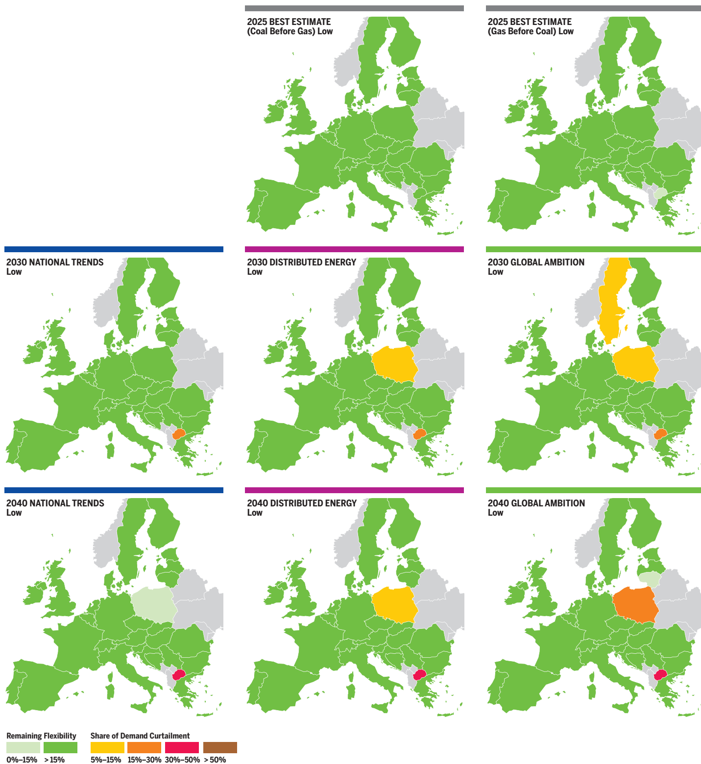
Figure 3.69 Low infrastructure level: Belarus transit disruption under 2-week cold spell situation.
