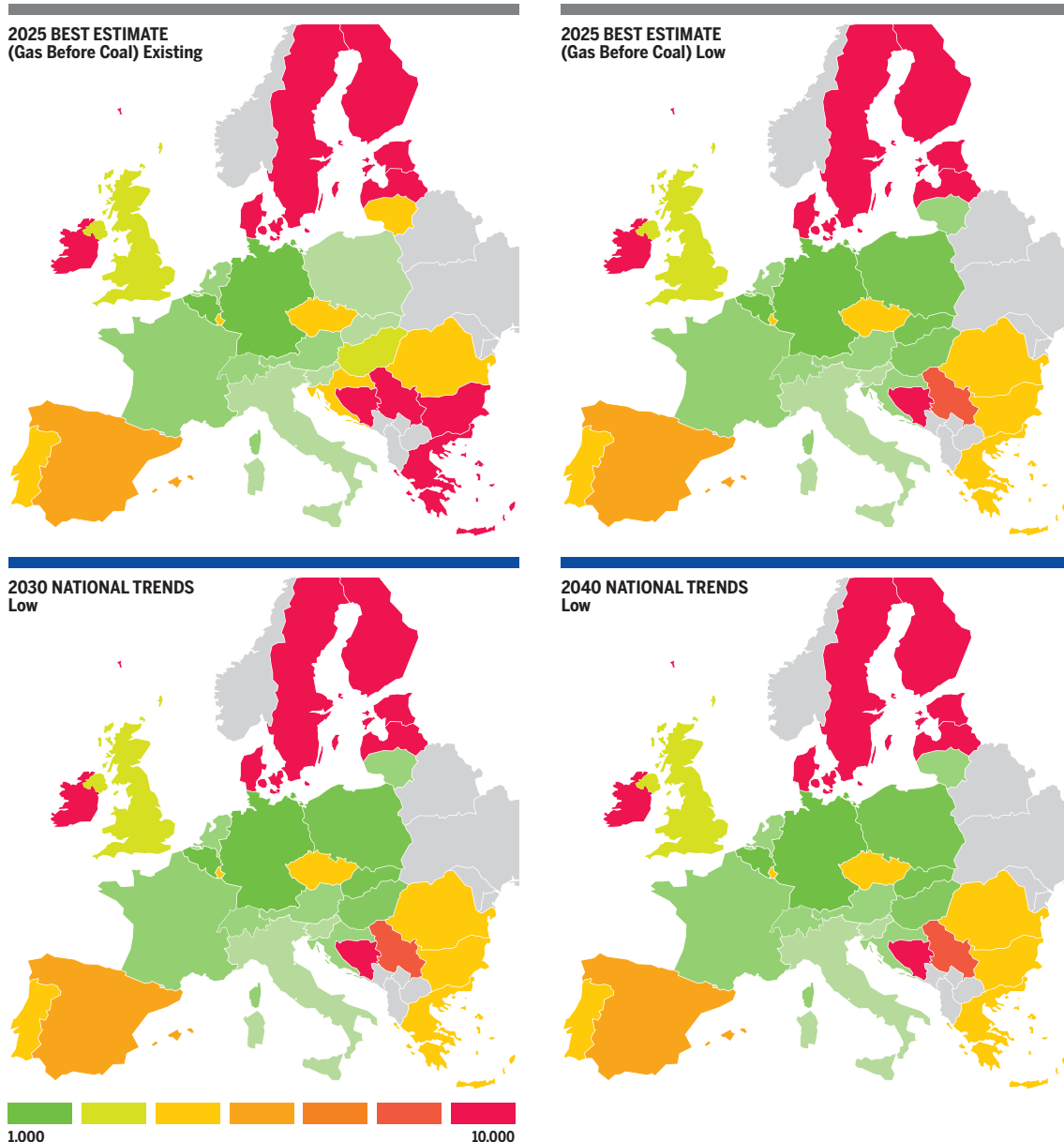
Figure 4.35 LNG and Interconnection Capacity Diversification – Existing and Low infrastructure levels.
