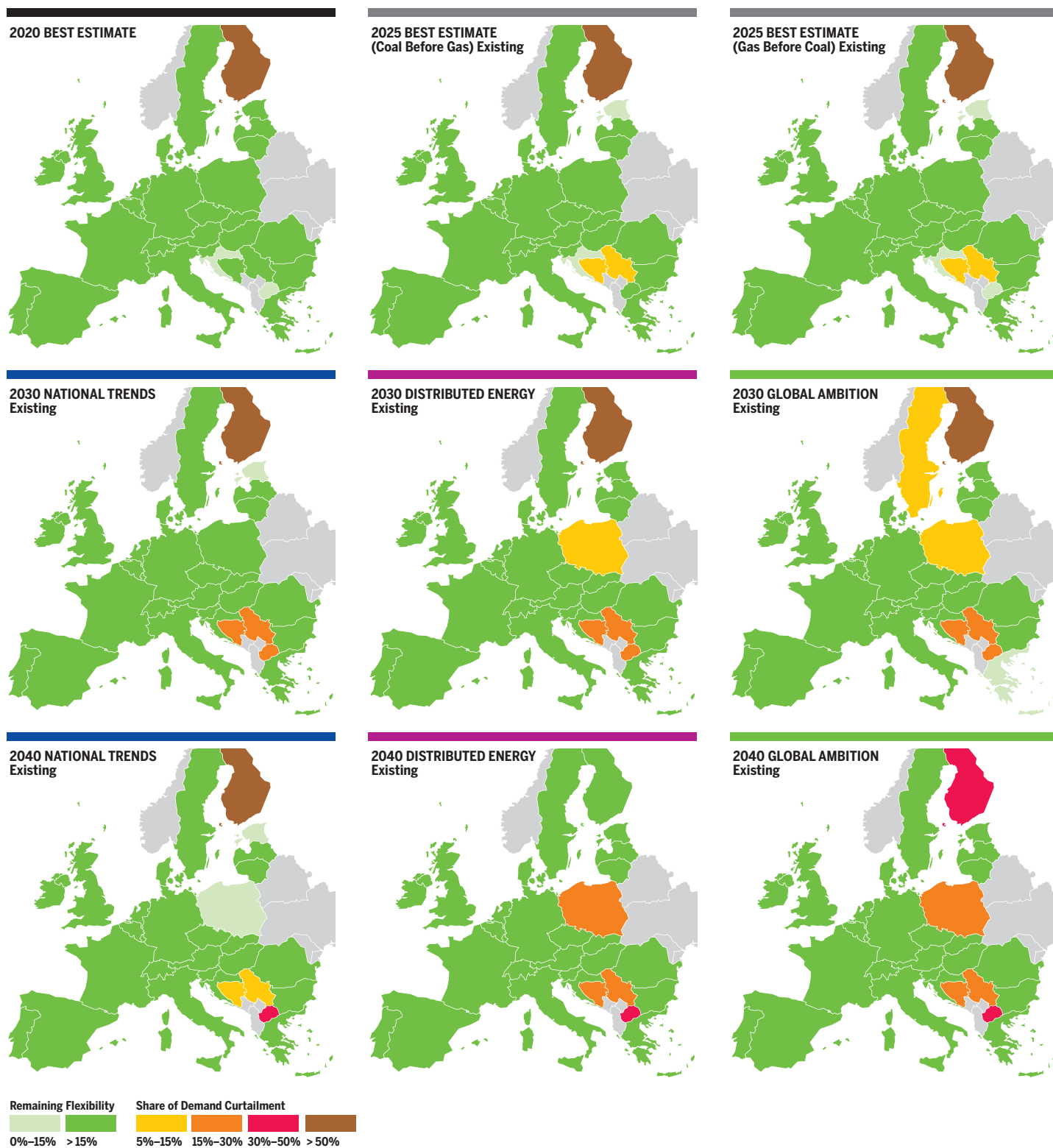
Figure 3.85 Existing infrastructure level: Baltics States and Finland transit disruption under 2-week cold sell situation.
