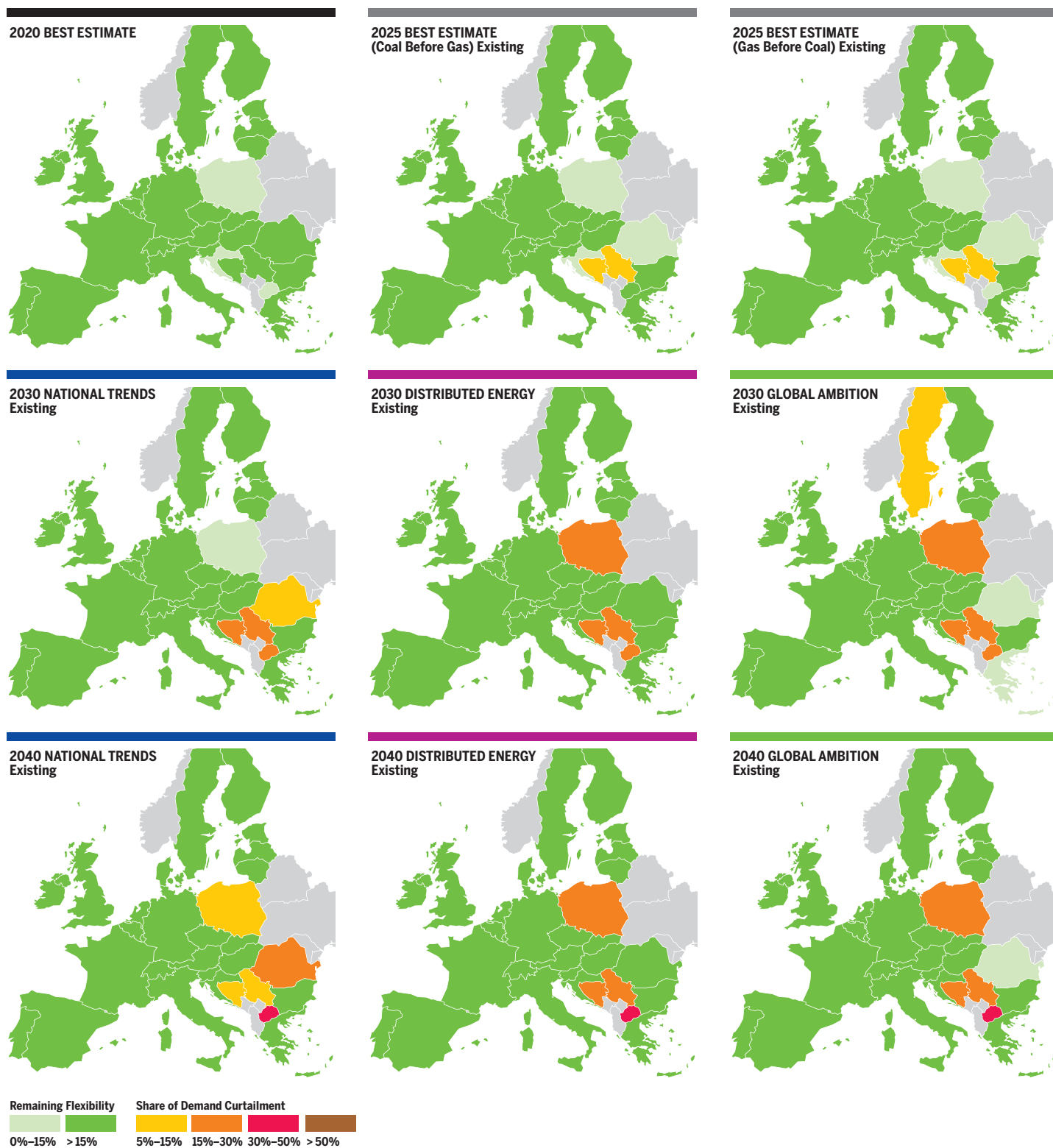
Figure 3.48 Existing infrastructure level: Ukraine transit disruption under 2-week cold spell situation.
