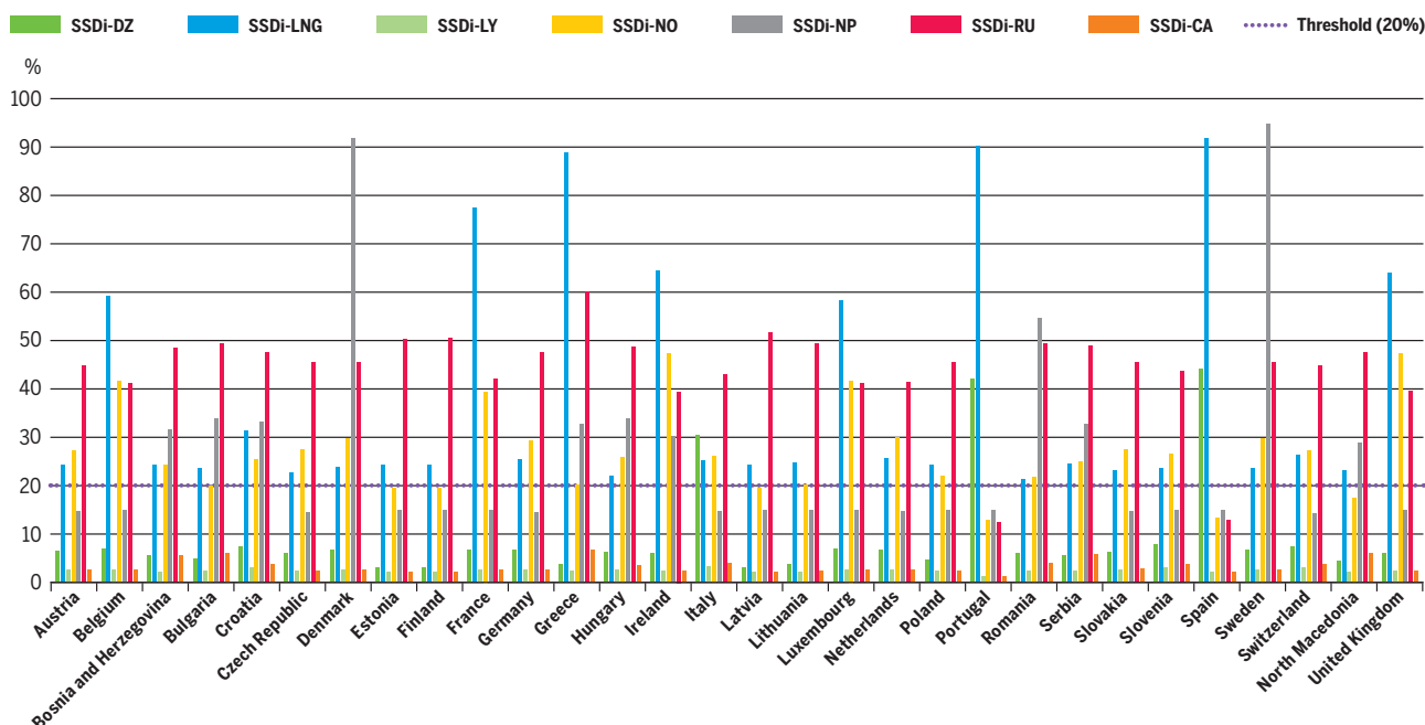
Figure 4.57 SSDi – Low infrastructure level – Distributed Energy 2030
