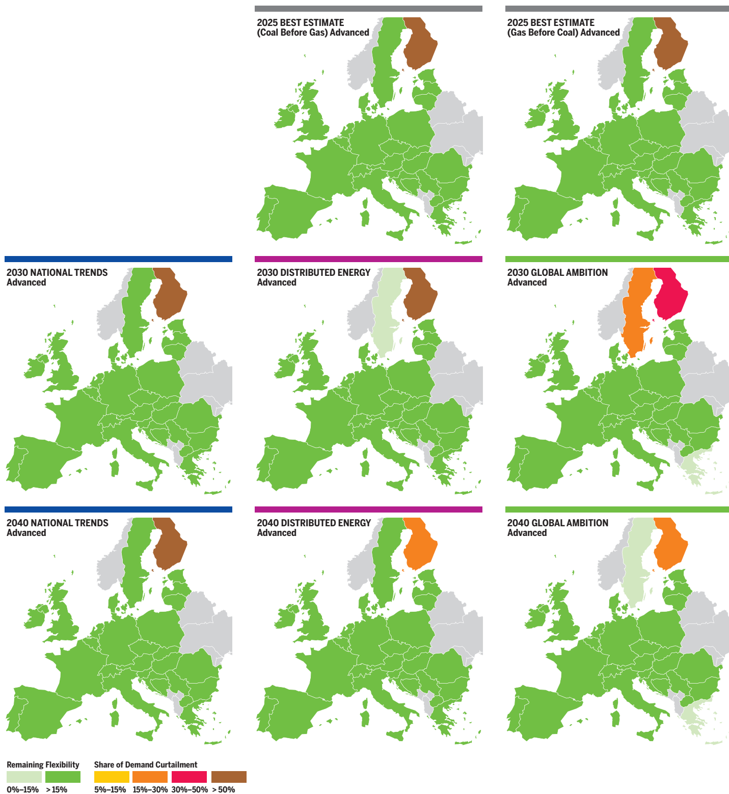
Figure 3.92 Advanced infrastructure level: Baltics States and Finland transit disruption under 2-week Dunkelflaute situation.
