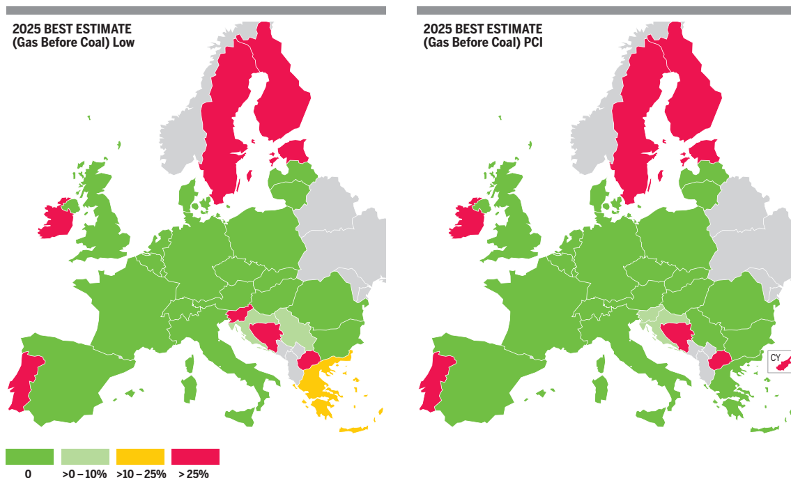
Figure 3.125 Maximum exposure to demand curtailment in case of SLID in Low and PCI infrastructure levels in 2025 for Gas Before Coal scenario.
