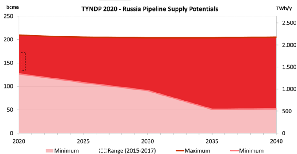
FIGURE 39: RUSSIA PIPELINE SUPPLY POTENTIAL FOR EU
