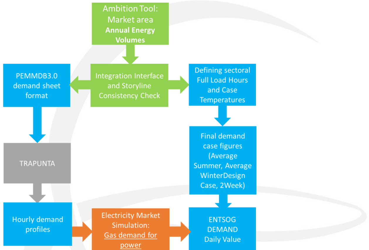
FIGURE 15: DEMAND PROFILE BUILDING PROCESS STEPS
