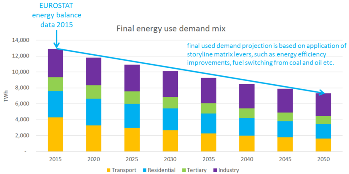
FIGURE 13: FINAL USE DEMAND COMPOSITION AND DEVELOPMENT
