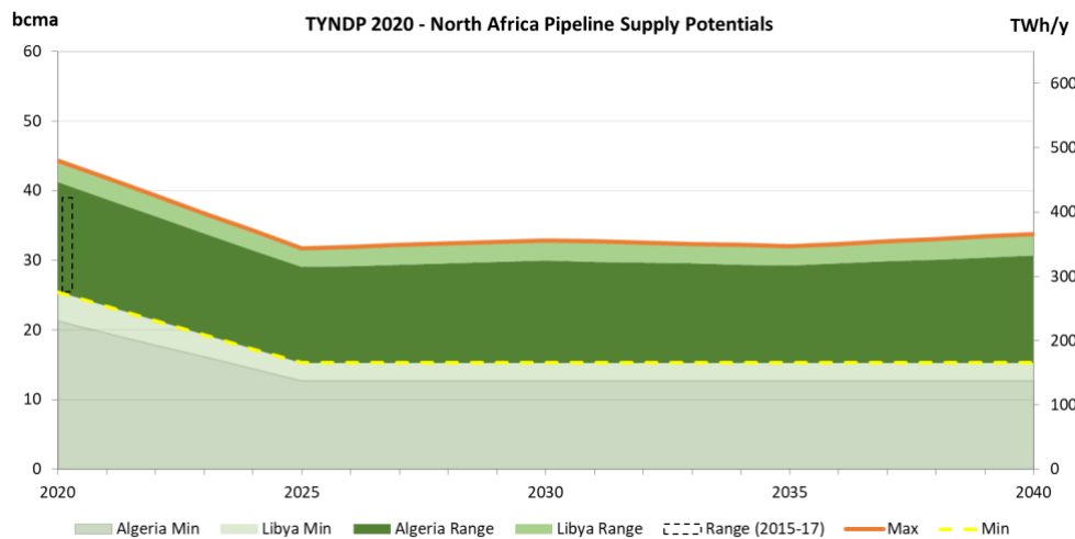
FIGURE 41: NORTH AFRICA PIPELINE SUPPLY POTENTIAL FOR EU
