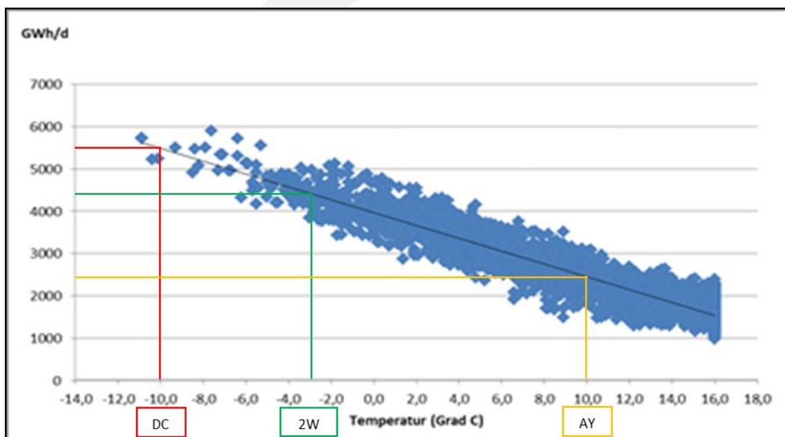
FIGURE 26: TEMPERATURE VS DEMAND INTERPOLATION
