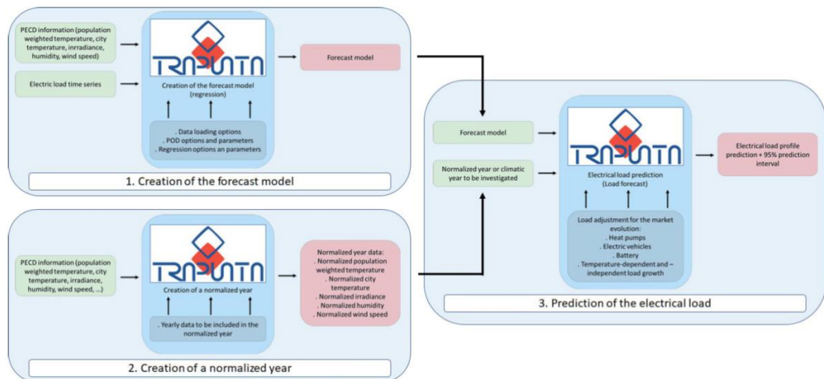
FIGURE 20: THREE PROCESS STEPS IN TRAPUNTA
