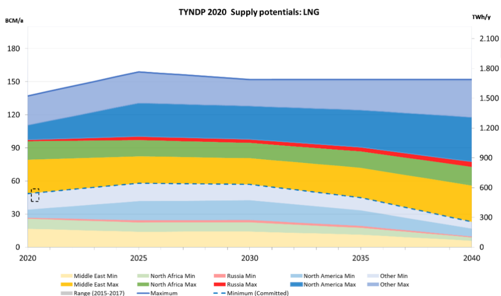
FIGURE 43: LNG SUPPLY POTENTIAL FOR EU
