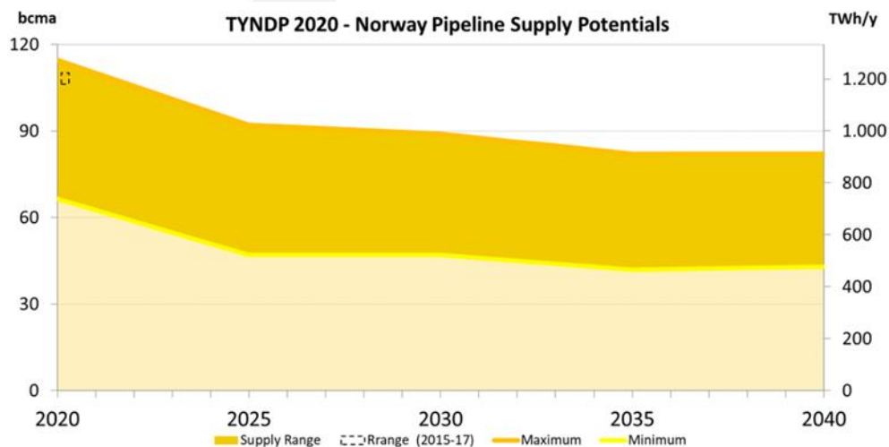
FIGURE 40: NORWEGIAN PIPELINE SUPPLY POTENTIAL FOR EU
