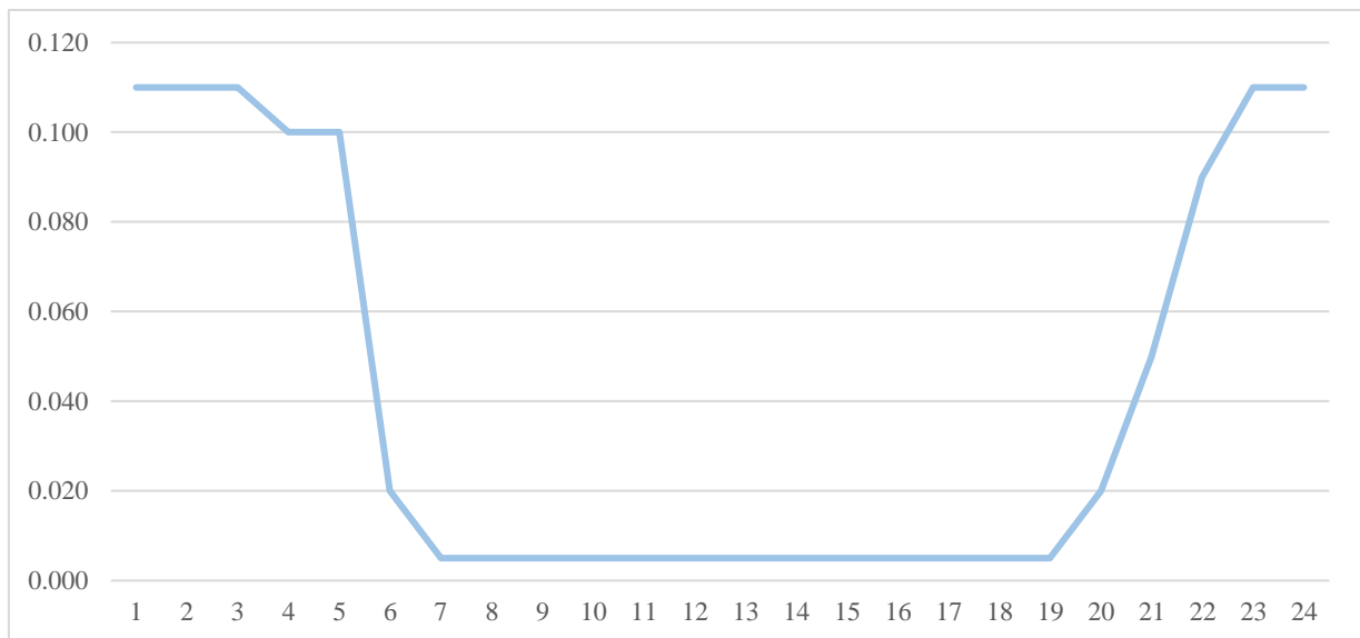
FIGURE 24: HEAVY GOODS CHARGING PROFILE
