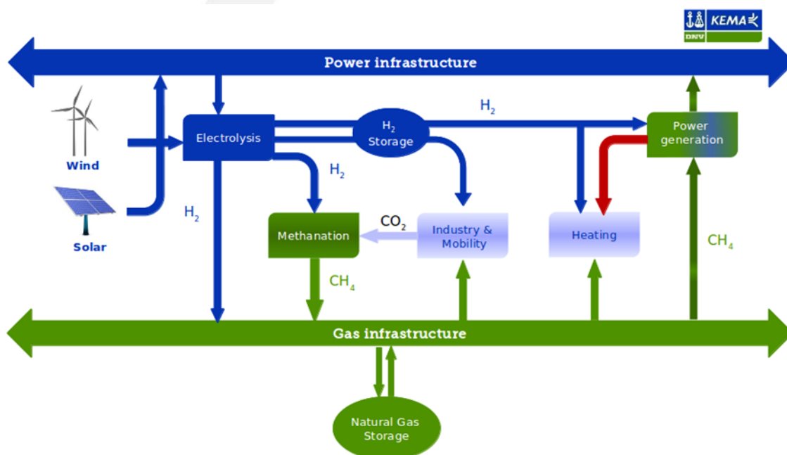
FIGURE 44: P2G PROCESS CHAIN
