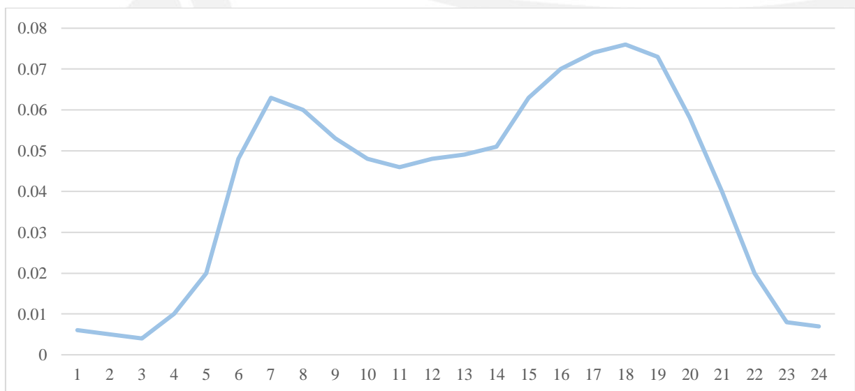
FIGURE 23: PASSENGER TRAINS LOAD PATTERN
