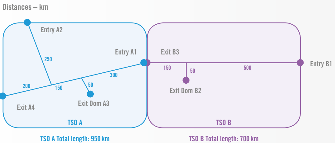
Figure 66: Distance map before the merger
