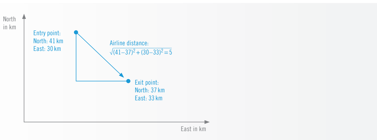
Figure 17: Simple example of airline distance calculation
